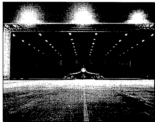
Figure 7-3 B-1 Bomber in Large Anechoic Chamber for Installed Systems Testing
