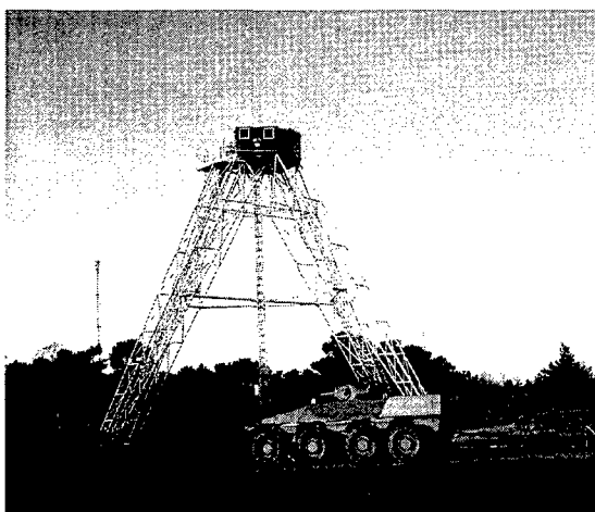
Figure 7-1 STRADI Radar Static Signature Evaluation Facility at CELAR Facility in France
