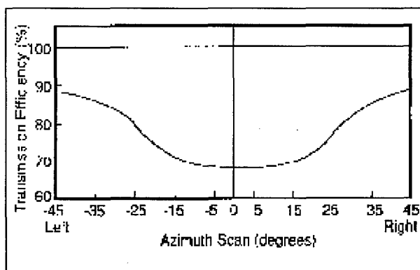
Figure 9-2 Transmission Efficiency
