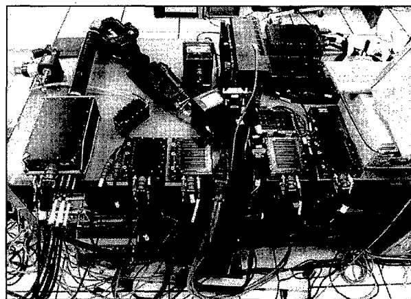
Figure 5-1 Federated System in HITL Test at ECSEL Facility, Pt. Mugu, California
