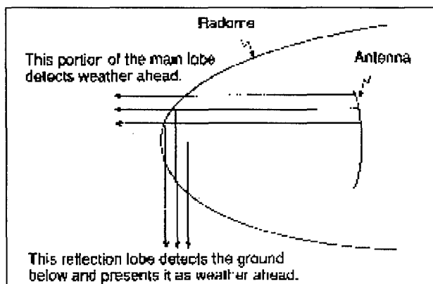
Figure 9-1 Radome Ground Return
