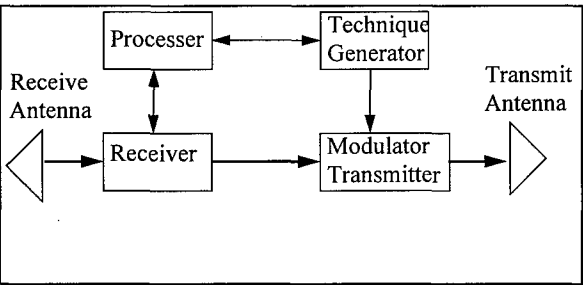
Figure 3-1 Simplified Jammer Block Diagram
