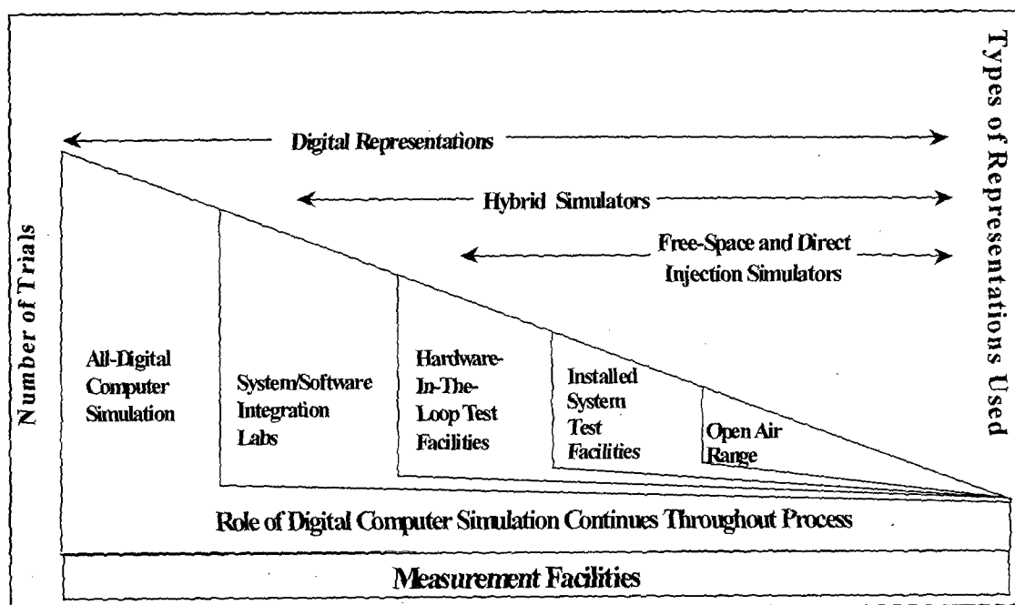
Figure 6-1 Activities Within the Digital M&amp;S Interface
