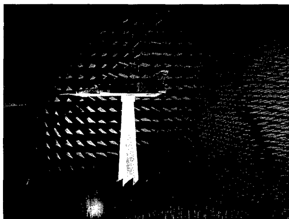
Figure 7-4 CHEOPS Anechoic Facility, France
