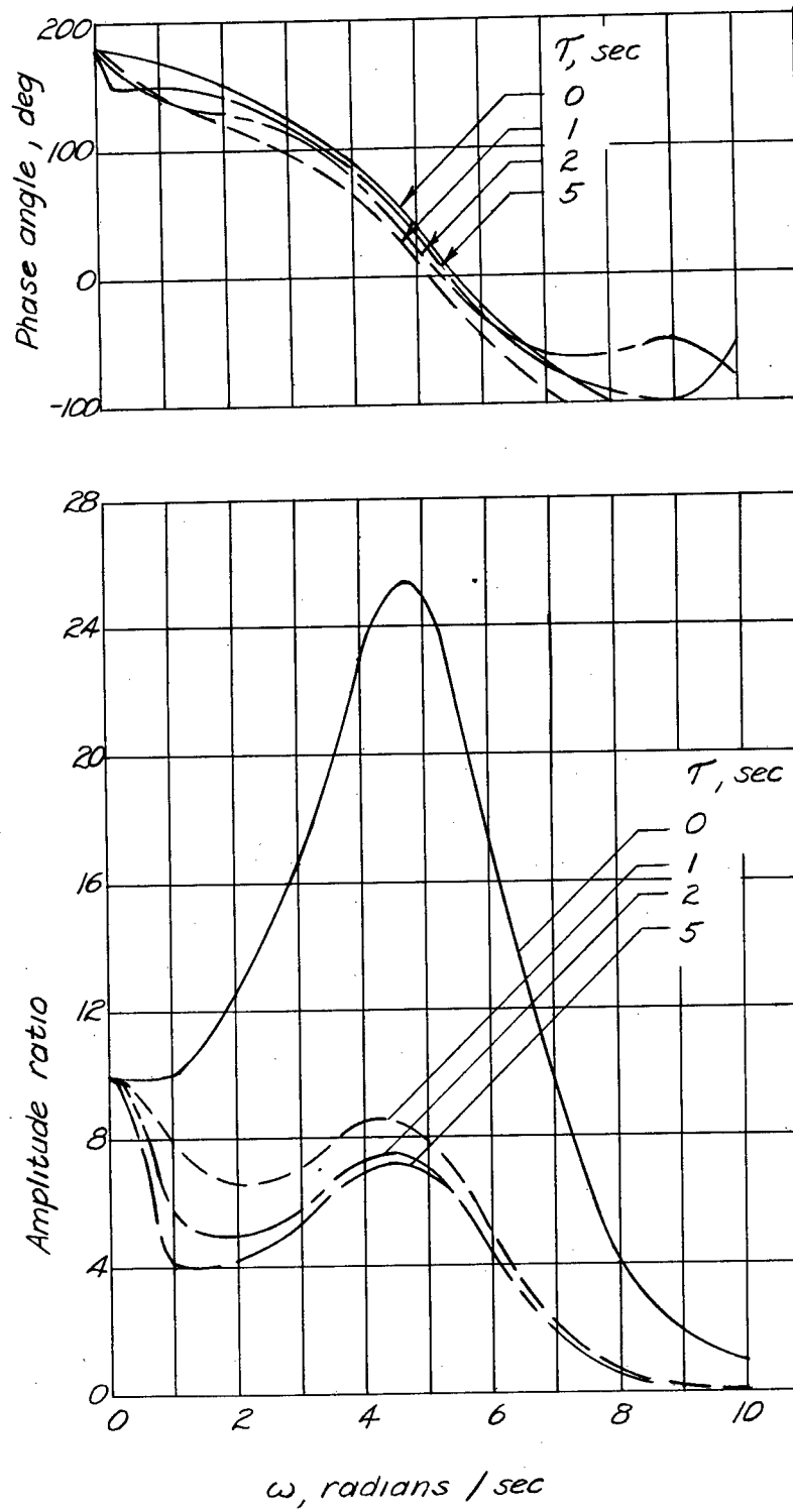
(c) Response of roll angle \phi to side gusts \beta_g .
