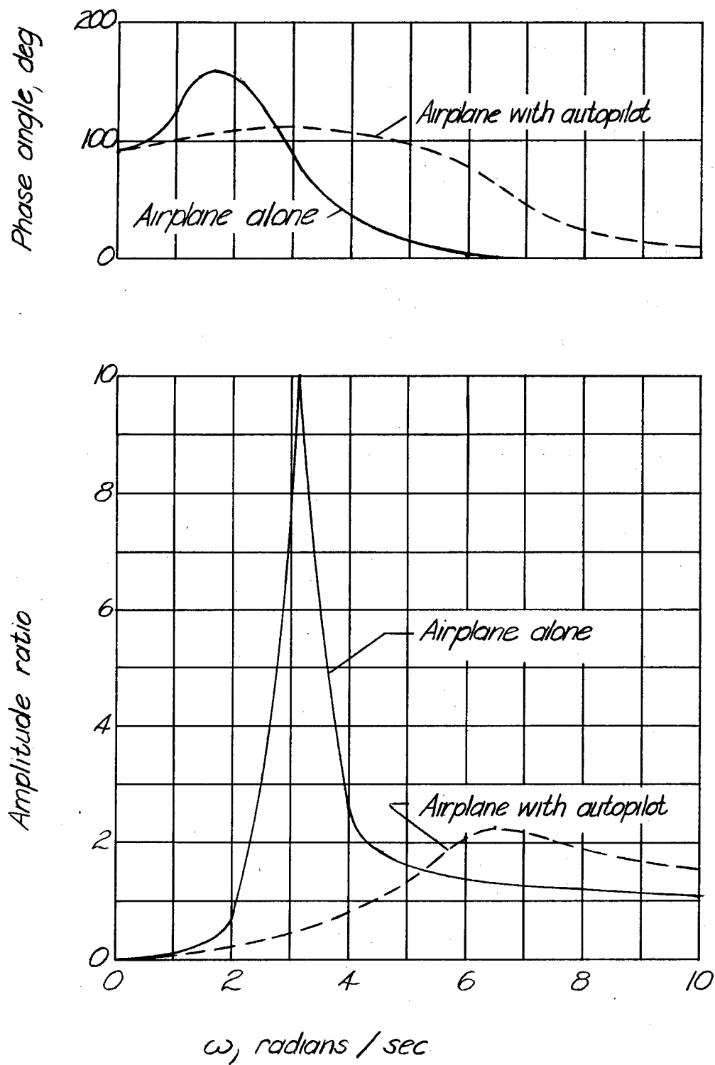
(b) Response of sideslip \beta to side gusts \beta_g .
