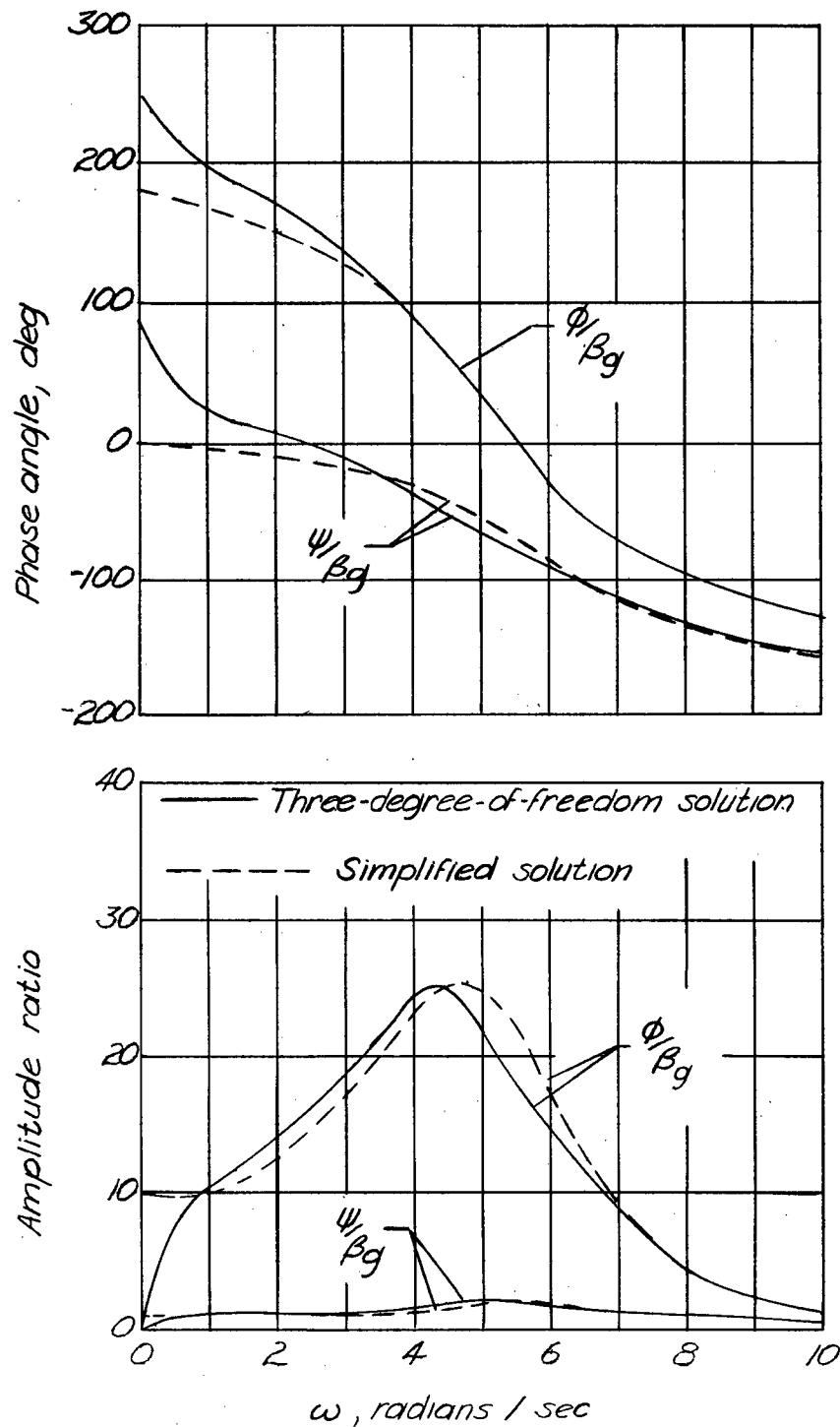
Figure 2.- Frequency response of the airplane in combination with the basic autopilot. The comparison is shown between the results obtained by using a three-degree-of-freedom analysis and the simplified analysis used in this paper.
