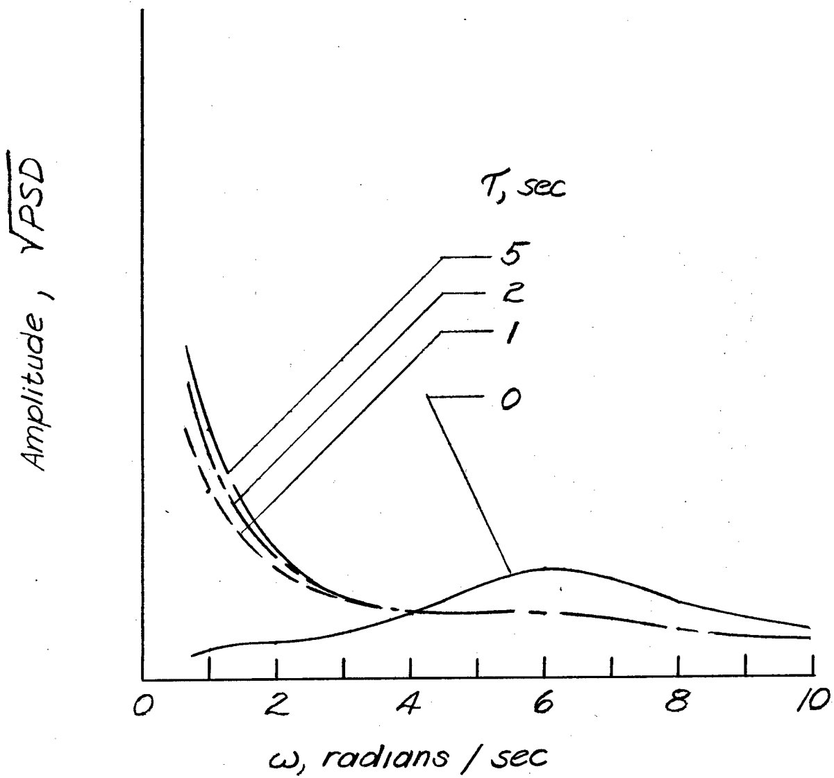
(b) Amplitude variation of sideslip angle \beta with frequency.
