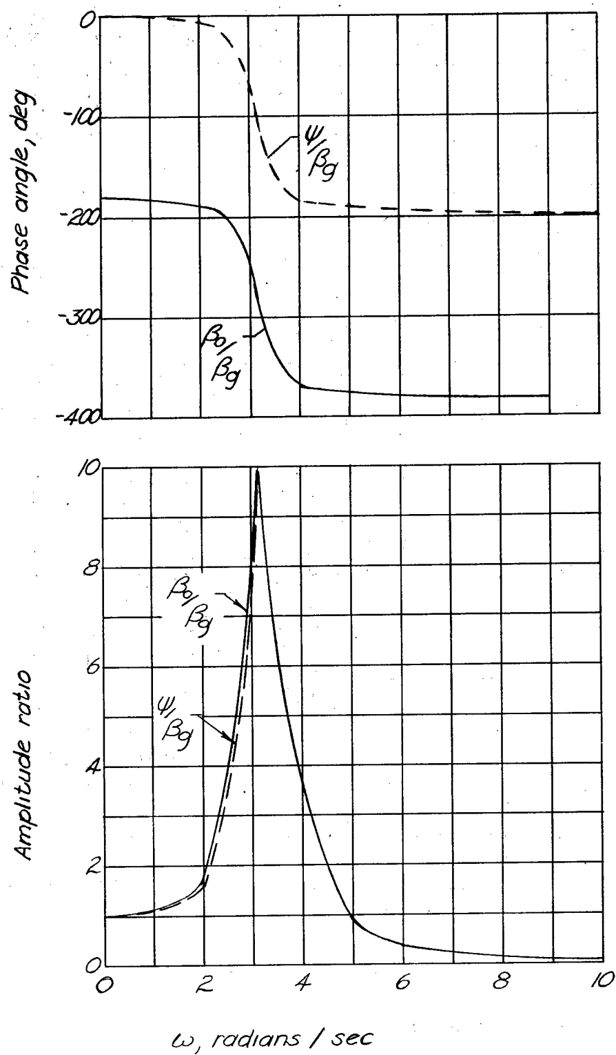
(c) Frequency responses of airplane to side gusts.
