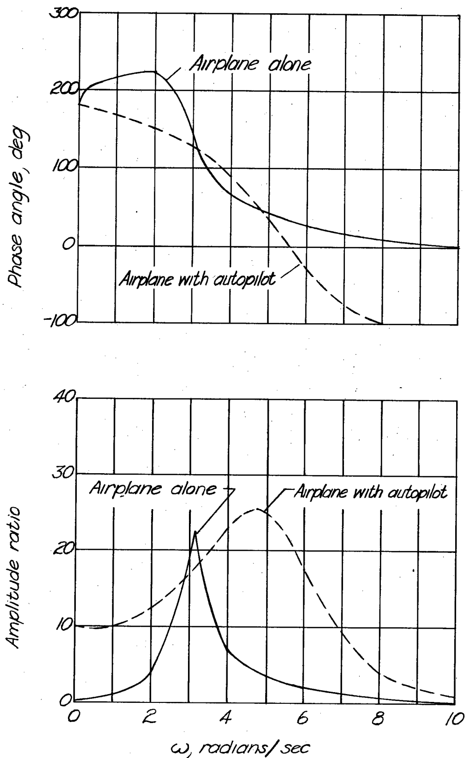
(c) Response of roll angle \phi to side gusts \beta_g .
