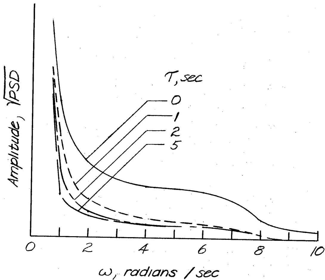
(a) Amplitude variation of yaw angle \psi with frequency.
