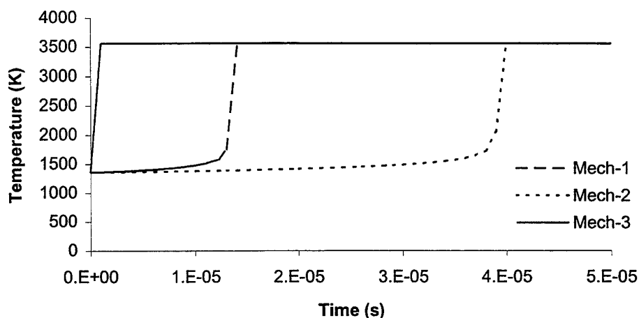
Figure 25: Temperature profiles against time for various kinetics mechanisms for a stoichiometric MT composition. References: Mech-1[19], Mech-2[20], Mech-3[21].
