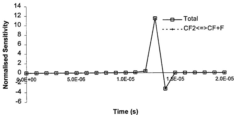
Figure 20: Normalised sensitivity for CF radicals for a stoichiometric MT mixture.
