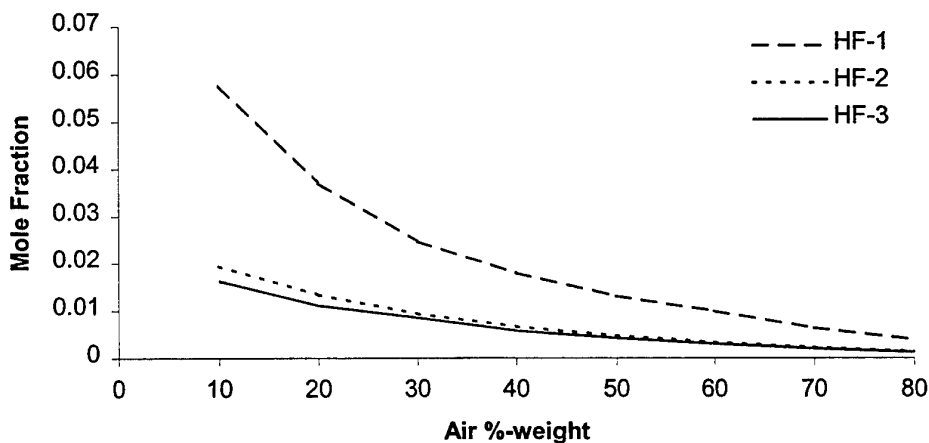
Figure 15: Concentration profiles of HF from various MTV-air reactions. (numerals HF-1 etc. refers to the MTV-1 formulation etc, respectively).
