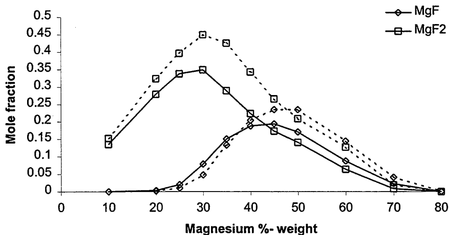
Figure 9: Comparison of MgF and MgF 2 profiles: --- MT, — MTV (16% Viton).
