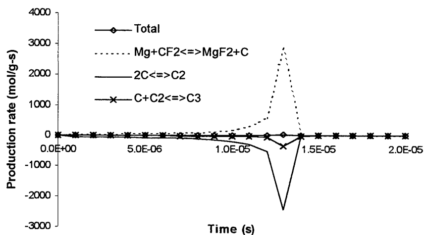
Figure 22: Production rate for Carbon via three main reaction (stoichiometric MT composition).
