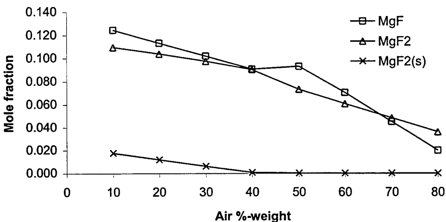
Figure 11: Magnesium fluorides concentration from combustion of MTV-air composition (MTV-1 mixture in Table 1).
