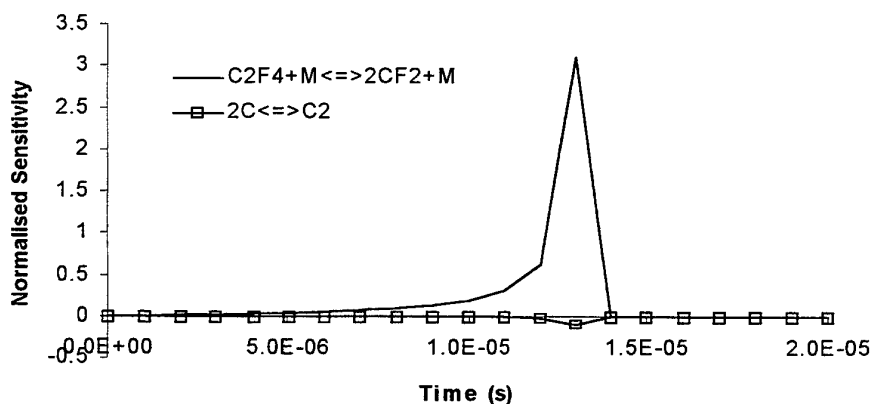
Figure 23: Normalised sensitivity for temperature with respect to important reaction rates (a stoichiometric MT composition).
