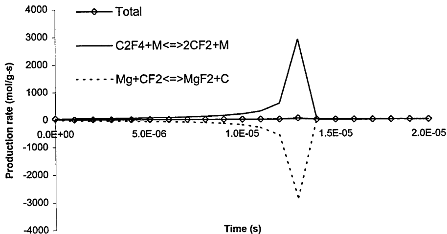
Figure 21 : Rate of production for CF2 via two major reactions (Mixture: stoichiometric MT composition).
