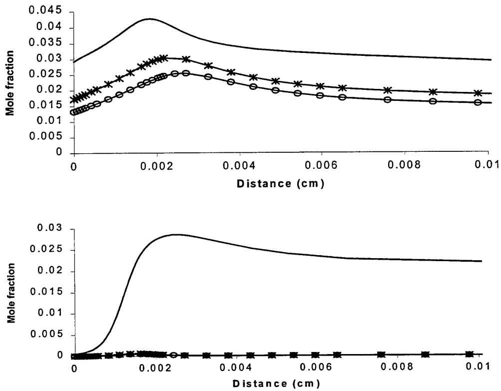
Figure 33: Profiles of CF (top) and CF2 (bottom) species against distance from burner's exit plane. Mixtures: ___stoichiometric, -* UK Flare, -o- US igniter..
