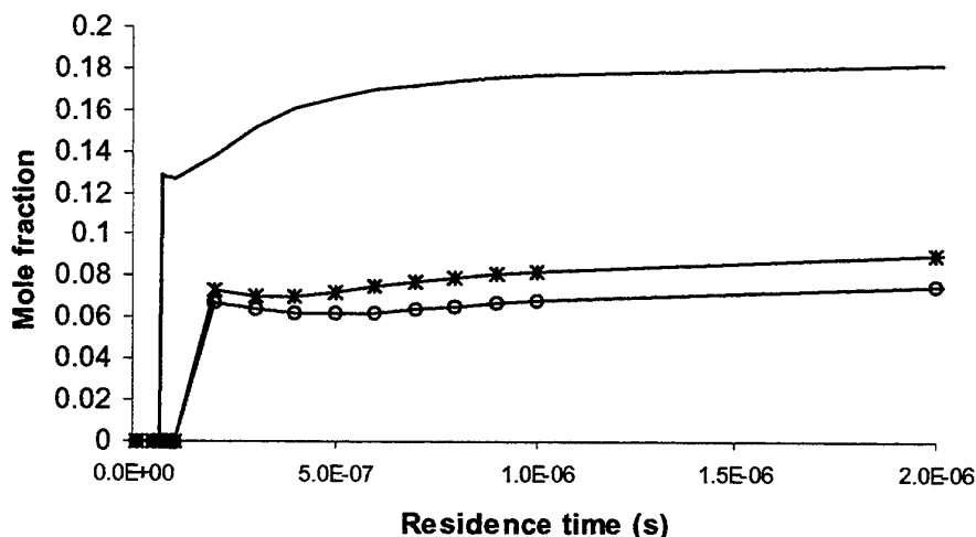
Figure 31: Total Carbon ( C , C_2 , C_3 , etc.) against residence time. MT compositions: — stoichiometric, —* UK Flare, —o US igniter.
