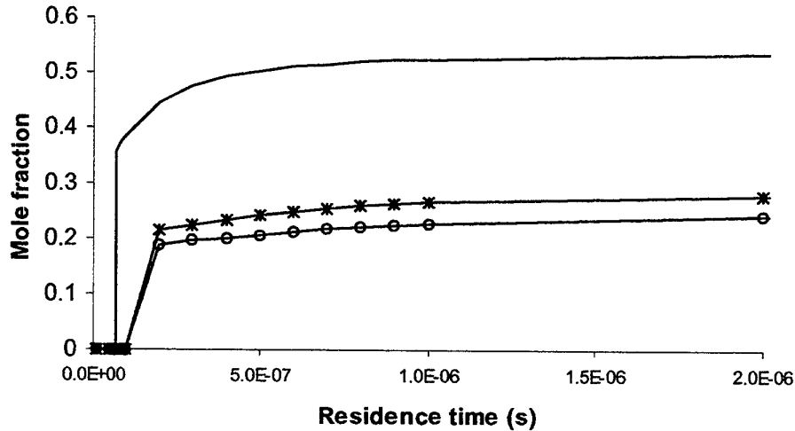
Figure 28: Distribution of \text{MgF}_2 against residence time. MT compositions: ___stoichiometric, - * UK Flare, -o- US igniter.
