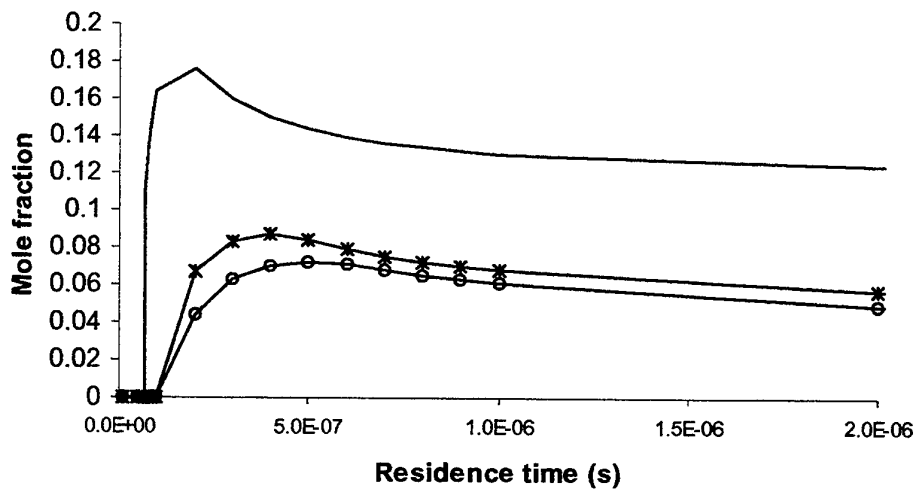
Figure 29: Profiles of \text{CF} against residence time. MT compositions: ___stoichiometric, - * UK Flare, -o- US igniter.
