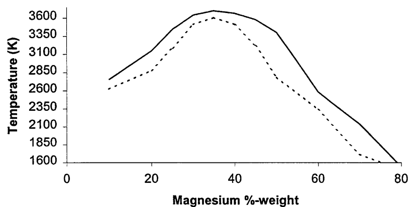
Figure 2: Effect of inlet temperature and phase state on the adiabatic flame temperature of MT composition (Species in liquid and solid phases are included). Legend as in Figure 1.
