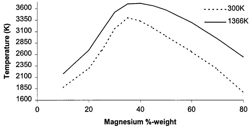
Figure 1: Effect of inlet temperature and phase state on the adiabatic flame temperature of MT composition (all species are in gaseous phase).
