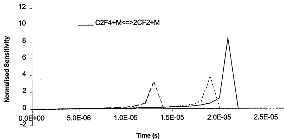
Figure 24: Normalised sensitivity for temperature with respect to a main reaction: ..... Stoichiometric mixture 33:67, ____ Flare composition 55:45, - - - Igniter composition 61:39.
