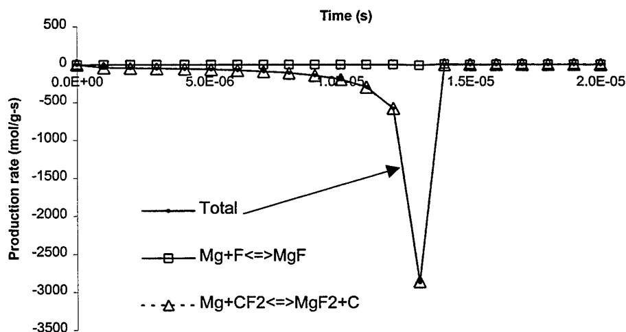
Figure 19: Production rate for Mg with respect to important reactions.
