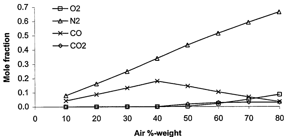
Figure 12: CO, O 2 , CO 2 and N 2 profiles of MTV-air combustion.
