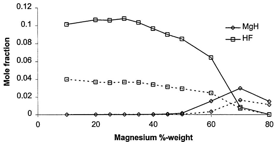
Figure 8: Concentration of MgH and HF for MTV mixtures: — 16% Viton, --- 5% Viton. (inlet temperature 1366K).
