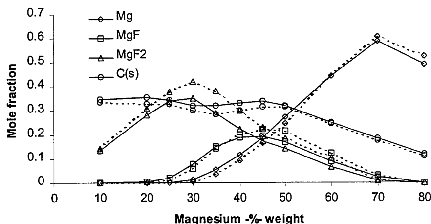
Figure 7: Products concentration of MTV mixtures: — 16% Viton, - - - 5% Viton. (inlet temperature 1366K).
