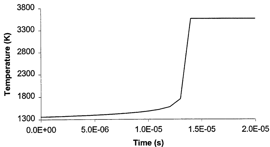
Figure 17 : Time evolution of flame temperature for a stoichiometric MT composition.
