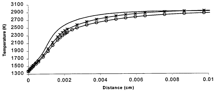
Figure 32: Temperature profile in the downstream direction of a burner-stabilised premixed MT mixtures: ___stoichiometric, -* UK Flare, -o- US igniter.
