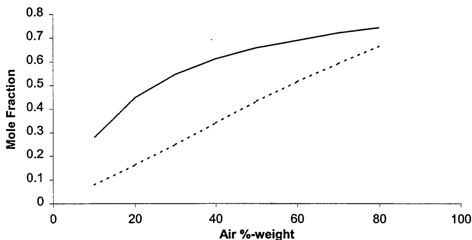
Figure 16: Concentration profile of N_2 for MTV-1 reacting with air : - - - MTV-air, ___ MTV products-air.
