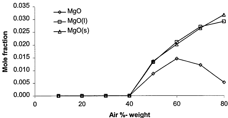
Figure 10: Effect of air on the concentration of magnesium oxides of MTV combustion.
