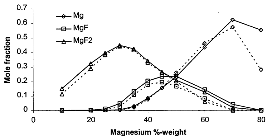
Figure 3: Equilibrium mole fraction profiles of major species of MT composition: inlet temperature 1366K: - - - gaseous species only, — liquid and solid phases are also included.
