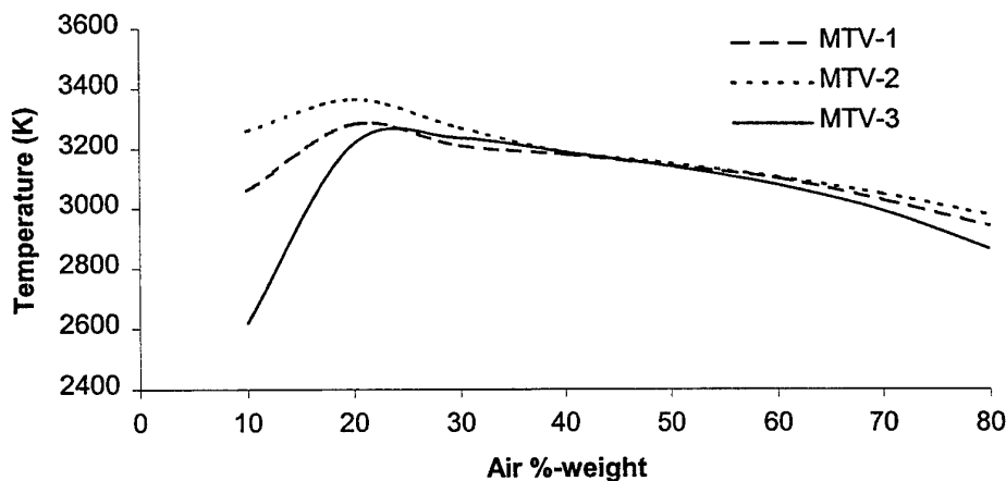
Figure 13: Temperature profiles for reaction between combustion products of various MTV compositions and air.
