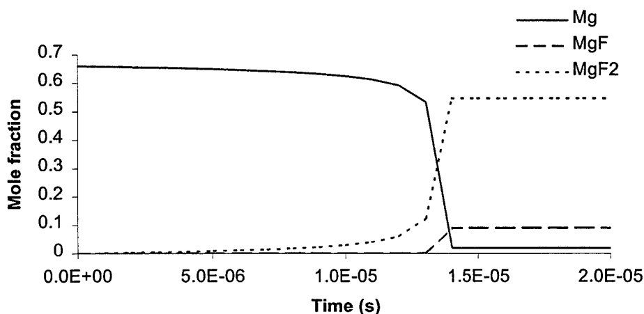
Figure 18: Time evolution of major species for a stoichiometric MT composition.
