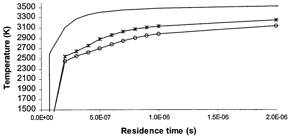
Figure 26: Flame temperature for different residence time of various MT compositions: ___stoichiometric, -* UK Flare, -o- US igniter.
