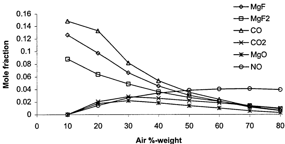
Figure 14: Concentration profiles of major species from MTV-1 products reacting with air.
