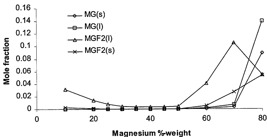
Figure 5: Equilibrium mole fraction profiles of major liquid and solid species (except carbon) of MT composition: inlet temperature 1366K.
