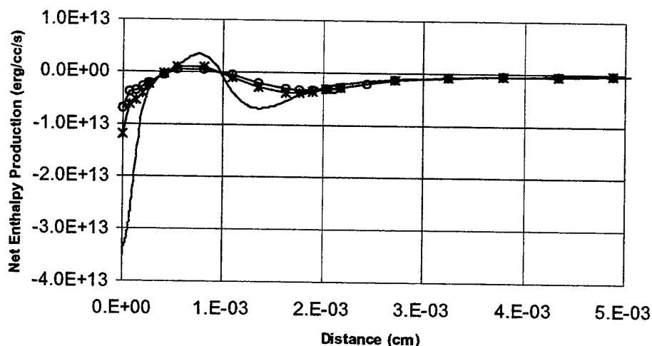
Figure 34: Net enthalpy production for different MT compositions: — stoichiometric, -*- UK Flare, -o- US igniter..
