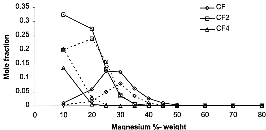
Figure 4: Equilibrium mole fraction profiles of C-F species of MT composition: inlet temperature 1366K: --- gaseous species only, — liquid and solid phases are also included.
