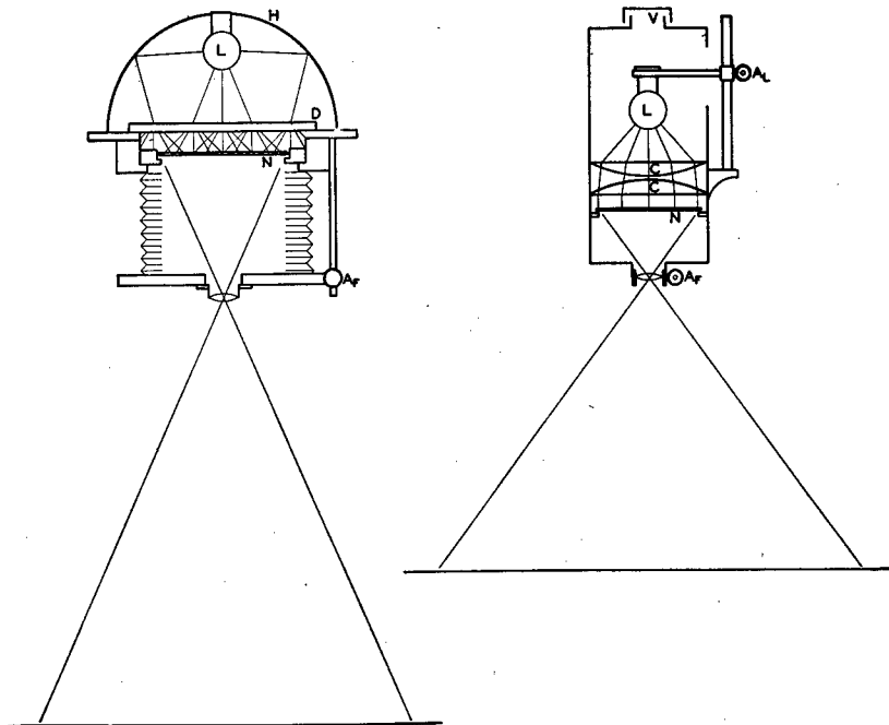
FIGURE 69.—Projection printers.
