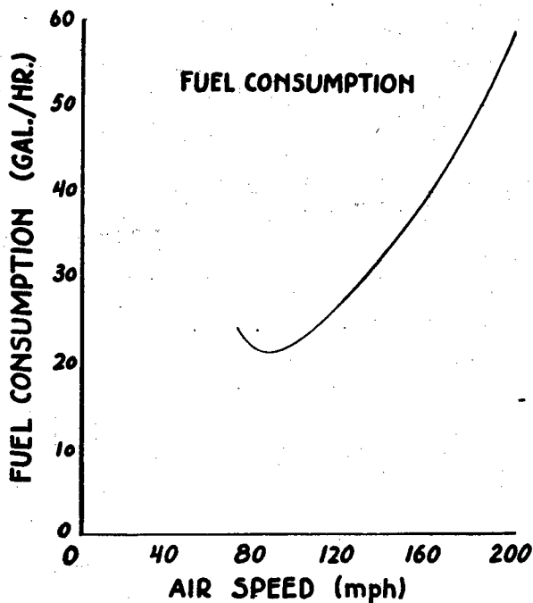
FIGURE 30.—Typical fuel consumption curve.
