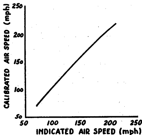
FIGURE 27.—An air speed meter calibration curve.
