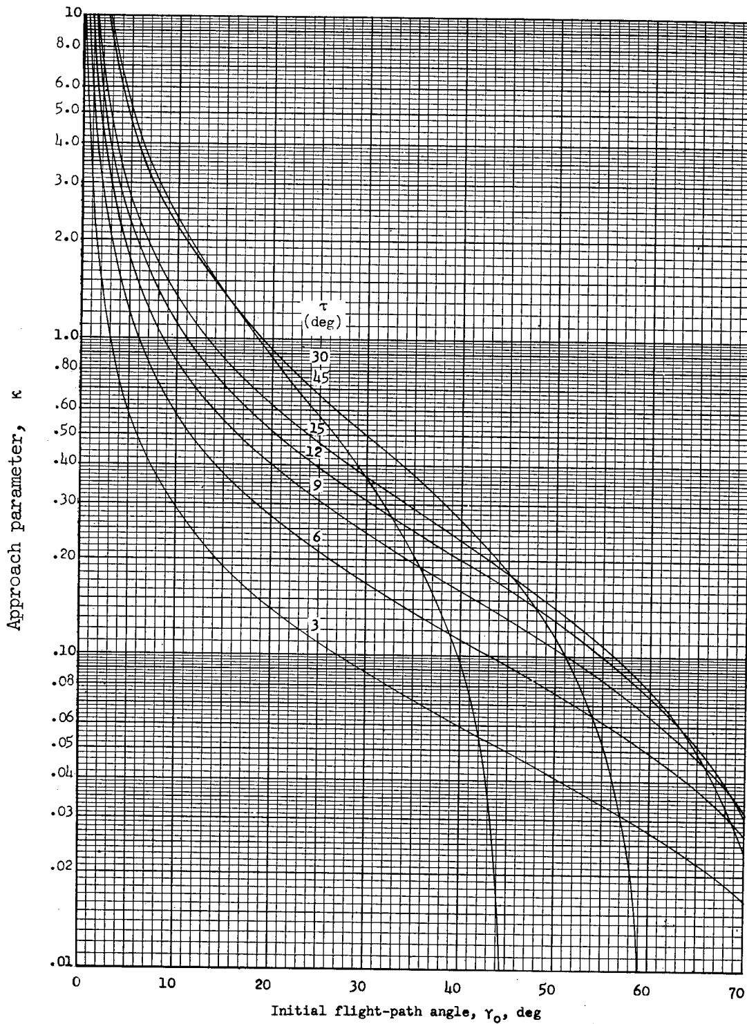
Figure 3.- Variation of approach parameter with trim and flight-path angle.
