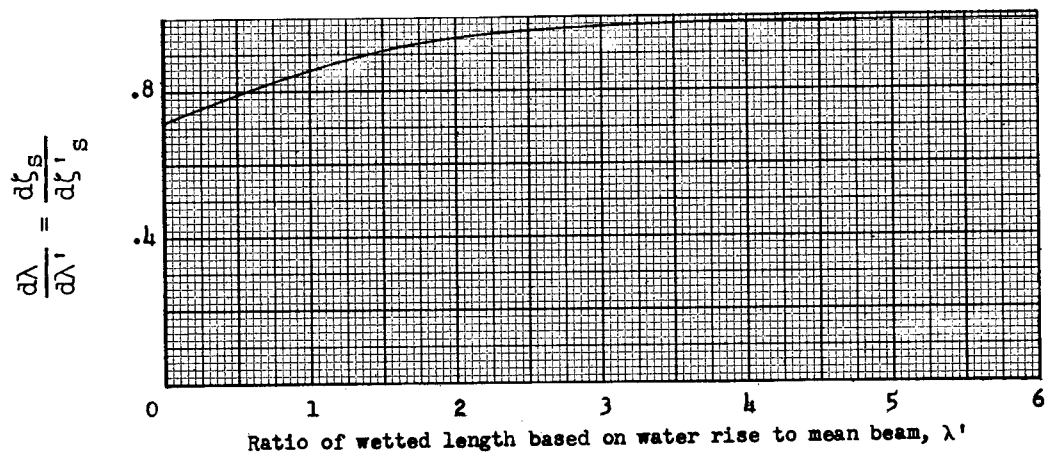
(b) Variation of derivative of wetted-length ratio with ratio of wetted length based on water rise to mean beam.
