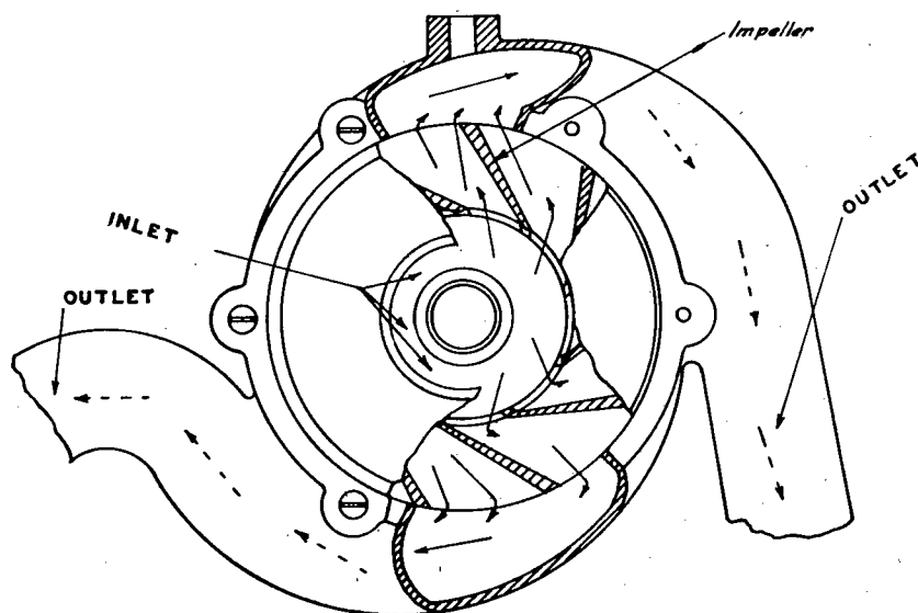
FIGURE 46.—Coolant pump.
