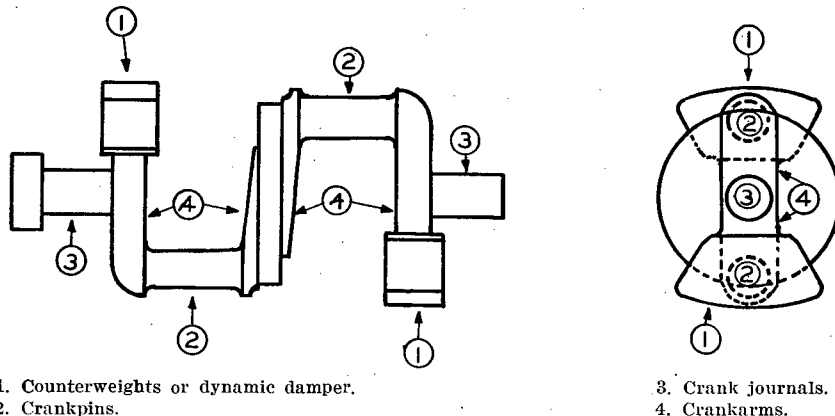
FIGURE 26.—Typical 180° crankshaft.
