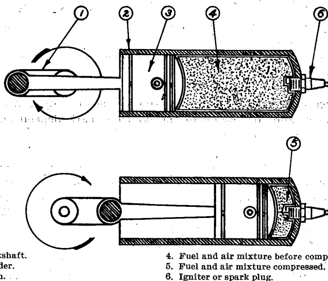
FIGURE 1.—Method of converting heat energy to mechanical energy in an internal-combustion engine.
