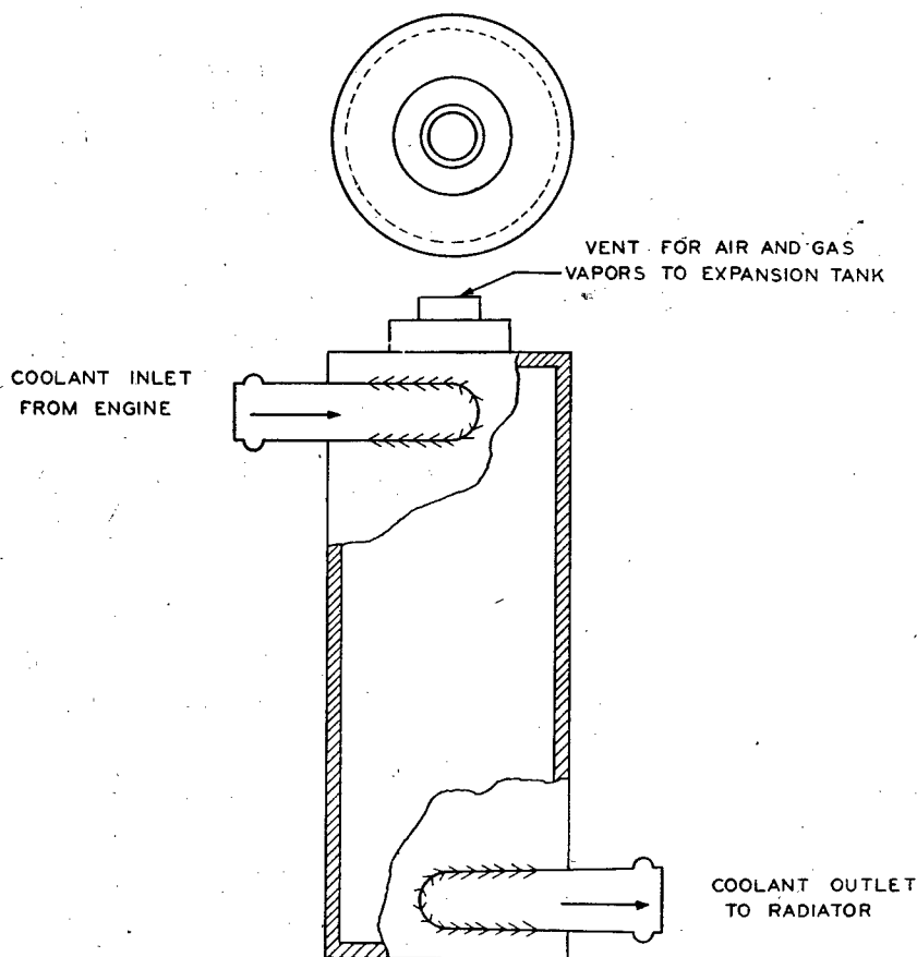
FIGURE 53.—Centrifuge chamber.
