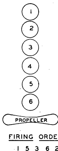
FIGURE 11.—Cylinder numbering and firing order of 6-cylinder in-line engine.
