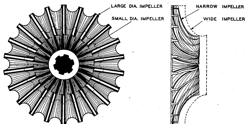
FIGURE 30.—Impellers.
