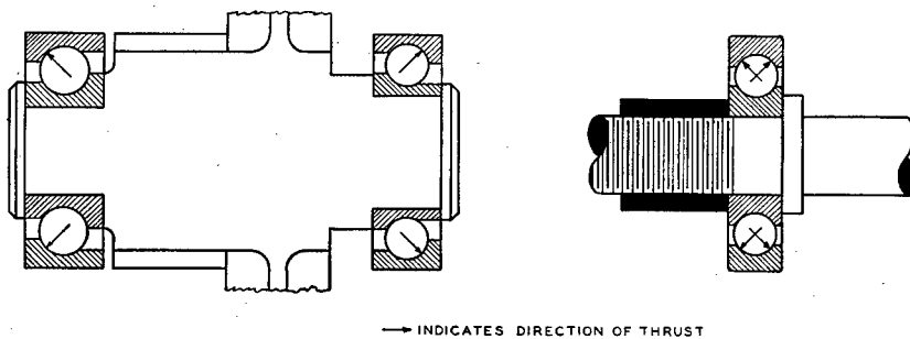
① FIGURE 28.—Types of thrust bearings.
