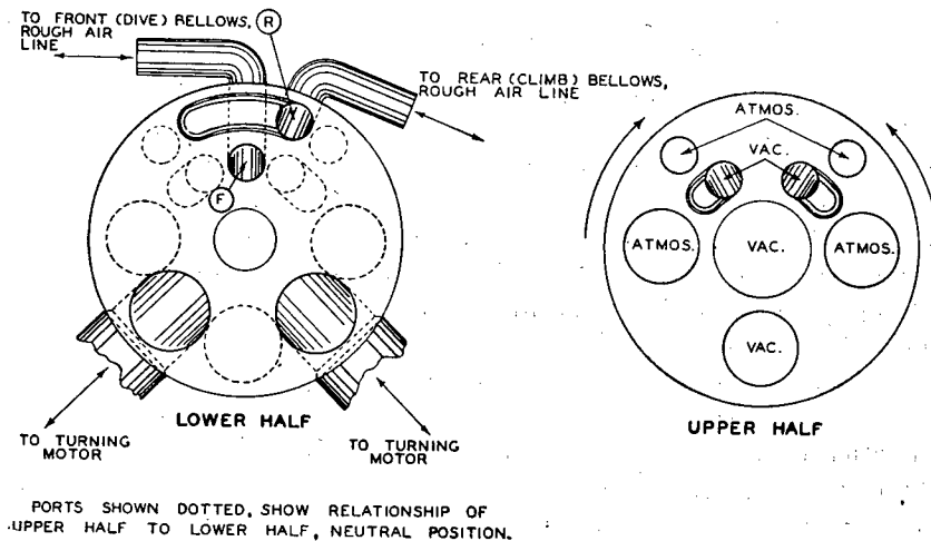
FIGURE 70.—Rudder valve.
