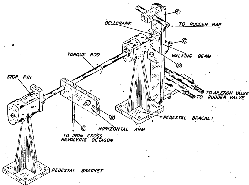
FIGURE 81.—Bank turner.
