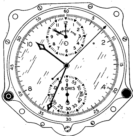
FIGURE 107.—A-8 clock (face).
