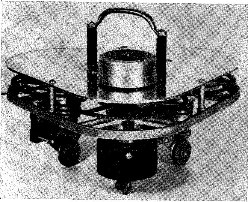
FIGURE 41.—Automatic recorder.
