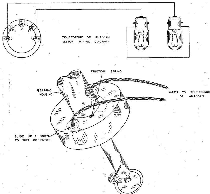
FIGURE 62.—Recorder lights.
