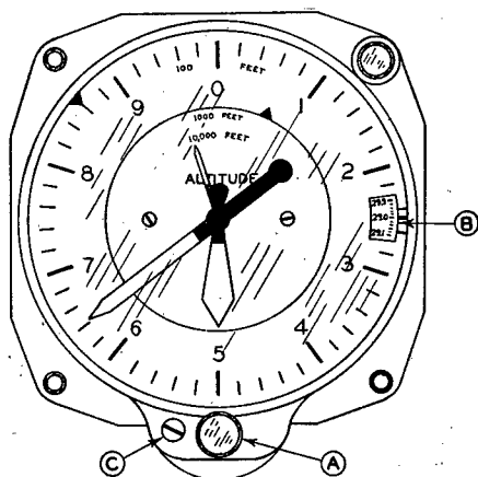
FIGURE 100.—Altimeter (face).
