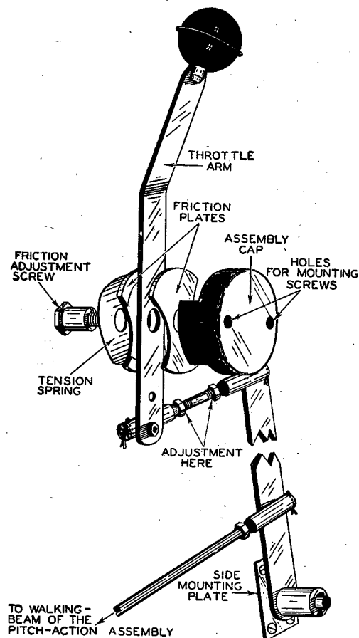
FIGURE 86.—Throttle assembly.
