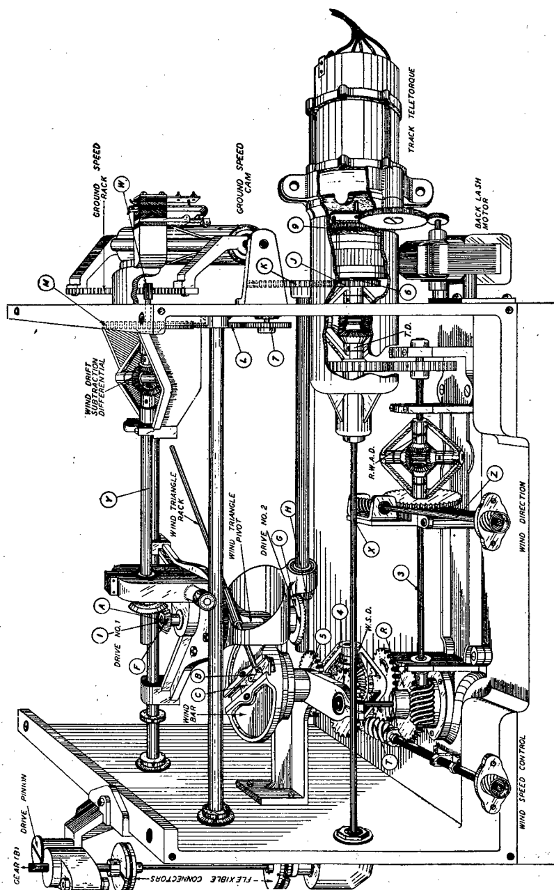
FIGURE 120.—Wind drift mechanism.
