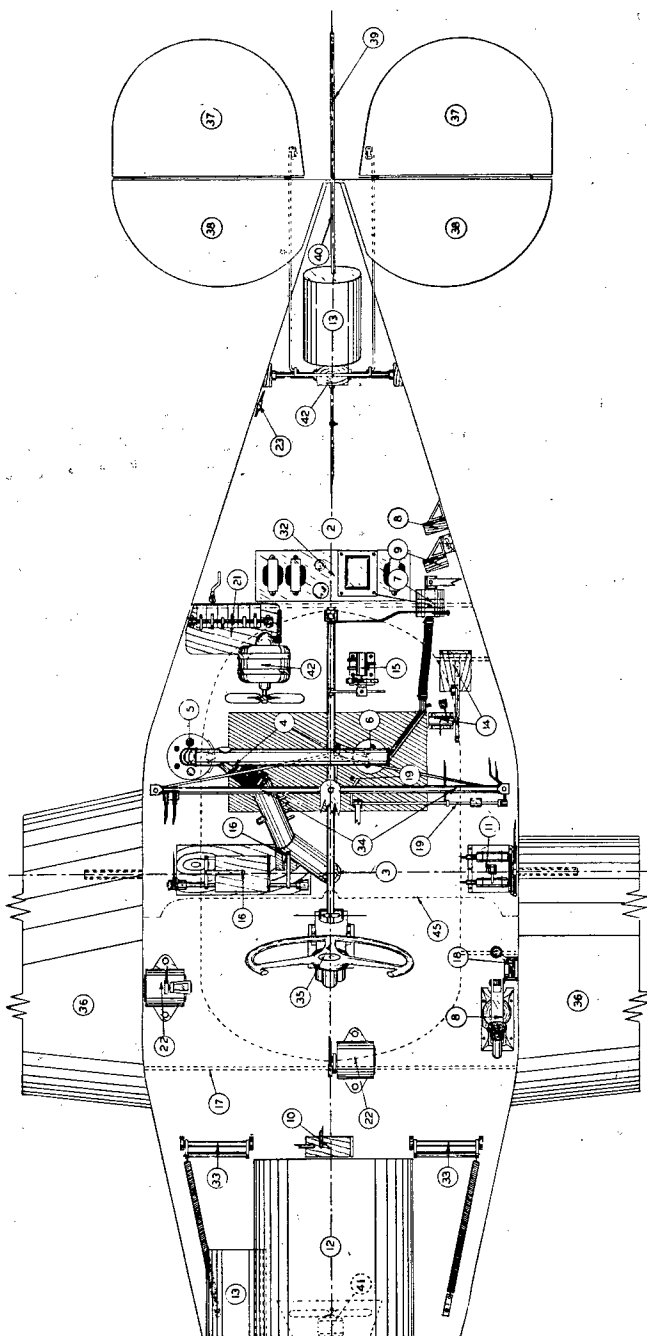
FIGURE 2.—Fuselage—top view.
