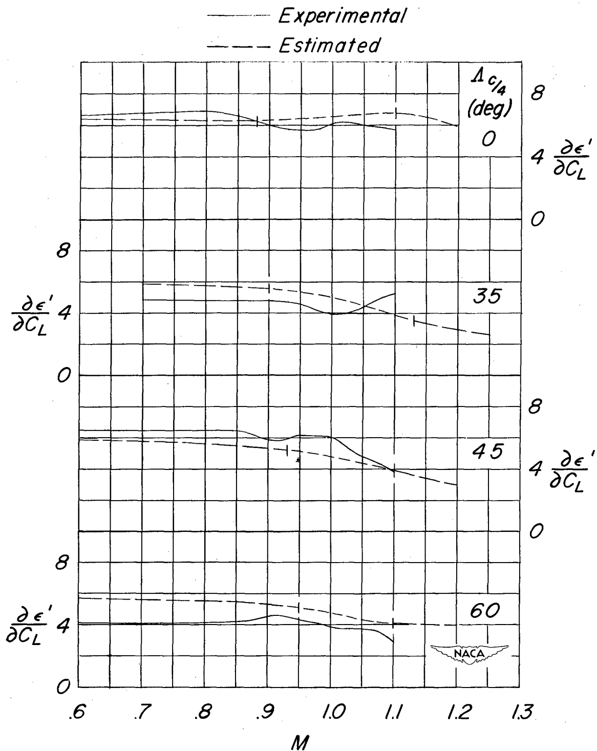
Figure 47.- Comparison of experimental and estimated variation of floating-angle parameter \partial \epsilon' / \partial C_L with Mach number for various sweep angles. Wing and fuselage; z = 0.3 ; A = 4 ; \lambda = 0.6 ; \frac{t}{c} = 0.06 .
