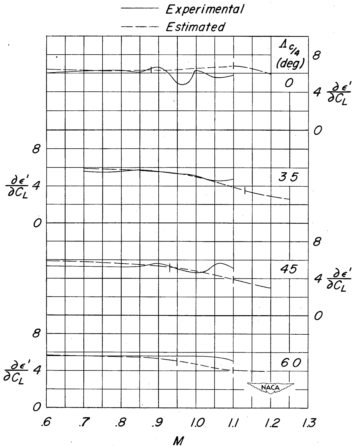
Figure 46.- Comparison of experimental and estimated variation of floating-angle parameter \partial \epsilon' / \partial C_L with Mach number for various sweep angles. Wing alone; z = 0.3 ; A = 4 ; \lambda = 0.6 ; \frac{t}{c} = 0.06 .
