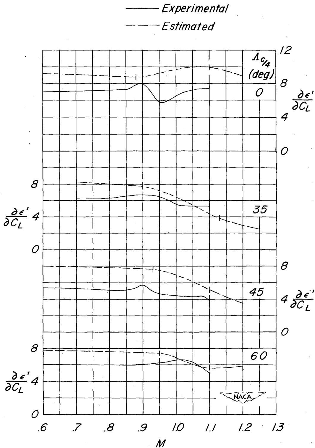
Figure 44.- Comparison of experimental and estimated variation of floating-angle parameter \partial \epsilon' / \partial C_L with Mach number for various sweep angles. Wing alone; z = 0 ; A = 4 ; \lambda = 0.6 ; \frac{t}{c} = 0.06 .
