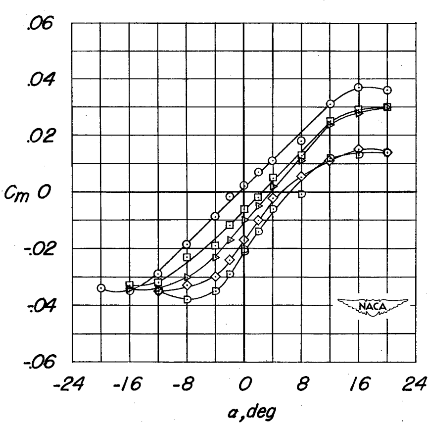
(e) M = 0.95 .
