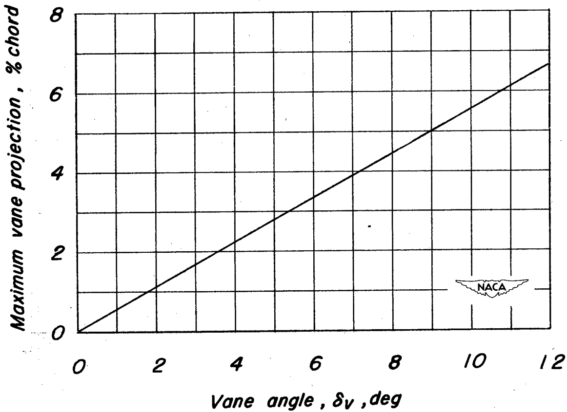
Figure 4.- Vane geometry. (Vaness in vertical position.)
