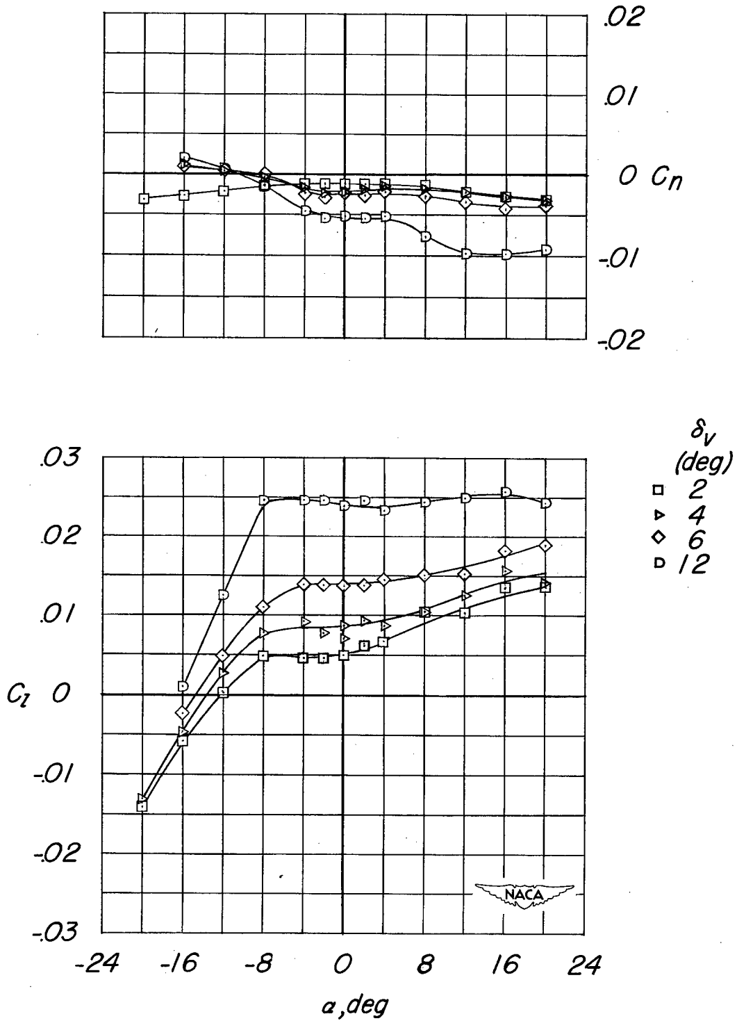
(a) M = 0.60 .
