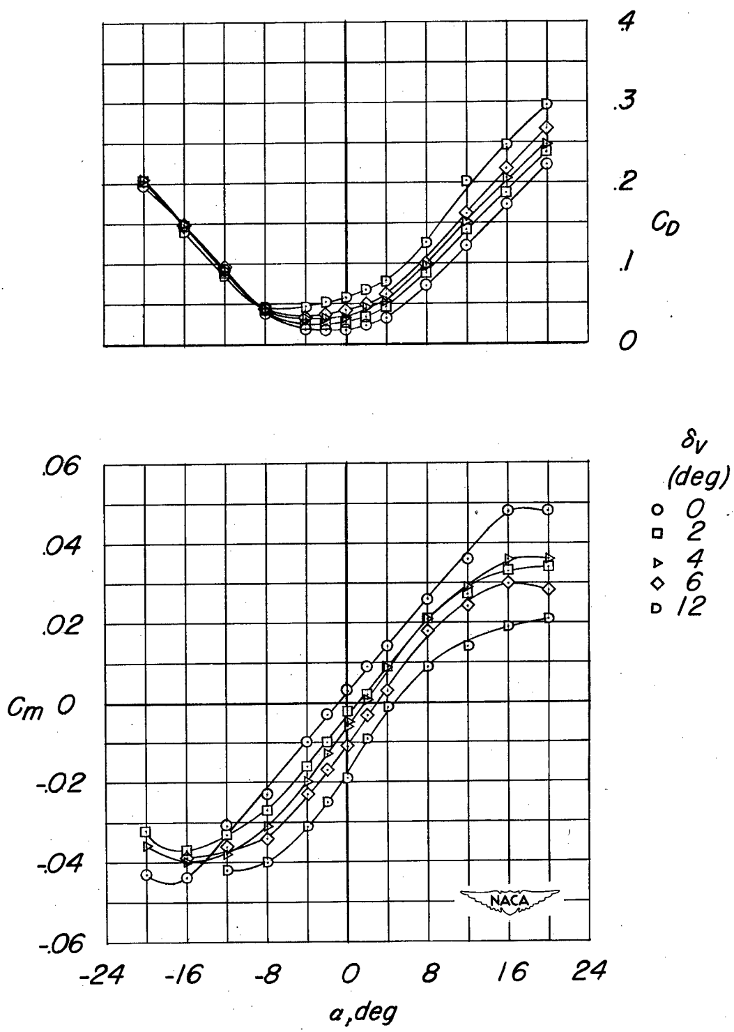
(b) M = 0.70 .
