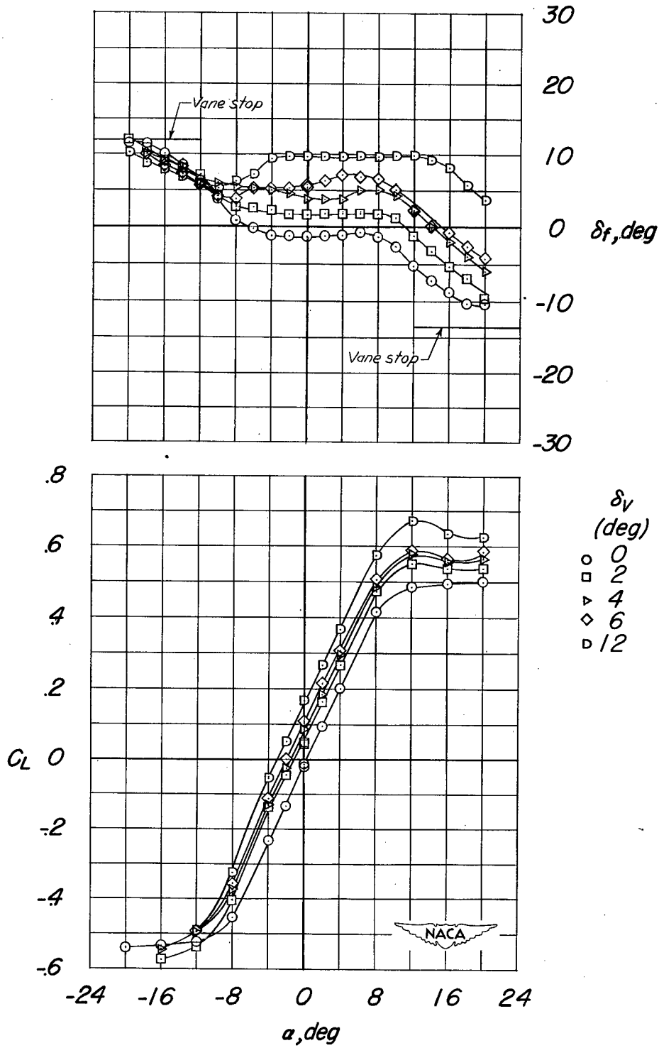
(e) M = 0.95 .
