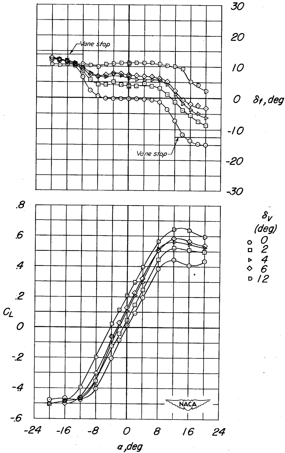
(c) M = 0.80 .
