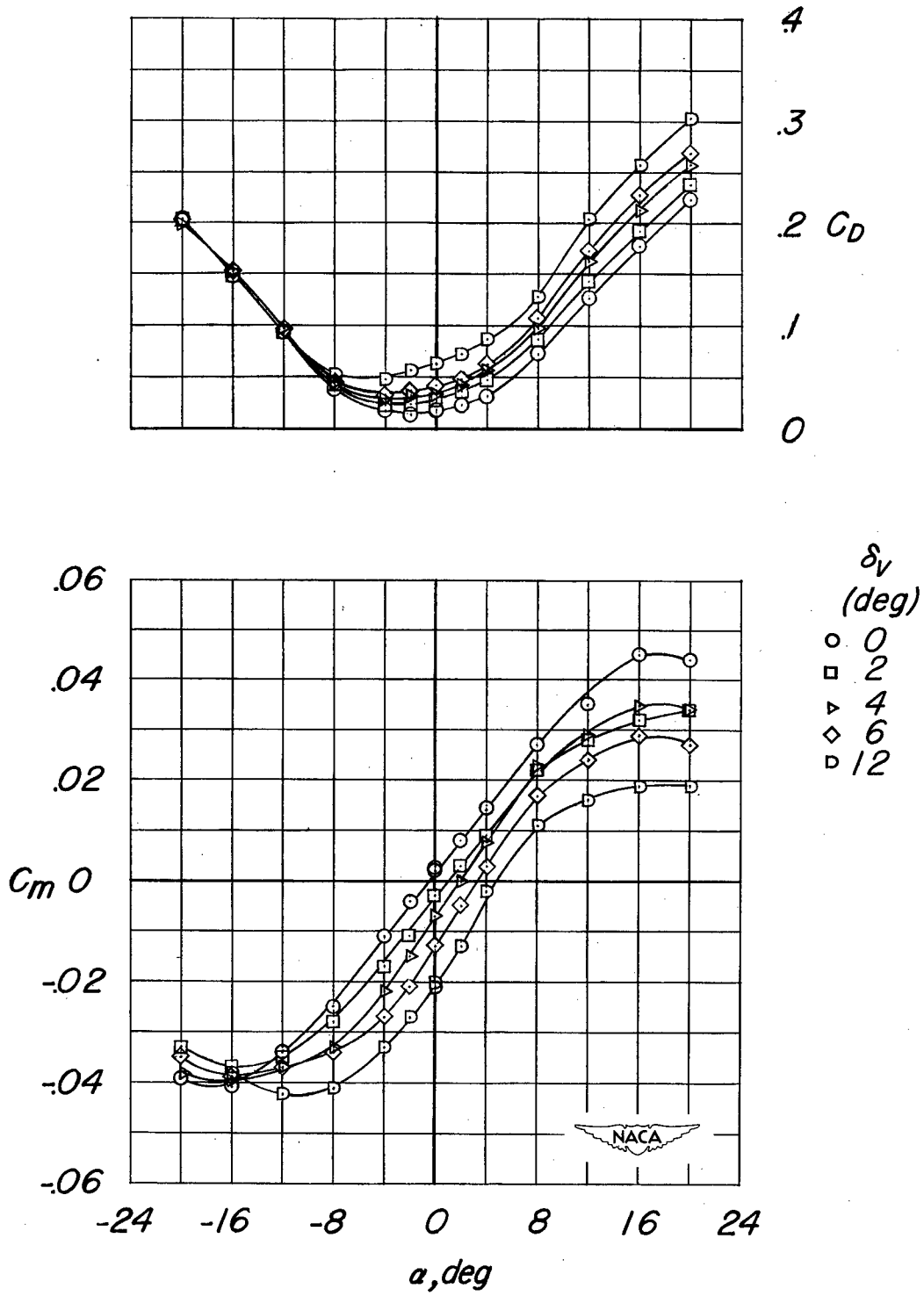
(c) M = 0.80 .
