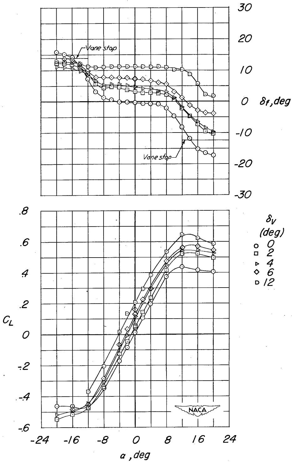
(b) M = 0.70 .
