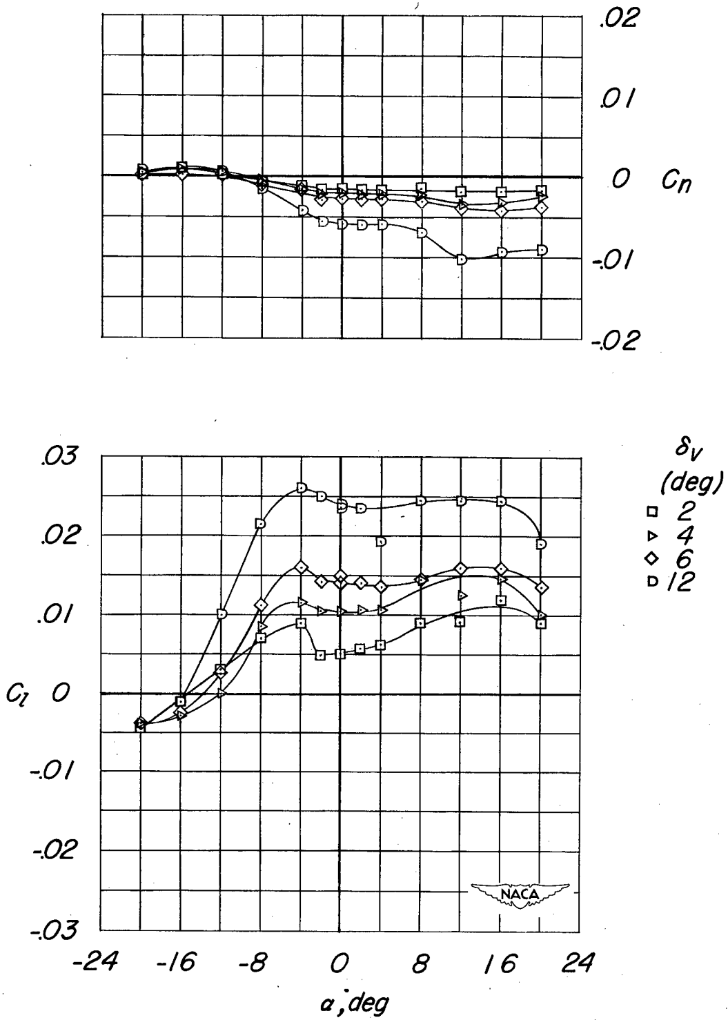
(c) M = 0.80 .
