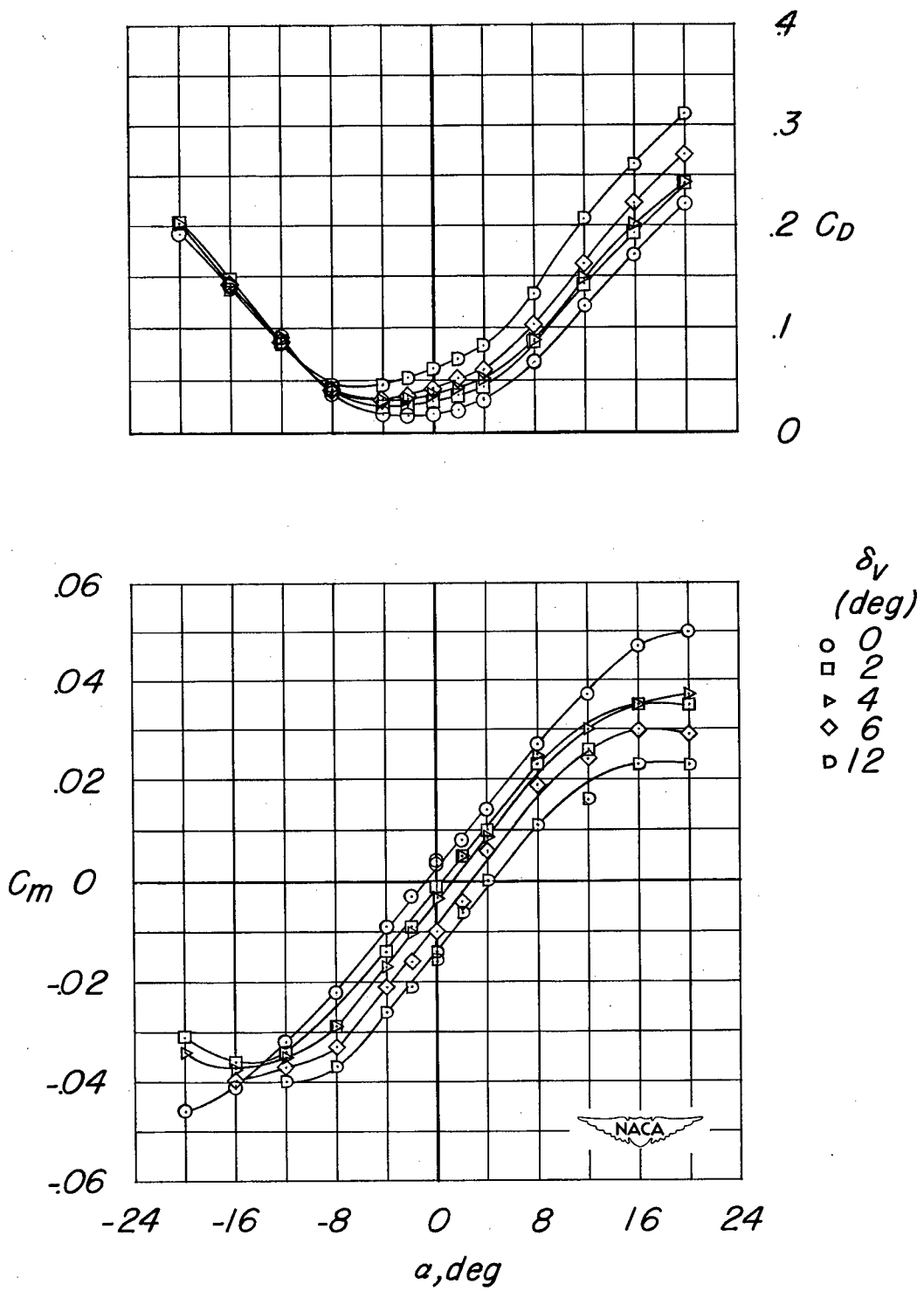
(a) M = 0.60 .
