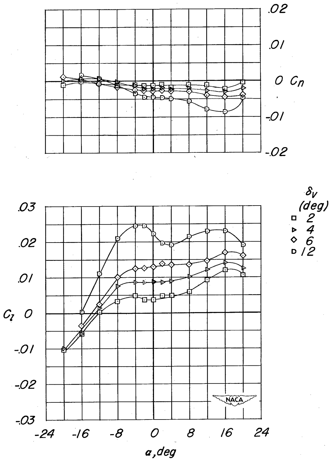
(b) M = 0.70 .
