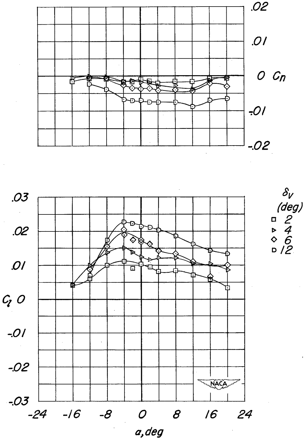
(e) M = 0.95 .
