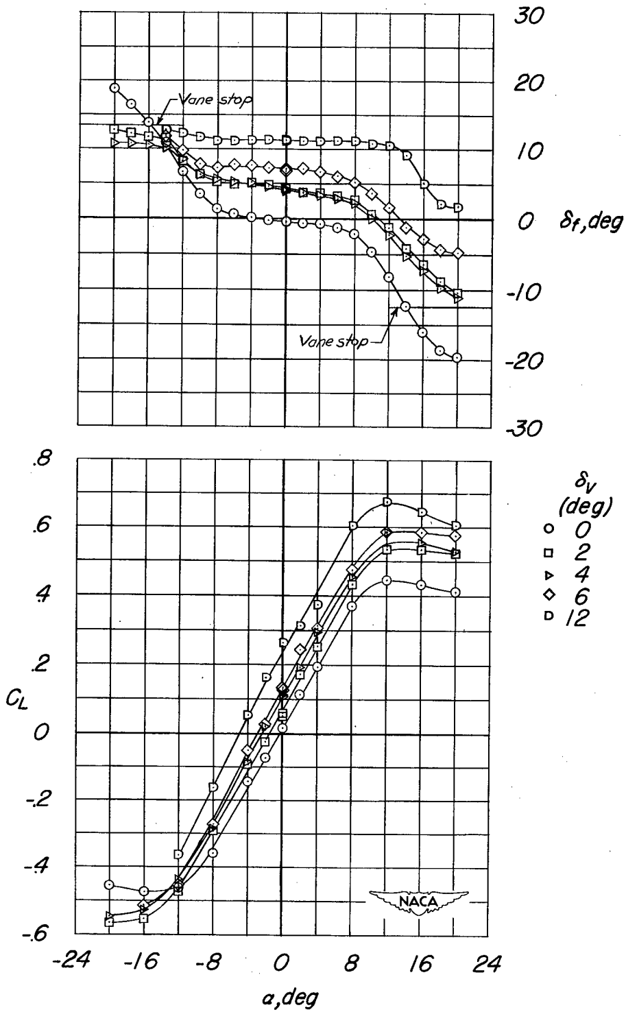
(a) M = 0.60 .
