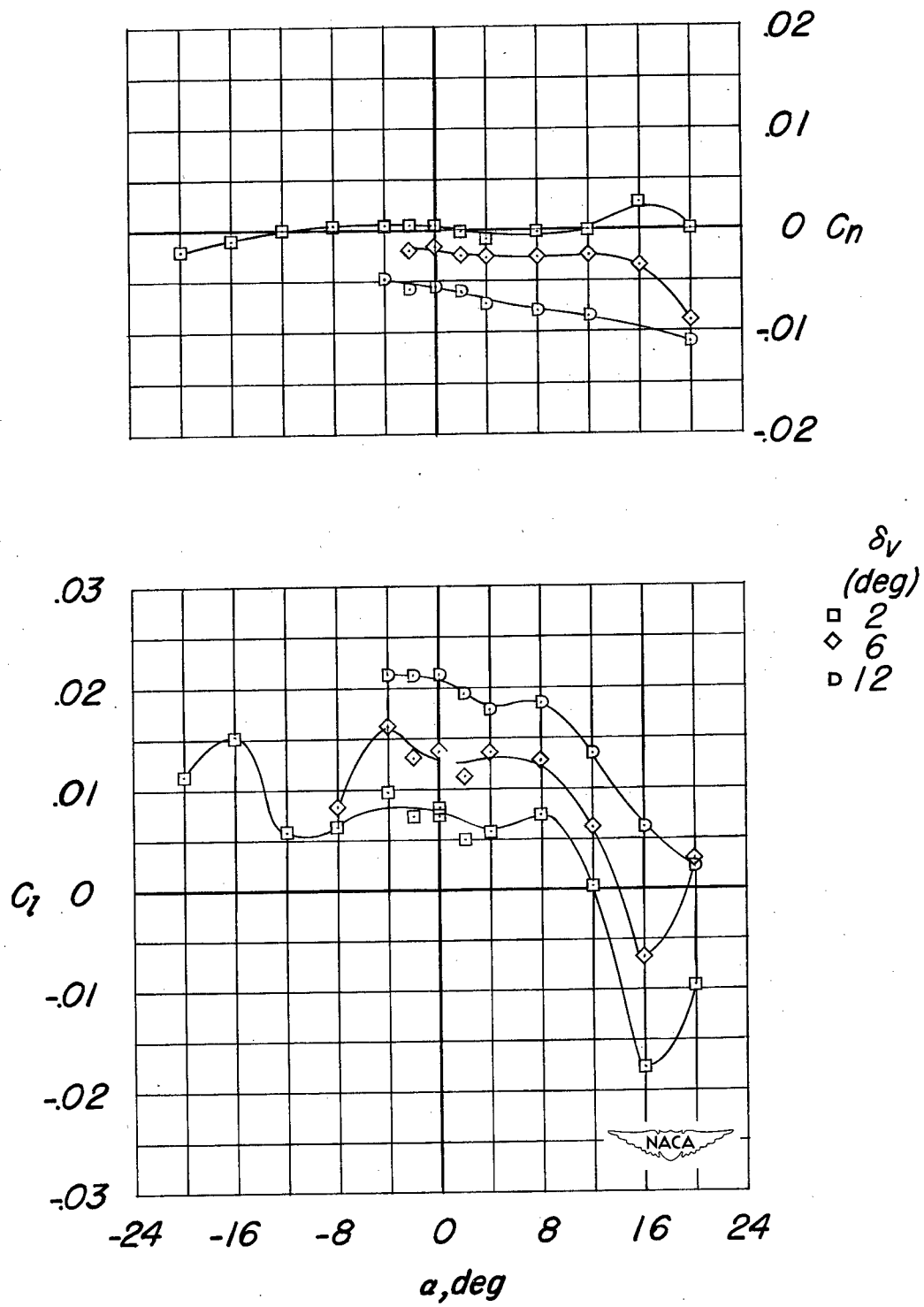
Figure 9.- Concluded.
