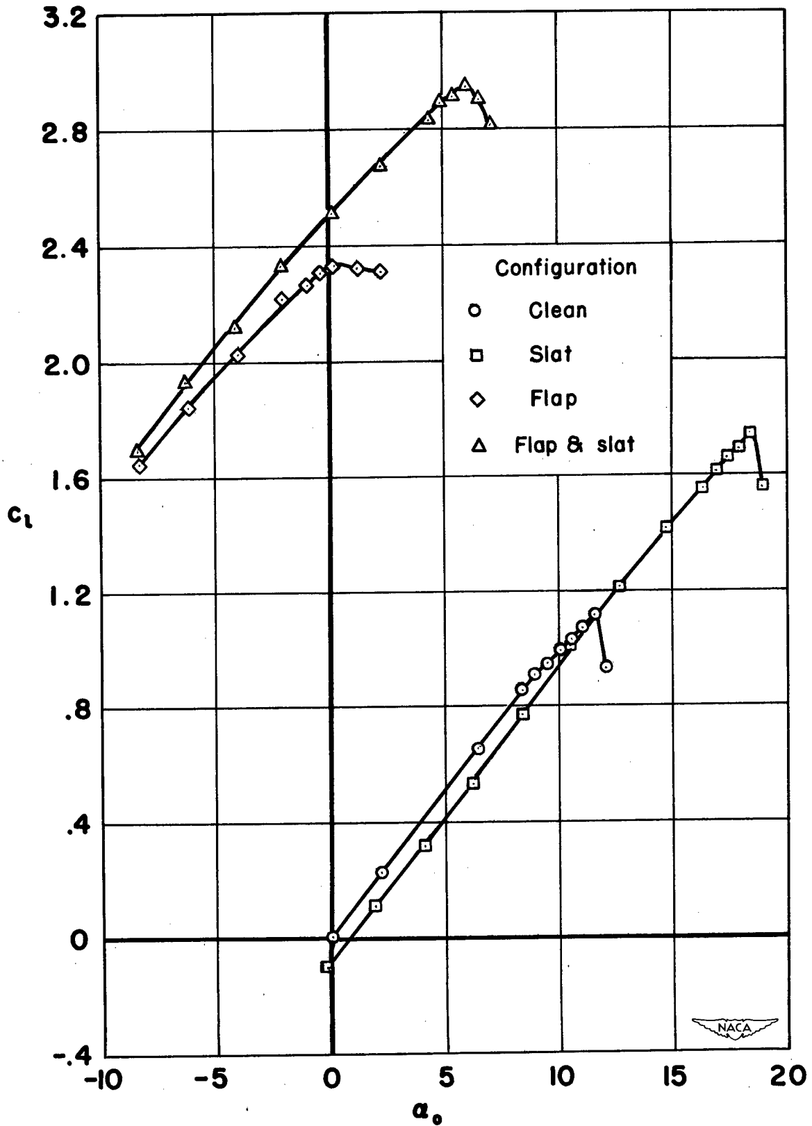
Figure 5.- Two-dimensional lift characteristics of the NACA 64A010 section with various combinations of slats and double-slotted flaps.
