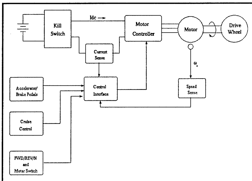
Figure 5. Solar electric vehicle drive system.
