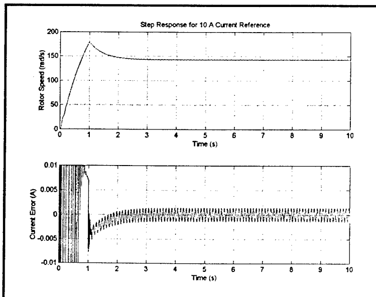
Figure 3. Step response for current controller with 10A reference.
