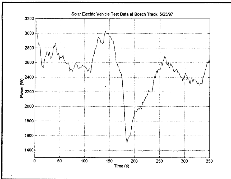
Figure 6. Solar vehicle 50 mph test without current control.
