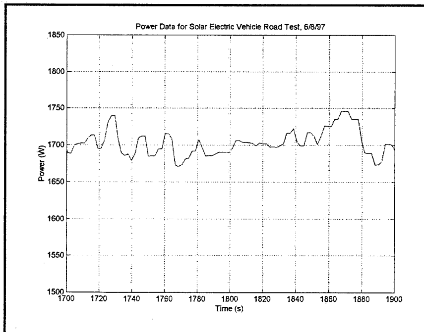
Figure 7. Solar vehicle 40 mph test with current control.
