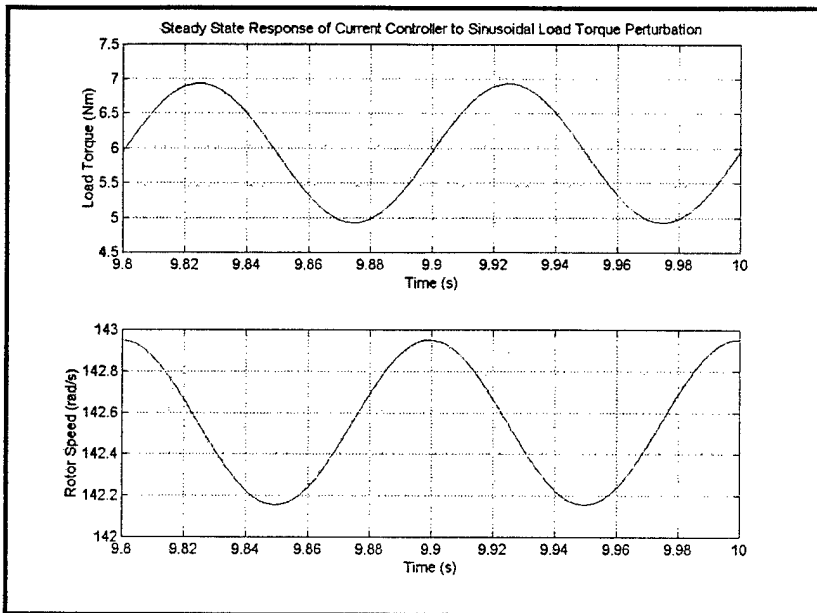
Figure 4. Steady-state response to load torque perturbation.
