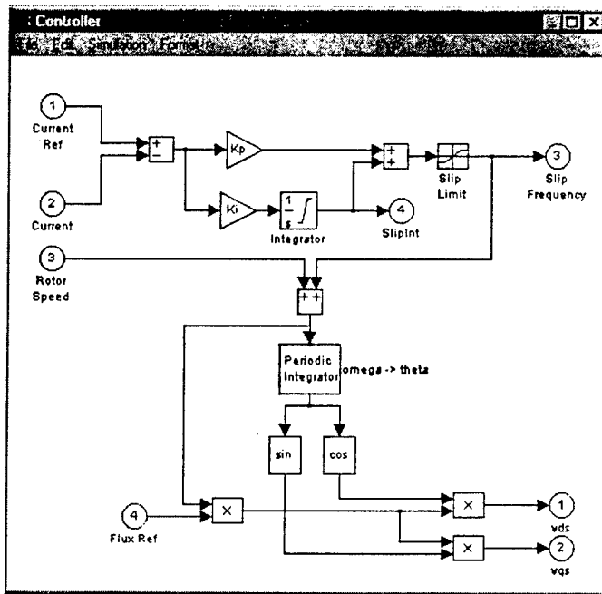
Figure 2. Bus current controller.
