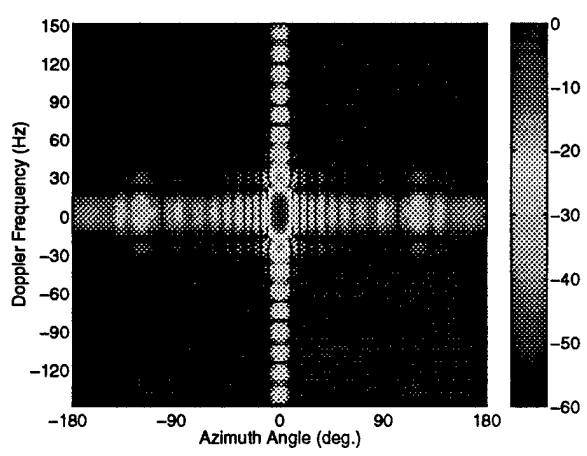
(c) Second Iteration
