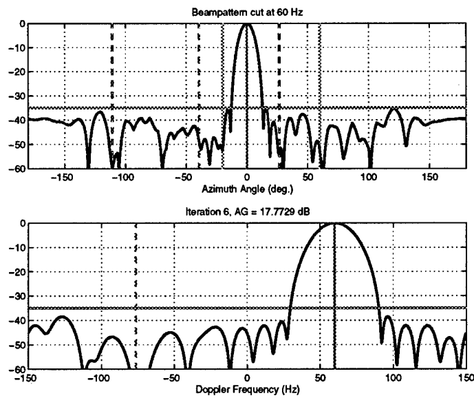
(b) Sixth Iteration beampattern cuts
