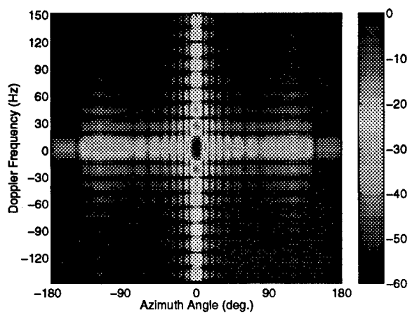
(a) Conventional beampattern
