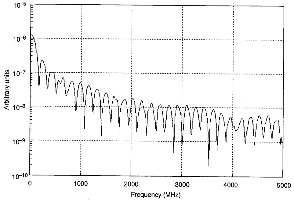
Figure 6. Fourier transform of 5-ns FWHM impulse.
