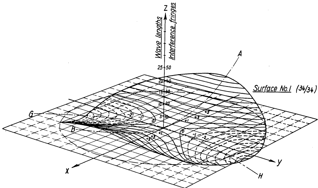
Fig.27 Perspective representation of the actual surface of the well ground and polished sample plate 36 inches in diameter, 1/4 inches thick.
