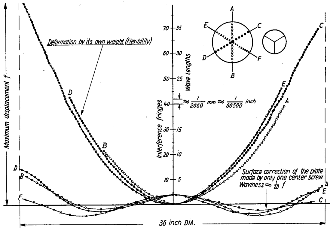
Fig.29 The deformation of a well ground and polished glass plate 36 inches in diameter, \frac{1}{4} inches thick by only one center screw while supported between 12 screws and lock screws along the periphery
