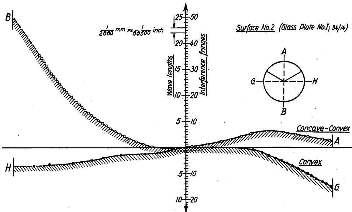
Fig. 26 . The actual surface profile of a well ground and polished sample plate 36 inches in diameter, 1/4 inches thick, prepared as a plate with a uniformly curved surface and a larger number of rings in the pattern than in surface No. 1
