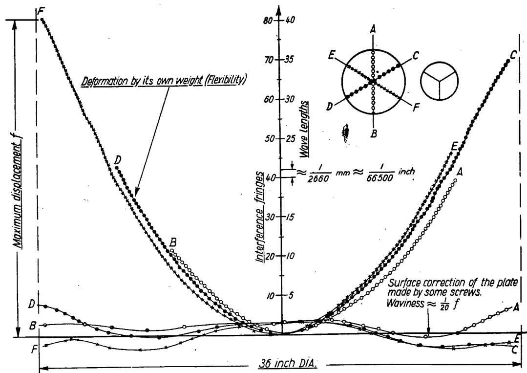
Fig.30 The deformation of a well ground and polished glass plate 36 inches in diameter, \frac{1}{4} inches thick by several screws while supported between 12 screws and lock screws along the periphery.
