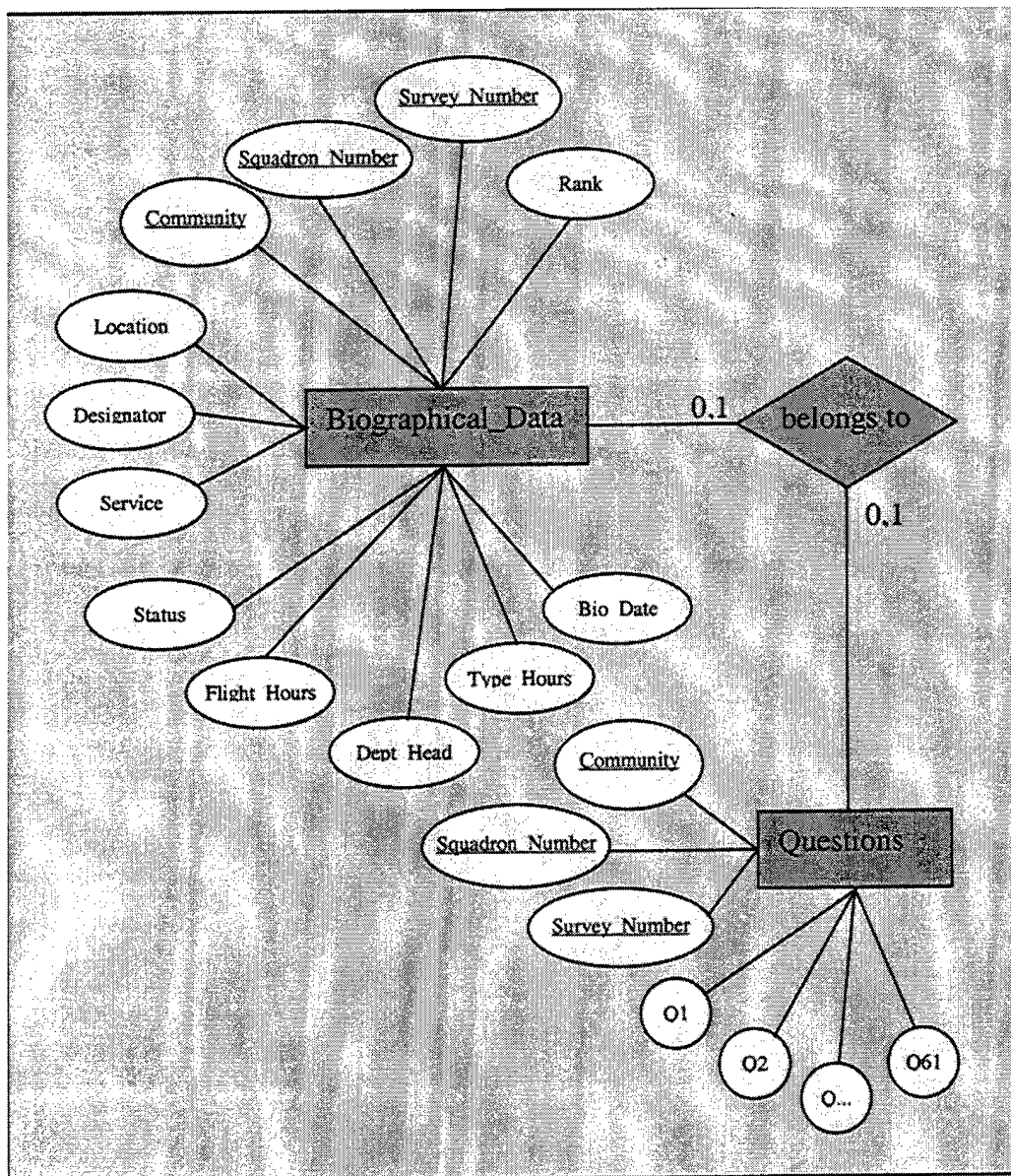
Figure 3: ER Diagram for Original Database
