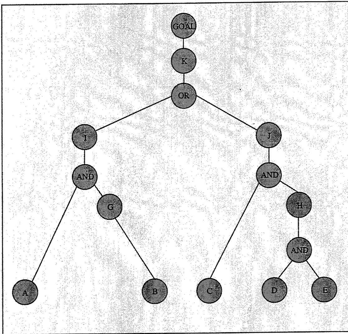
Figure 8: Backward Chaining Inference Tree
