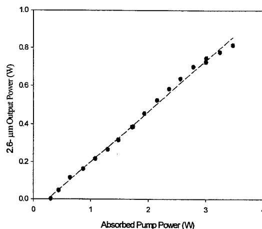
Figure 6b: 6.5-W Exp. (1,1.5 mm pump semiaxes)
