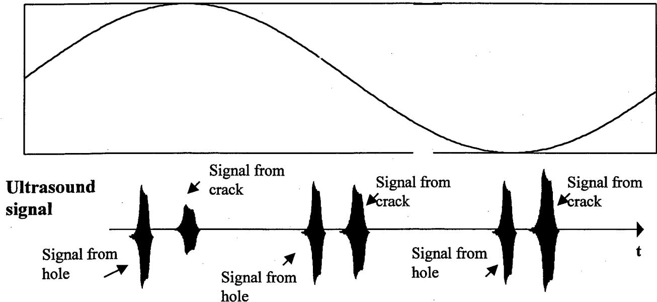
Figure 7.2.. The time tracks of the ultrasound signal reflected at different phases of the vibration.
