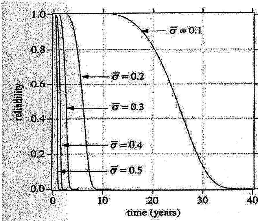
Figure 2.5. The reliability function for various level of normalized applied stress \sigma/\sigma_y
