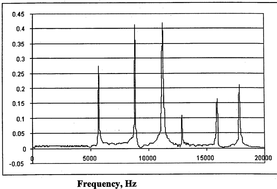
Figure5.4. The spectrum of impulse produced vibration
