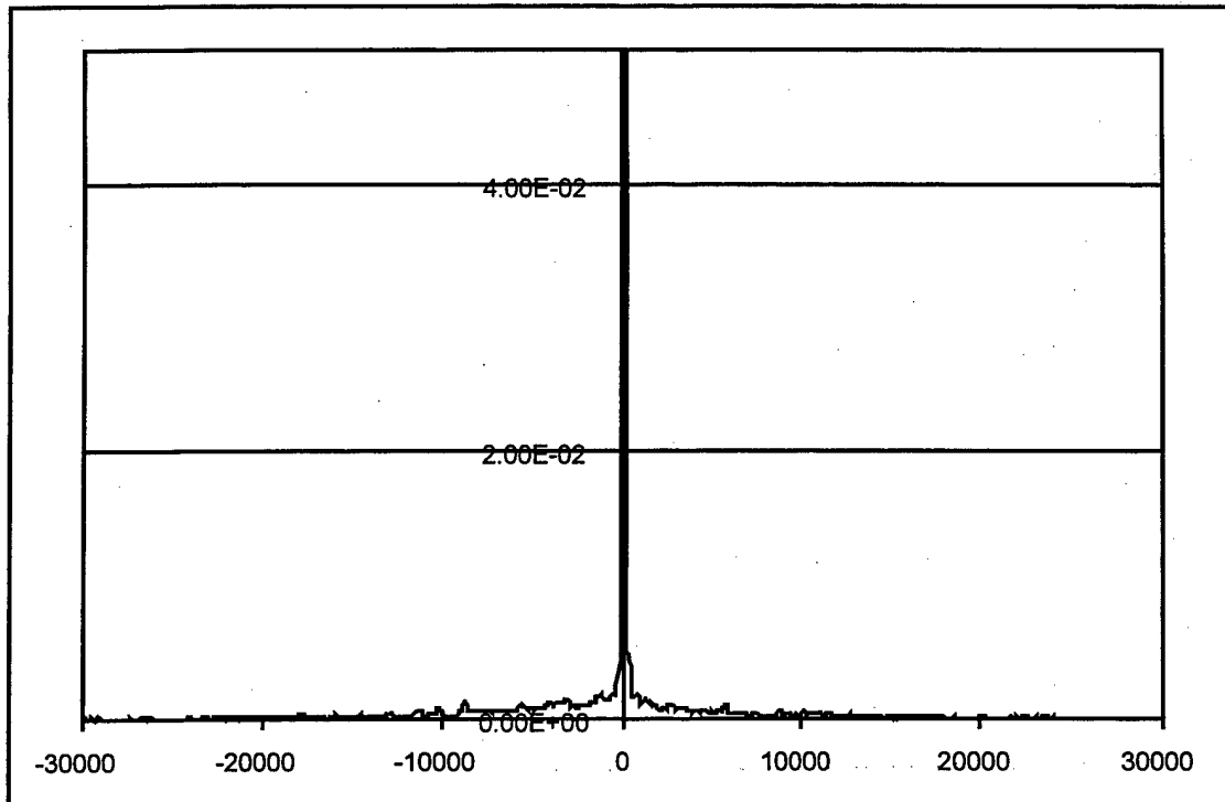
Figure 5.7. Averaged summation spectrum for sample #A1, uncracked
