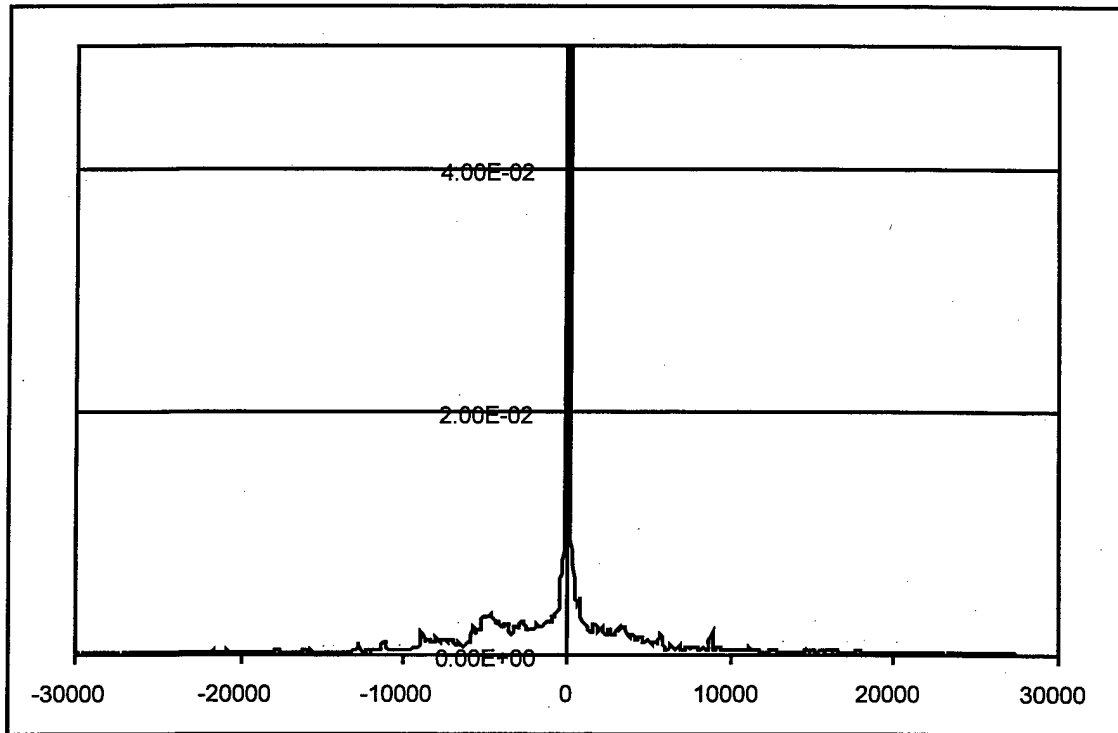
Figure 5.11. Averaged summation spectrum for sample #A5, uncracked
