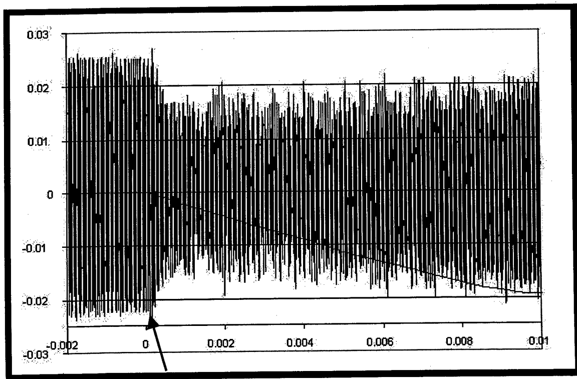
Figure 4.5. The time series of the detected signal signal from the bearing cap with crack ( frequency 205 kHz). The moment of impact is shown by arrow and it is seen the amplitude modulation of the received signal after impact.
