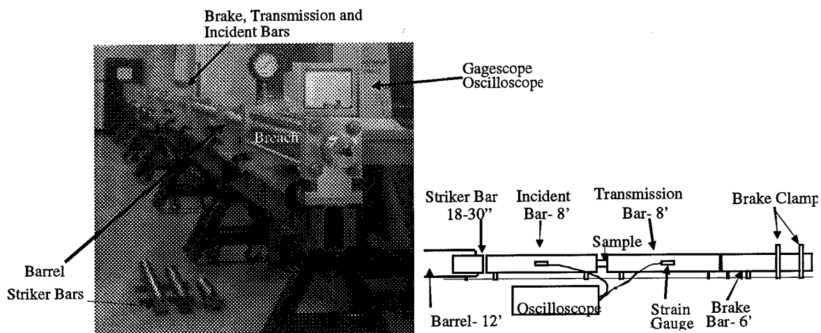
Figure 4.1: Photograph and schematic of 3-inch Hopkinson Bar
