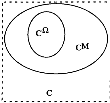
Figure 3.2: Basic schematic of double inclusion method
