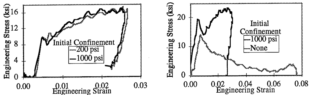
Figure 4.11: Effect of initial confinement on concrete response and response of radially confined and unconfined concrete.
