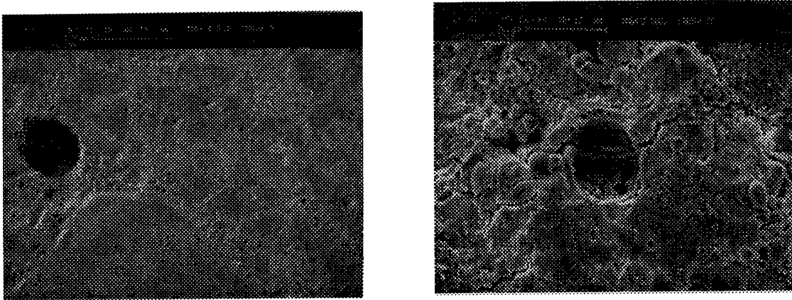
Figure 4.20: SEM micrographs of: untested concrete (25x); mortar tested in triaxial compression (500x)
