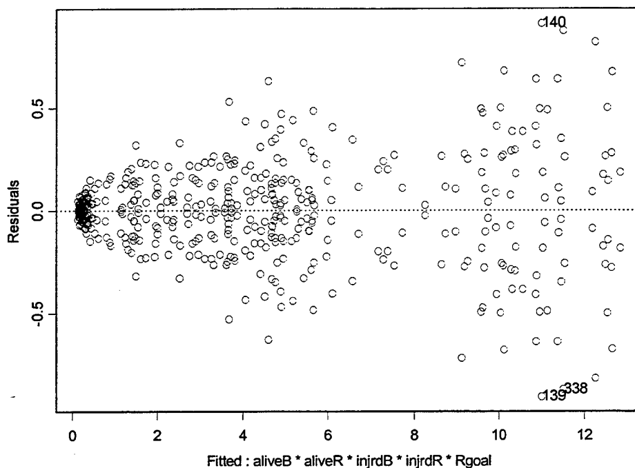
Figure 8: Residuals vs. Fitted Values of the variables. The funnel shaped plot strongly suggests that the standard deviation increases as the mean value increases.
