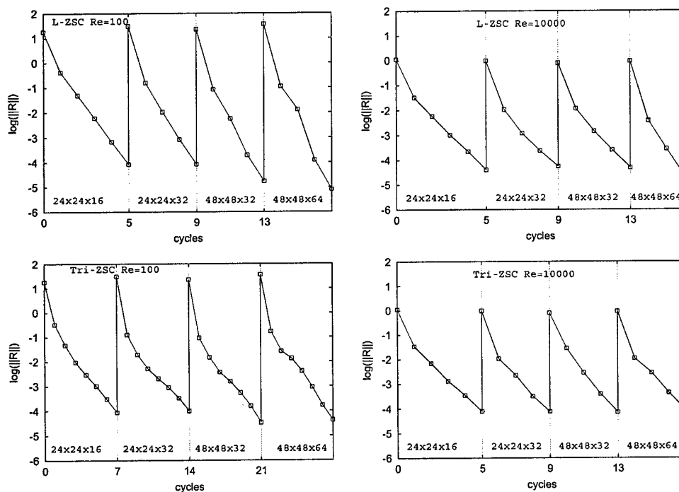
FIG. 4.8. L_2 -norm of the residual versus F(2,1)-cycles with lexicographic (top graphs) and tri-plane (bottom graphs) xy-plane implicit smoothers combined with z semi-coarsening (ZSC) for several grids and Reynolds numbers.
