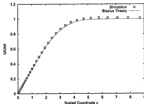
FIG. 4.7. Simulation comparison with Blasius theory at the middle of the plate with Re = 10^4 .
