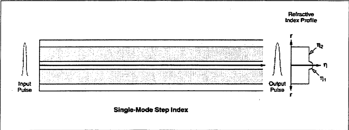
Figure 2-4. Single-mode Fiber [Ref. From Adams, 1999].
