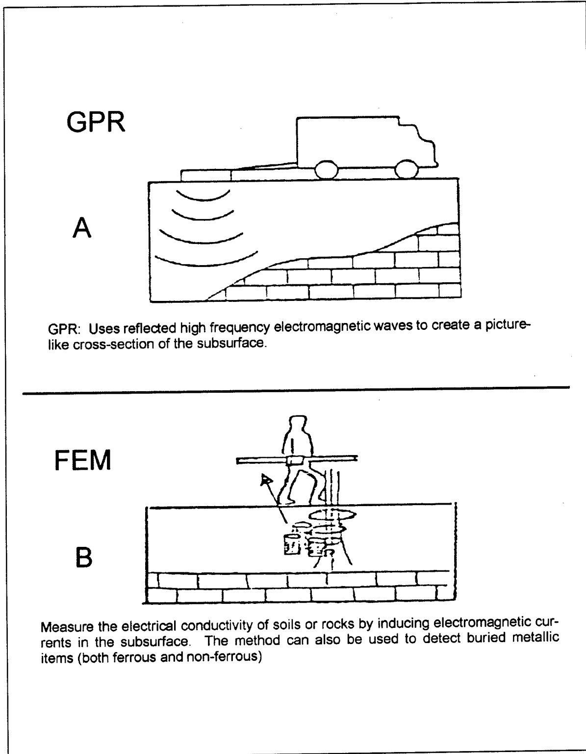
FIGURE A.1 Principles of Ground-Penetrating Radar (GPR) and Frequency Domain Electromagnetics (FEM)
