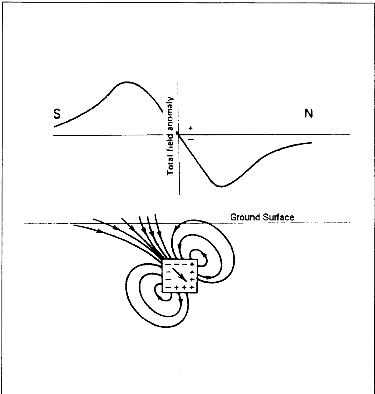
FIGURE A.7 Magnetic Response for a South-North Traverse over a Buried Ferrous Object in an Inclined Magnetic Field (Mid Latitudes, Northern Hemisphere) (Location of Object Is in Strong Gradient Area between the Relative High and Low Magnetic Anomalies)
