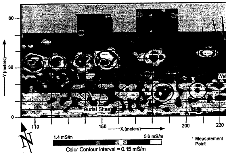
EM-31 conductivity survey over burial pits. The locations of several pits are indicated by the black circles
