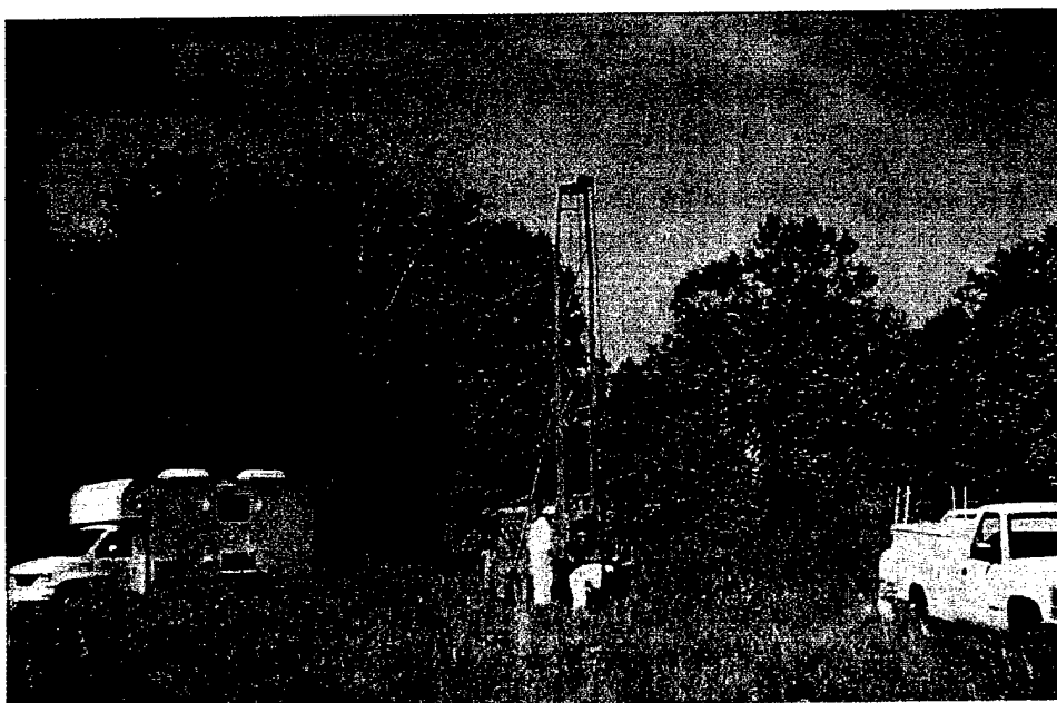
A Real Time Analytical Platform (RTAP) contained in the truck on the left is being used to monitor chemical warfare agents during intrusive sampling.
