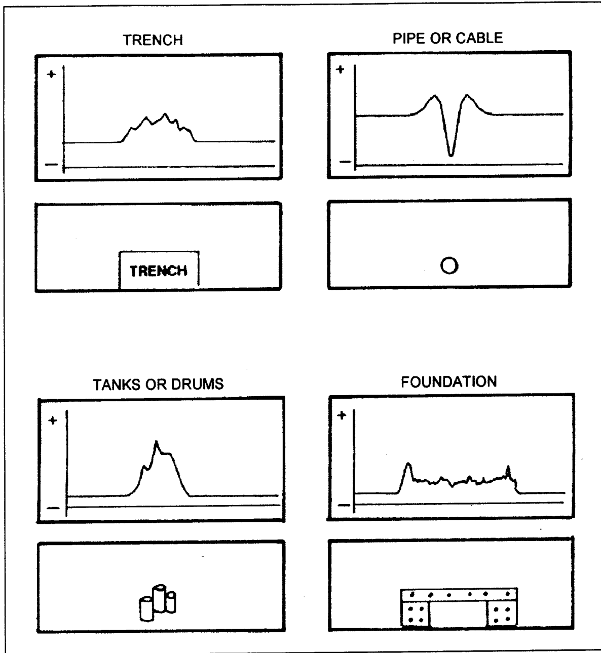
FIGURE A.11 Generalized Response of Metal Detectors to Various Objects
