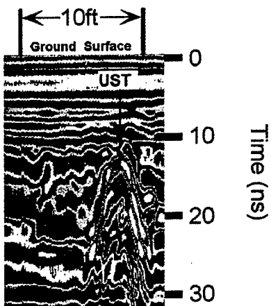
GPR profile over a buried storage tank (UST) showing the characteristic hyperbola signature.
