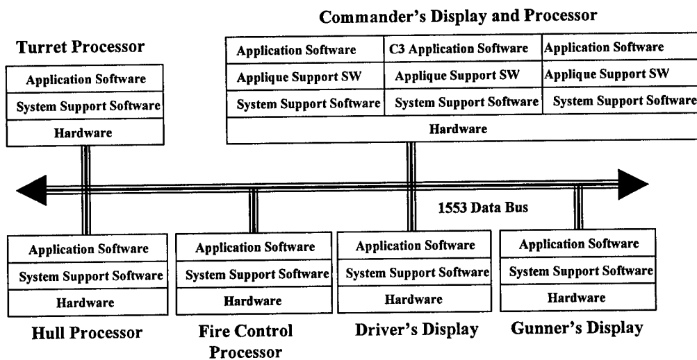
Figure 8 - M1A2 Weapons System Architecture "System of Sensors"
