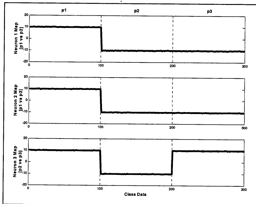
Figure III-11. Neuron Maps for Hypothetical 3-Class MSNN Typing. Each plot depicts how a trained neuron maps class data. Read vertically, the plots identifies the unique class type specifiers produced by the MSNN.
