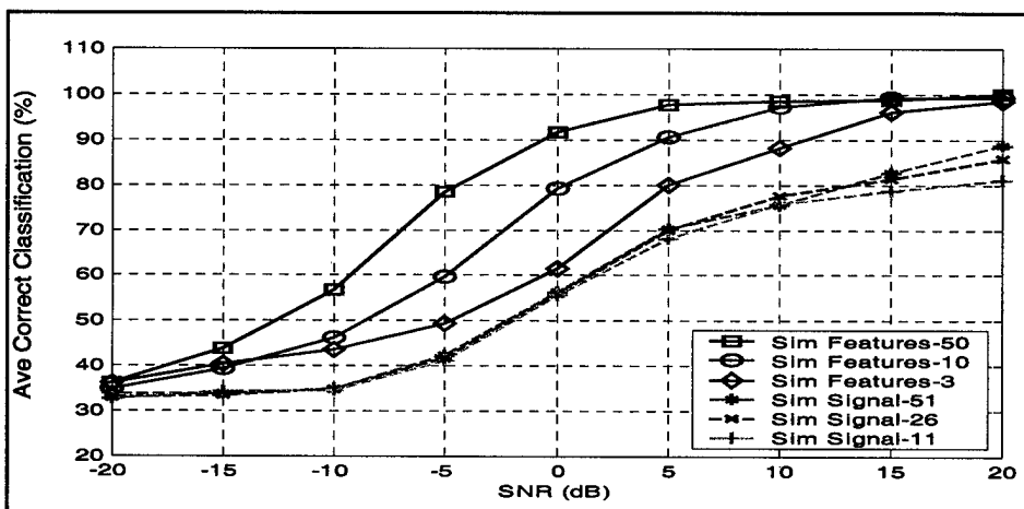
Figure B-6. MSNN Mod 3 Performance Results.
