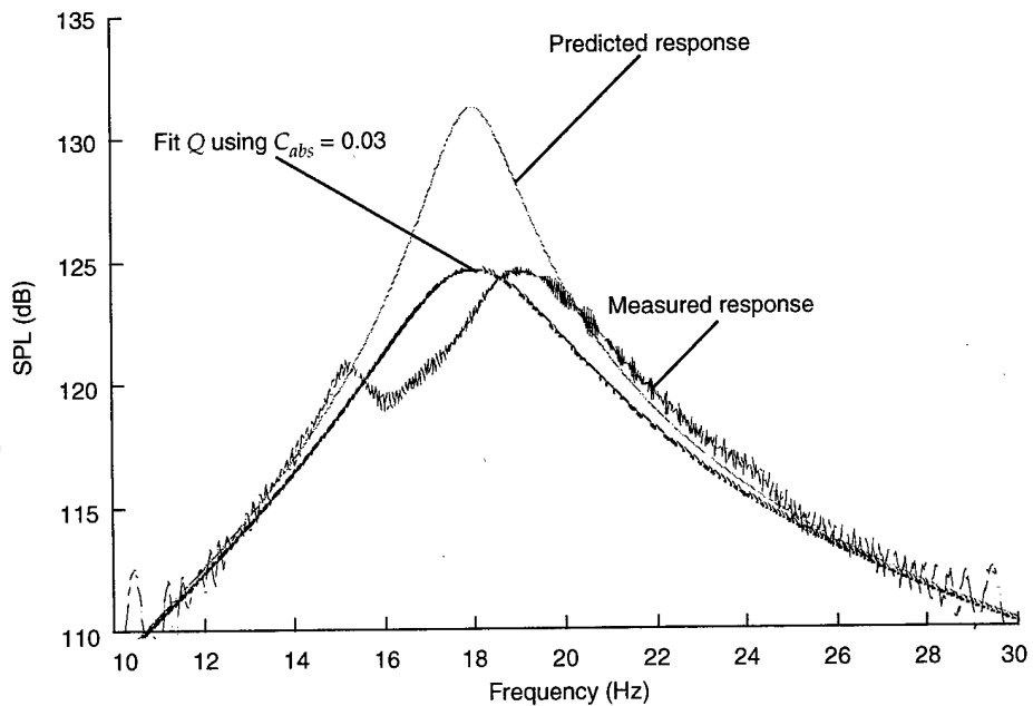
Figure 20. Measured and modeled response of chamber with 23-in.-diam, 4-in.-long port excited by JBL 18-in. loudspeaker. Jagged solid curve is measured response; smooth curves are model responses calculated with initial (upper curve) and modified (lower curve) chamber absorption.
