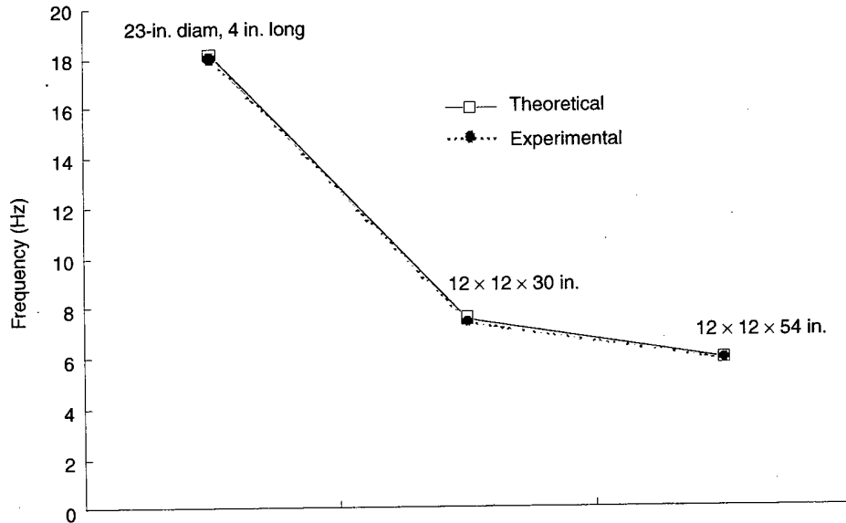
Figure 12. Comparison of predicted and measured natural resonant frequency of acoustic test chamber for various port configurations.
