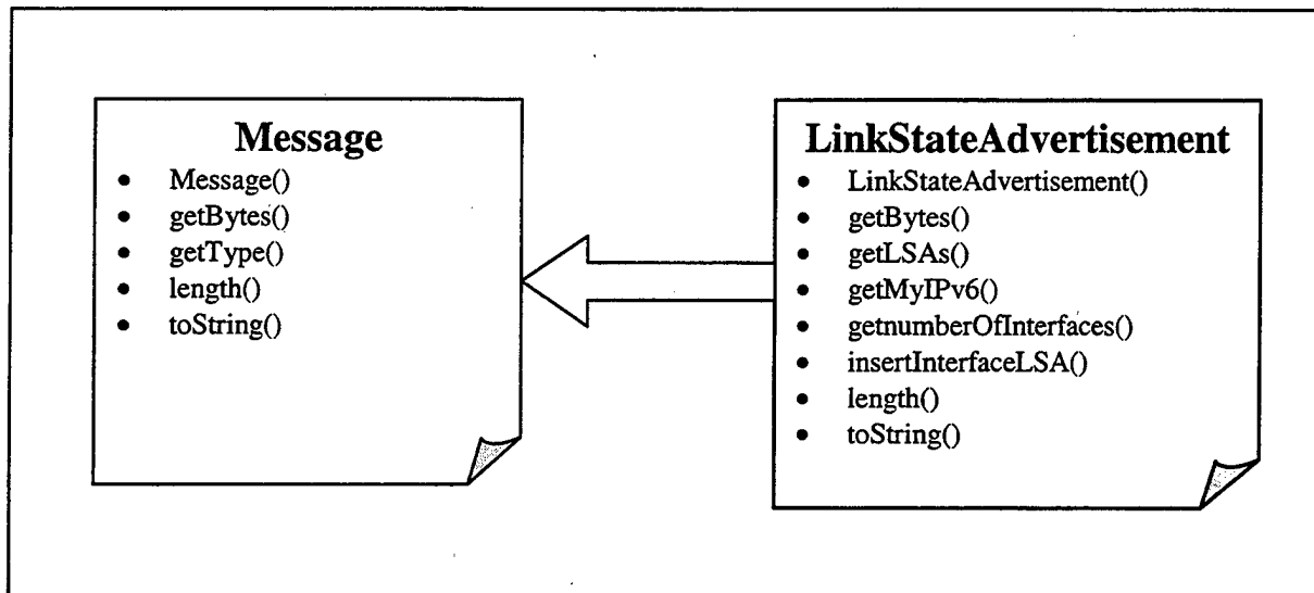
Figure 4. 5. saam.message.LinkStateAdvertisement
