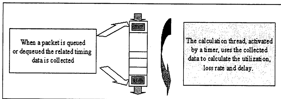
Figure 3. 6. Forming SLP-SA.
