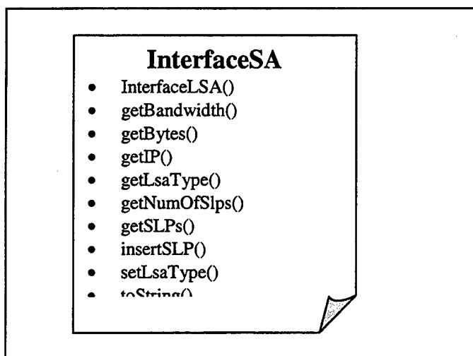
Figure 4. 3. saam.message.InterfaceSA
