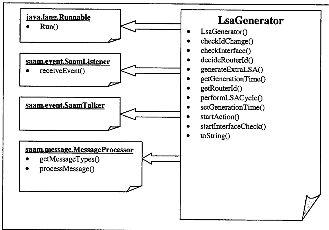
Figure 4. 6. saam.residentagent.router.LsaGenerator
