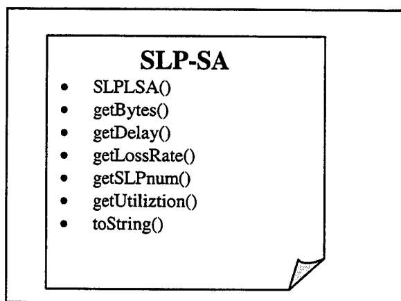
Figure 4. 2. saam.message.SLP-SA
