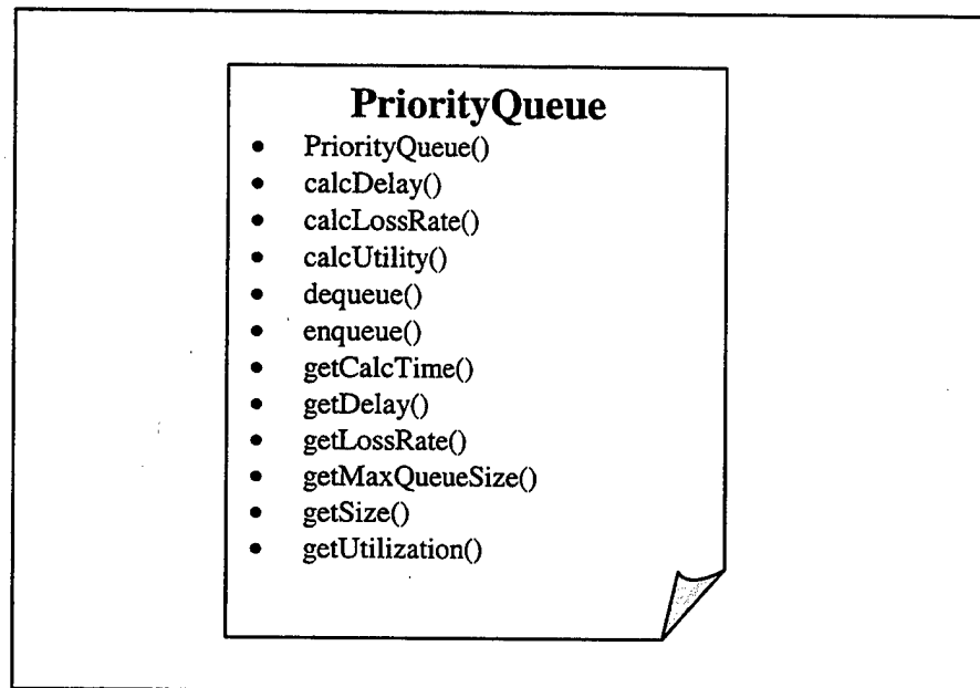
Figure 4. 1. saam.util.PriorityQueue
