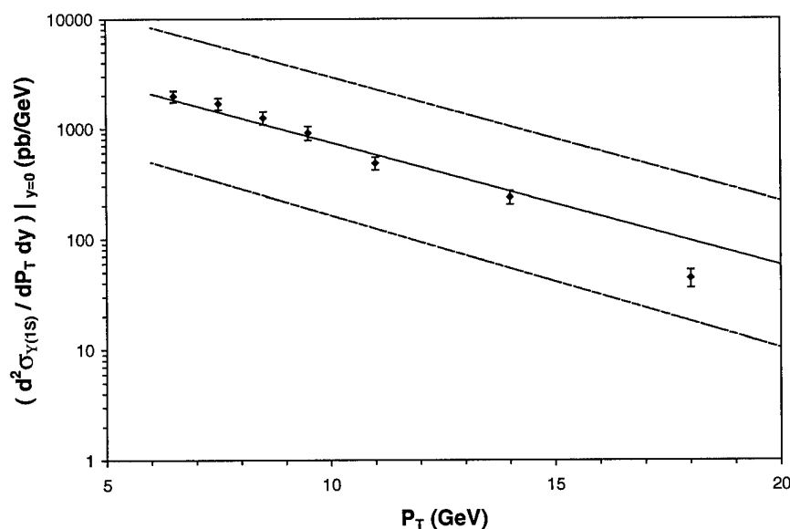
Figure 4.2: Plot of (d^2\sigma_{Y(1S)}/dP_T dy)|_{y=0} vs. P_T . The data points represent experimental measurements from Reference [22]. The lines are the theoretical predictions of the Color Evaporation Model.
