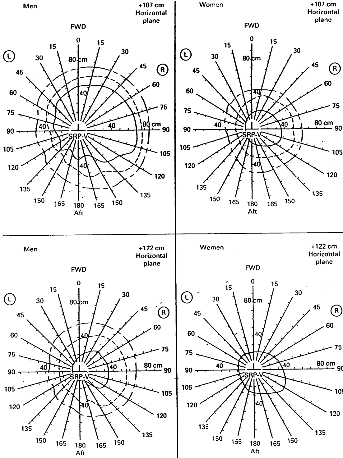
Figure 1-5(d). Reach contours in planes 107 and 122 cm above seat (SRP) height.
