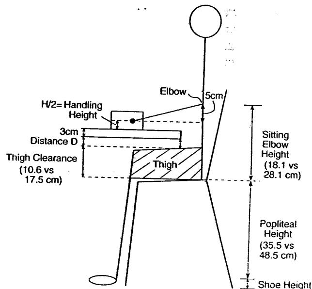
Figure 6.5 Calculation of product height. In the calculations assume that D=0 . The numbers given in parentheses are the 5th and 95th female percentiles
