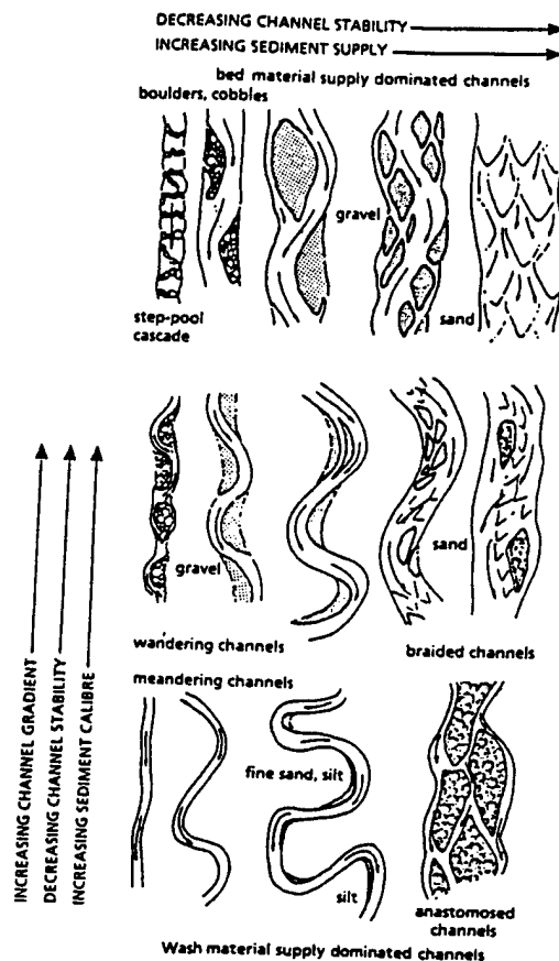
Fig. 4. Morphological types of large channels (reproduced with permission from M. Church (1992) Channel morphology and typology. Rivers handbook , Vol. 1 (ed. by P. Calow and G. E. Petts), p. 136. Blackwell Scientific, Oxford. The diagram is based on concepts from Schumm, S.A. (1985) Patterns of alluvial rivers. Ann. Rev. Earth Planetary Sci. 13, 5–72, with permission from Annual Reviews Inc., and Mollard, J.D. (1973) Air photo interpretation of fluvial features. Proceedings of the 7th Canadian Hydrology Symposium , pp. 341–380).
