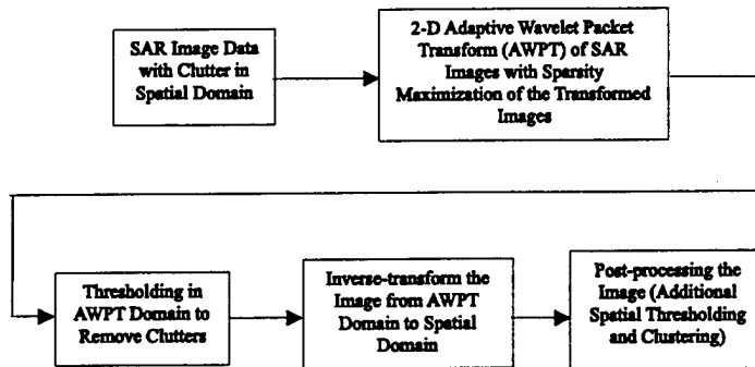
Figure 3. The processing scheme of automatic SAR clutter reduction based on Adaptive Wavelet Packet Transform (AWPT).
