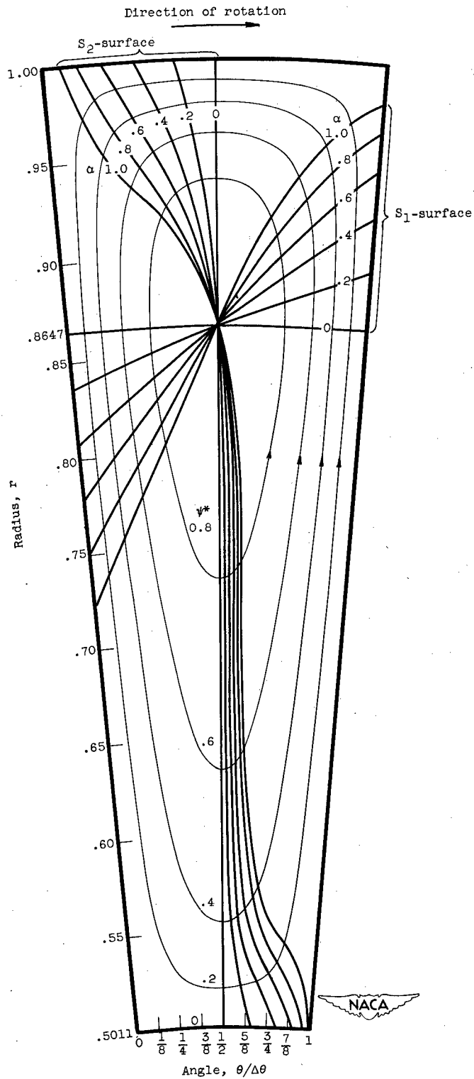
Figure 7. - Fluid-line positions of central S 1 - and S 2 -surfaces for example IV. Hub-tip ratio, r h , 0.50105; blade spacing, Δθ, 10°13'; minimum value of ψ, -0.00544.
