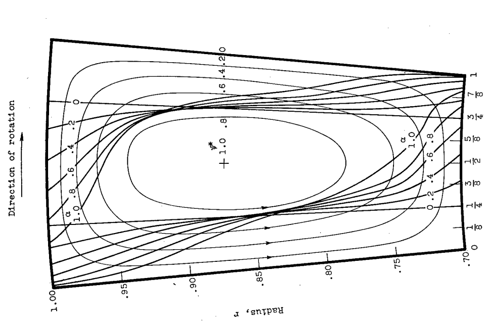
(d) Distortion of central S 1 -surface for wide range of \alpha .
