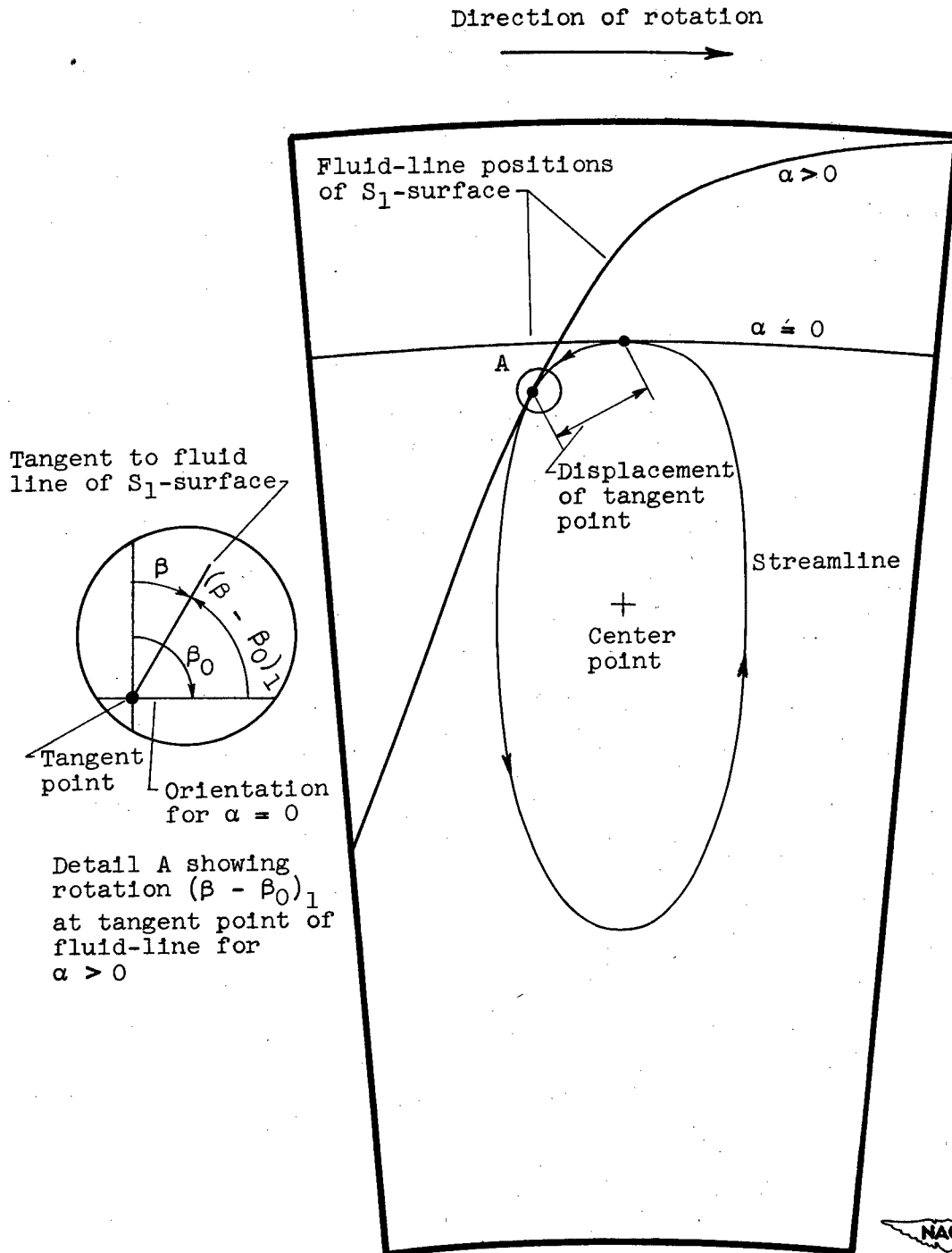
Figure 9. - Definitions of terms used to describe deviation of flow surfaces from initial orientation in r\theta -plane at \alpha = 1.0 .
