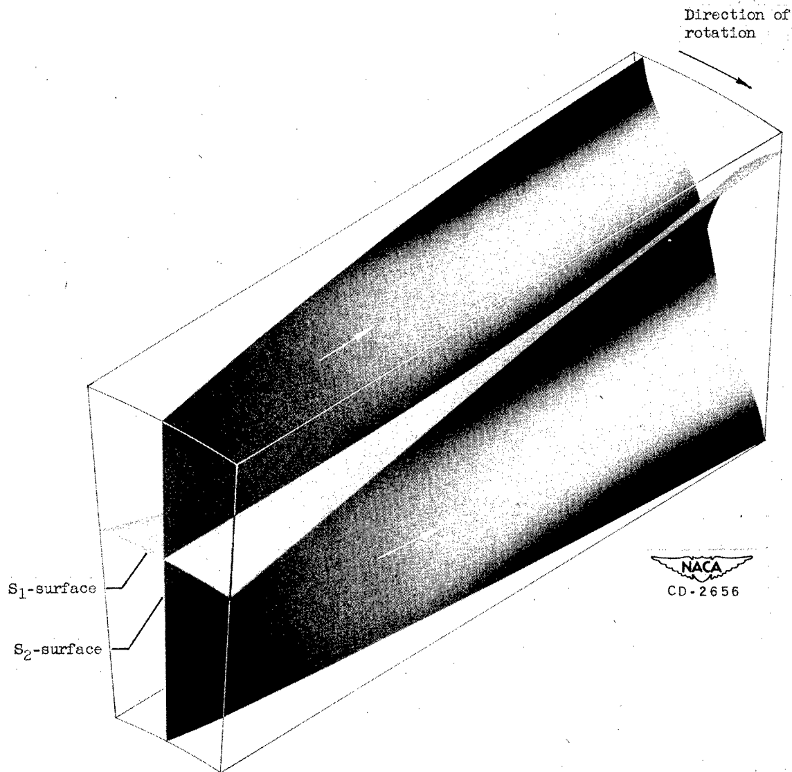
Figure 3. - Central S_1 - and S_2 -surfaces for example I with axial velocity w equal to 0.6.
