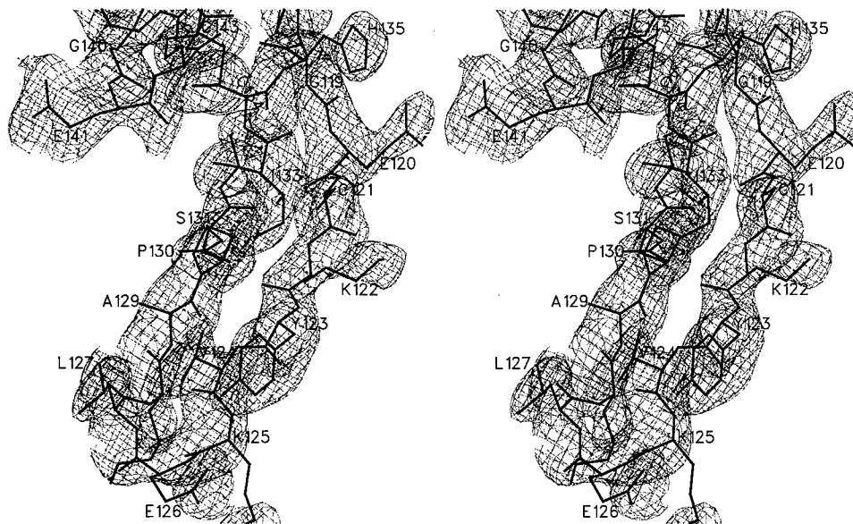
Figure 7. Representative Electron Density from a Simulated-Annealing F_o - F_c Omit Map Contoured at 1.6 \sigma . All atoms of HBEGF were omitted in the calculation of structure factors F_c . The region shown is the major \beta hairpin of HBEGF.
