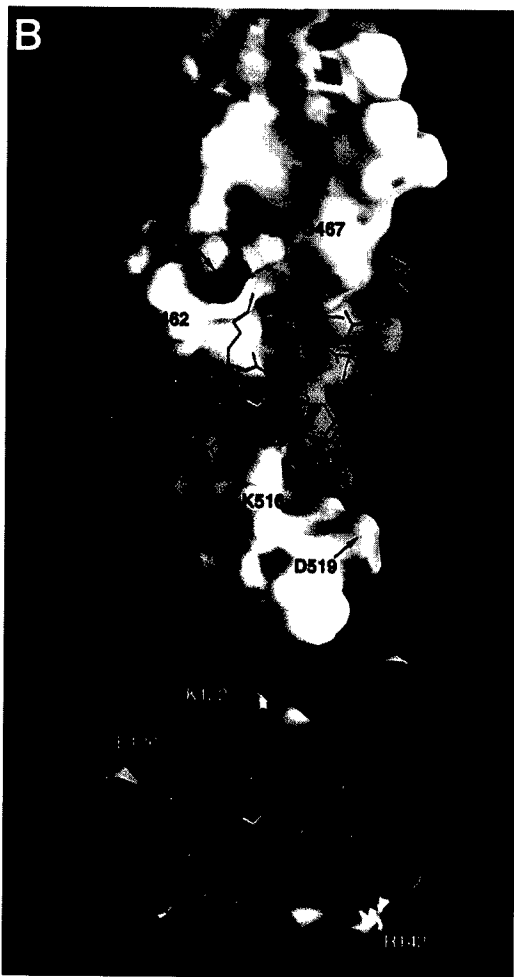
Figure 3. The Interaction between DT's R Domain and HBEGF (A) Interactions between DT's R domain and HBEGF. The polypeptide-chain backbones of the two molecules are represented as tubes (for clarity, partially transparent for HBEGF), and colored according to the scheme of Figure 2A. Nonpolar side chains at the interface are drawn in orange (DT) and brown-orange (HBEGF); polar side chains are drawn in blue (DT, darker; HBEGF, lighter). Direct intermolecular hydrogen-bond or salt-bridge interactions are shown as dark-blue dotted lines. Six water molecules that form bridging interactions between DT and HBEGF are also drawn as dark blue spheres. Amino acid residue labels use the one-letter abbreviation and are italicized and underlined for HBEGF. (B) Complementarity of interacting surfaces between DT's R domain (top) and HBEGF (bottom). Electrostatic potentials (positive, blue; negative, red) were calculated assuming a salt concentration of 0.15
