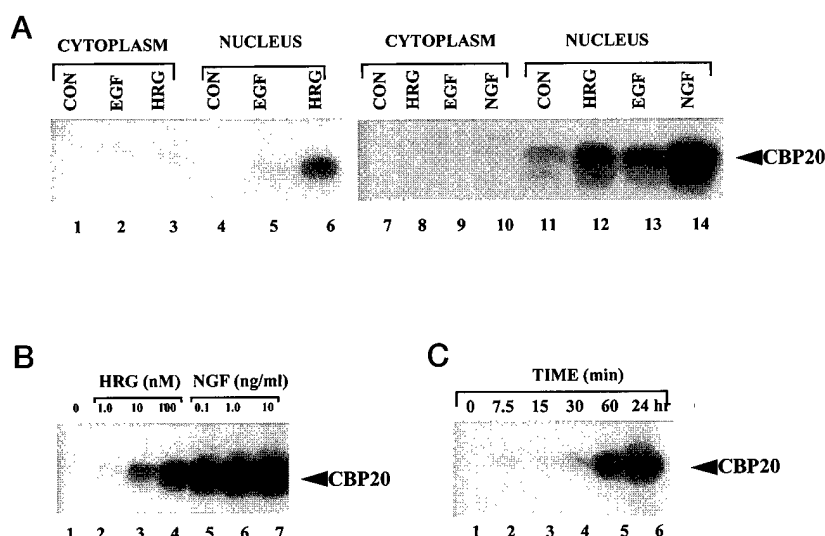
FIG. 4. Characterization of the growth factor-induced capped RNA-binding activity of the CBC (assayed by CBP20 [\alpha\text{-}^{32}\text{P}]\text{GTP} incorporation). A, HeLa cells (lanes 1–6) were serum-starved (control (CON); lanes 1 and 4) and then treated with 100 ng/ml EGF (lanes 2 and 5) or 30 nM heregulin (HRG; lanes 3 and 6) for 15 min at 37 °C. PC12 cells (lanes 7–14) were serum-starved (control; lanes 7 and 11) and then treated with 30 nM HRG (lanes 8 and 12), 100 ng/ml EGF (lanes 9 and 13), or 100 ng/ml NGF (lanes 10 and 14). The cells were lysed, separated into cytoplasmic (lanes 1–3 and 7–10) and whole nuclear (lanes 4–6 and 11–14) fractions, and assayed for [\alpha\text{-}^{32}\text{P}]\text{GTP} incorporation into CBP20 using 45 \mu\text{g} of protein from cell lysates. B, a dose-response experiment was performed with the addition of either heregulin (lanes 2–4) or NGF (lanes 5–7) to serum-starved PC12 cells (control; lane 1) for 30 min at 37 °C. For each dose of heregulin or NGF, 50 \mu\text{g} of total nuclear lysate protein were assayed for the incorporation of [\alpha\text{-}^{32}\text{P}]\text{GTP} into CBP20, and then 15% SDS-PAGE was performed. The resulting gel was dried and exposed to x-ray film for 5–15 h. C, a time course of 100 ng/ml NGF treatment was performed in serum-starved PC12 cells (control; lane 1) with NGF addition for 7.5 min (lane 2), 15 min (lane 3), 30 min (lane 4), 60 min (lane 5), or 24 h (lane 6). 50 \mu\text{g} of protein from the nuclear lysates were assayed for incorporation of [\alpha\text{-}^{32}\text{P}]\text{GTP} into CBP20, followed by 15% SDS-PAGE and autoradiography overnight.
