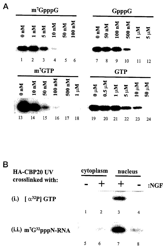
FIG. 3. Incorporation of [ \alpha - ^{32} P]GTP into CBP20 reflects an m 7 GpppN-capped RNA binding event by the CBC that can be growth factor-regulated. A, [ \alpha - ^{32} P]GTP incorporation into PC12 cell CBP20 is blocked by the addition of RNA cap analogs. Nuclear extracts were prepared from PC12 cells growing asynchronously in culture. 200 \mu g of lysate were then immunoprecipitated with 5 \mu l of \alpha CBP80 antiserum. The immunoprecipitates were assayed for [ \alpha - ^{32} P]GTP incorporation into CBP20 in the presence of m 7 GpppG (0, 1, 5, 10, 50, and 100 nM (lanes 1–6, respectively)), GpppG (0 nM, 50 nM, 100 nM, 500 nM, 1 \mu M, and 5 \mu M (lanes 7–12, respectively)), m 7 GTP (0 nM, 10 nM, 50 nM, 100 nM, 500 nM, and 1 \mu M (lanes 13–18, respectively)), and GTP (0, 0.5, 1, 5, 10, and 50 \mu M (lanes 19–24, respectively)). Following cross-linking, proteins were separated by 15% SDS-PAGE; the gel was dried; and autoradiography was performed. B, CBP20 binds capped RNA in a growth factor-dependent manner. PC12 cells stably expressing HA-CBP20 were serum-starved (–) and then treated with 100 ng/ml NGF for 1 h (+). After preparation of cytosolic and nuclear lysates, HA-CBP20 was immunoprecipitated from the lysates and assayed in the presence of either [ \alpha - ^{32} P]GTP (lanes 1–4) or m 7 G 32 pppN-capped RNA (lanes 5–8).
