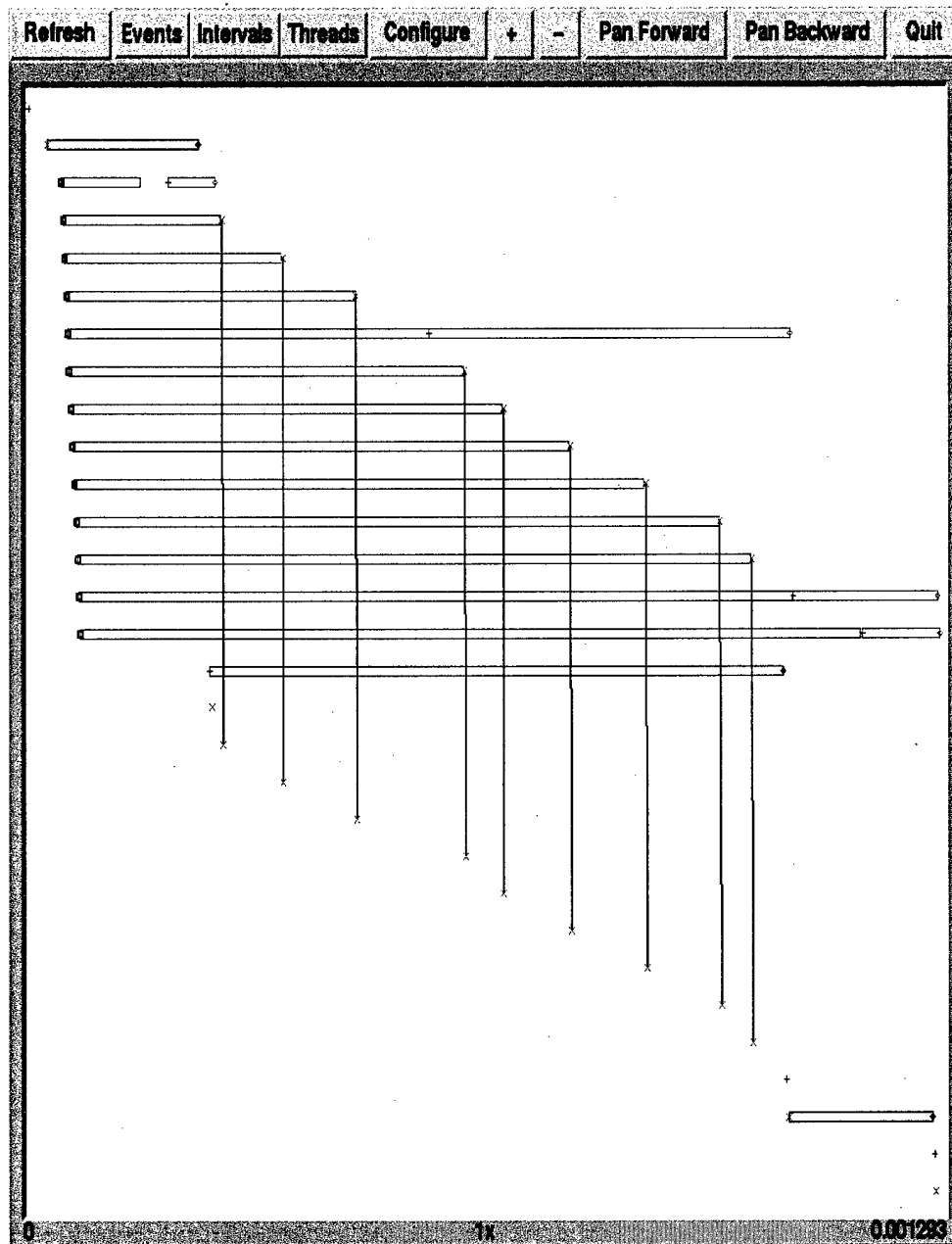
Figure 15. NoWaitSmallTimer interval is represented by the vertical line connection between the symbol x in the car thread and symbol x in the SmallTimer . There are 9 NoWaitSmallTimer intervals, originating from car 2, 3, 4, 6, 7, 8, 9, 10 and 11. These intervals represent the SmallTimer objects created by cars that did not have to stop at the intersection.
