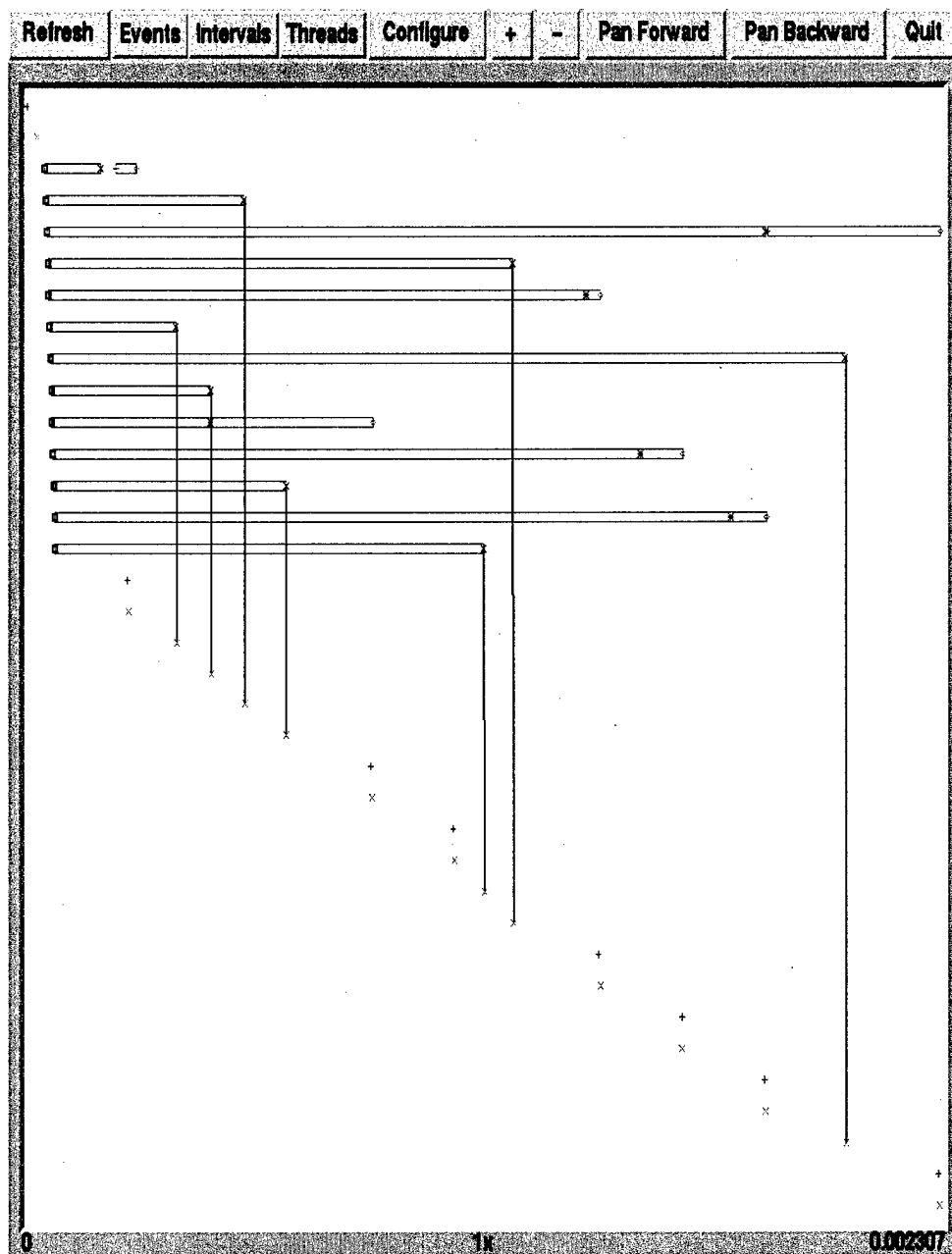
Figure 10. NoWaitSmallTimer interval is represented by the vertical line connection between the symbol x in the car thread and symbol x in the SmallTimer. There are 7 NoWaitSmallTimer intervals, originating from cars 2, 4, 6, 7, 8, 11, and 13. These intervals represent the new SmallTimer objects created by cars that did not have to stop at the intersection.
