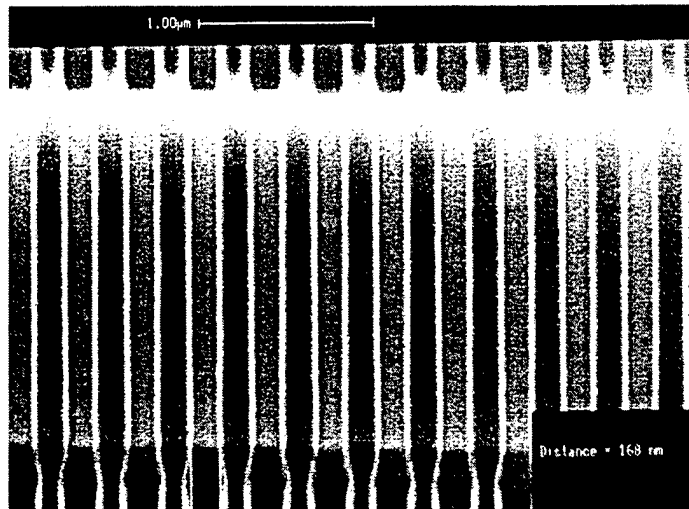
Figure 20. Grating etched into silicon dioxide.
