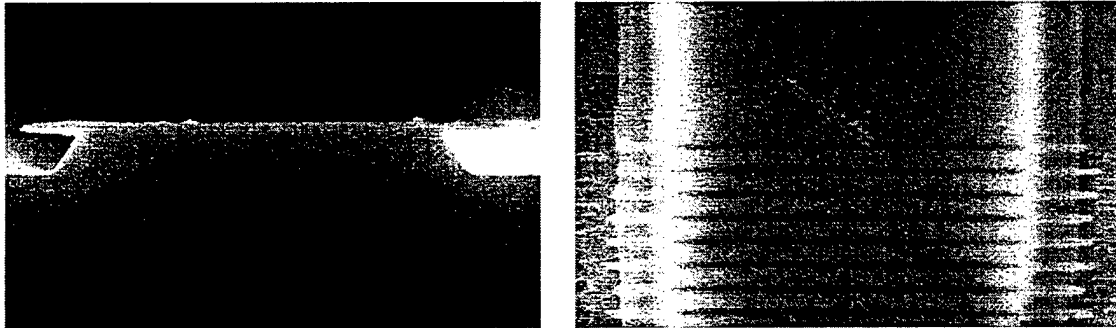
Figure 5 Distributed Bragg pulse shaper. Left: Entrance facet of waveguide. Right: Top view of waveguide and a section of Bragg grating. In both images the SiO 2 etch mask hangs over the etched waveguide.
