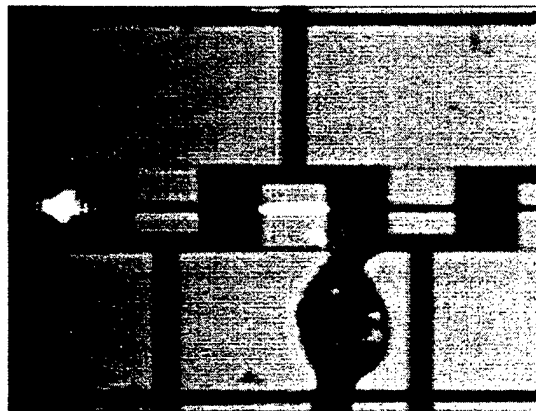
Figure 40. The distributed Bragg pulse shaper in operation. Light is injected into the facet at the left. Current in the grating section causes spontaneous emission.
