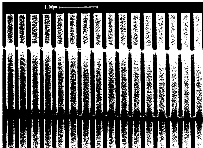
Figure 21. Grating etched into Al x Ga 1-x As, top view.
