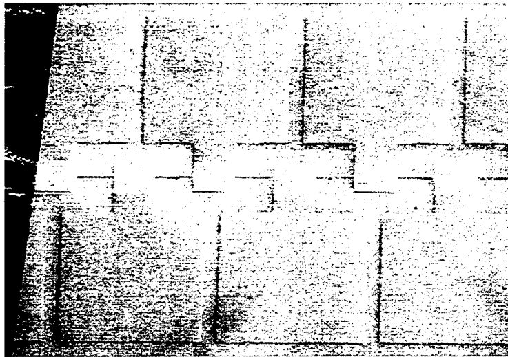
Figure 11 Distributed Bragg pulse shaper. The thin line is the waveguide, with large gold contacts covering the 50 µm grating sections of the waveguide.
