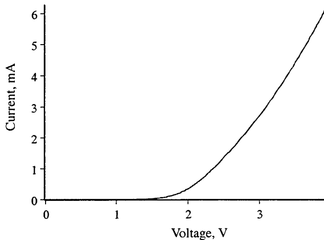
Figure 34. I-V curve for 14.1T1.H1, Device 8.
