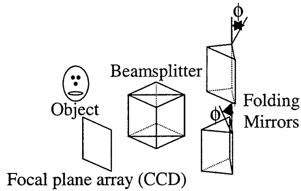
Figure 47. Rotational Shearing Interferometer
