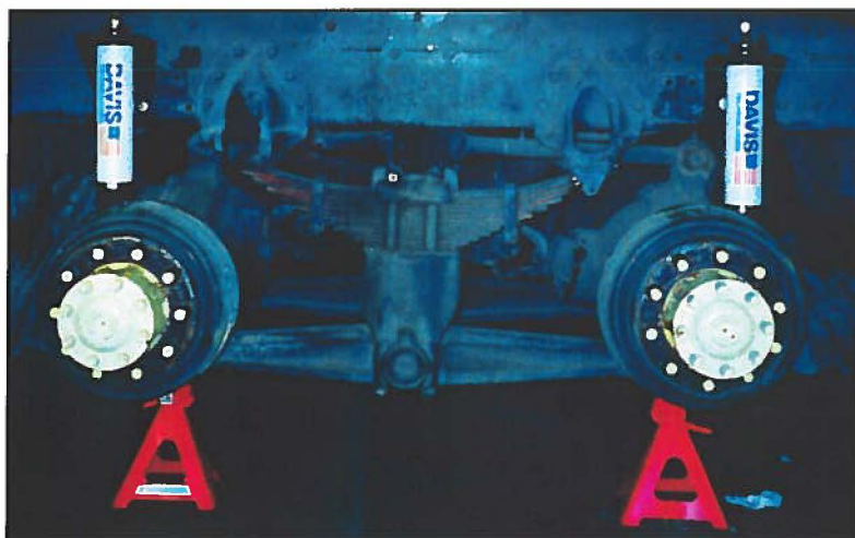
Figure 5. Installation of DTI Struts on Rear-Dual Axles
