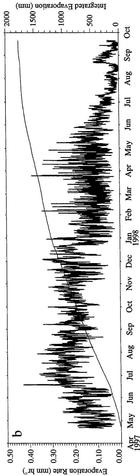
Figure 5-8. (a) Hourly averaged precipitation rate (black) and accumulated precipitation (gray) from IMET self-siphoning rain gauge. (b) Hourly averaged evaporation rate (black) and integrated evaporation (gray) from bulk formulae. (PACS South)
