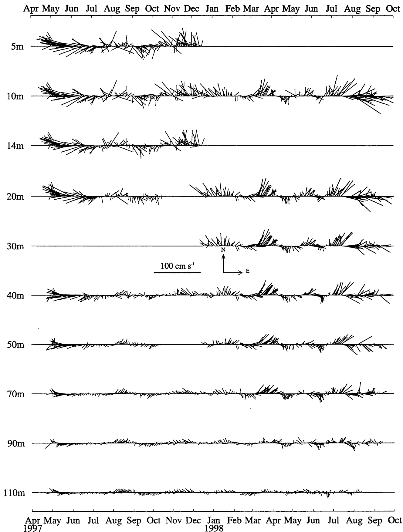
Figure 4-24. VMC 36 hour vector averaged velocity. (PACS North)
