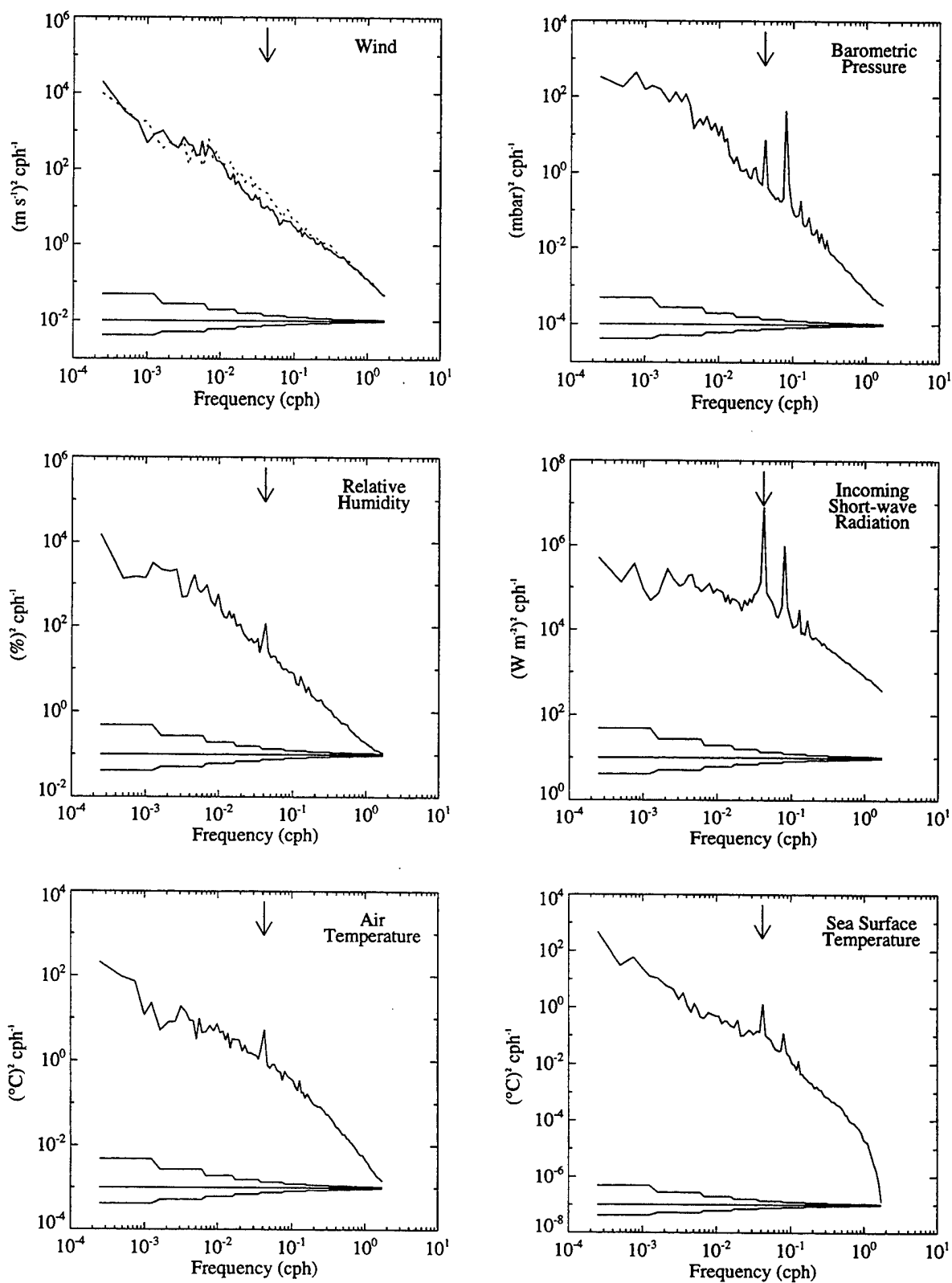
Figure 4-33. Autospectra of meteorological parameters. Rotary autospectra of the wind provides both clockwise (solid) and counter-clockwise (dotted) spectras. The arrow indicates the diurnal frequency ( 24^{-1} \text{ cph} ).
