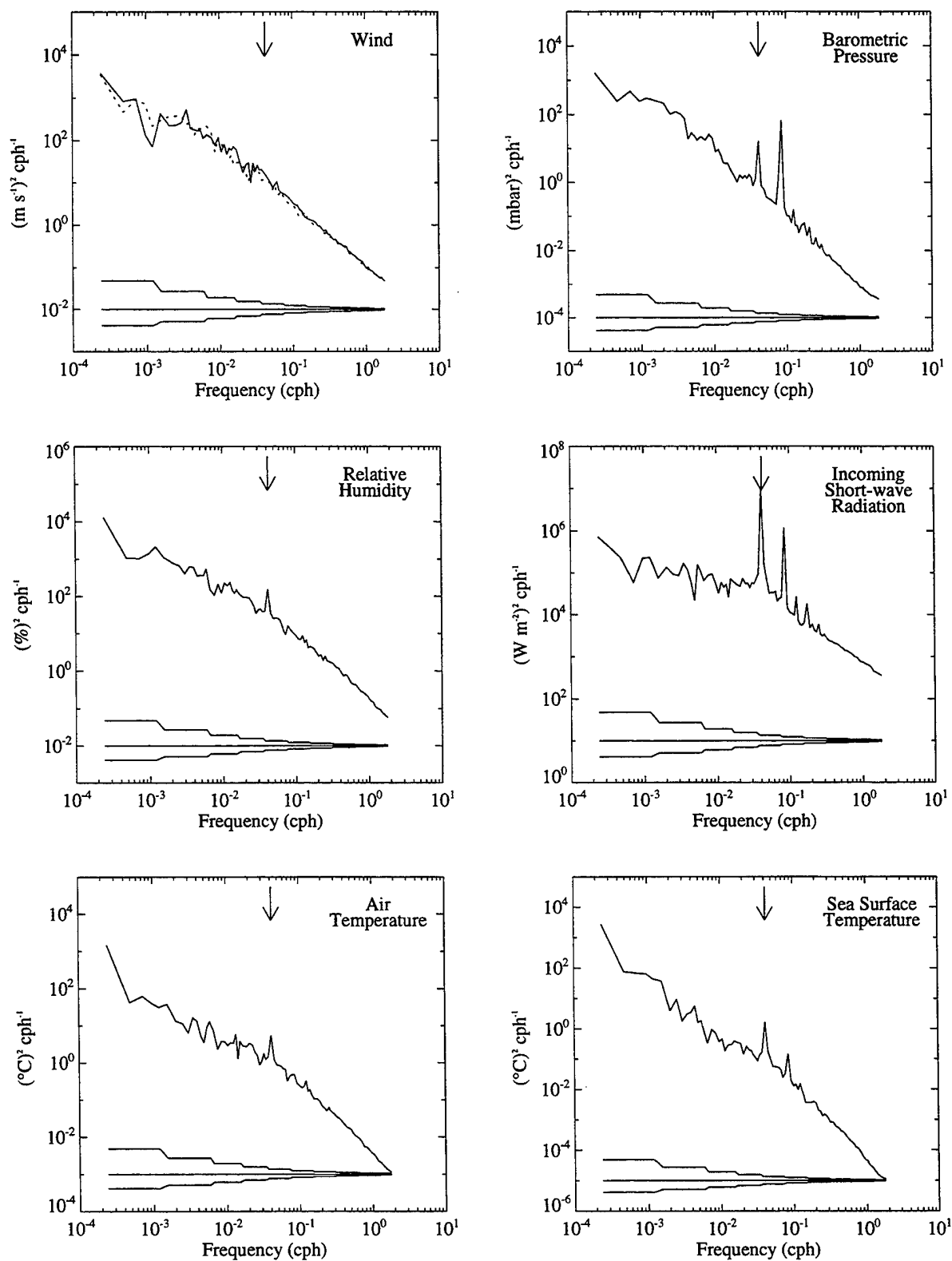
Figure 5-33. Autospectra of meteorological parameters. Rotary autospectra of the wind provides both clockwise (solid) and counter-clockwise (dotted) spectra. The arrow indicates the diurnal frequency ( 24^{-1} \text{ cph} ).
