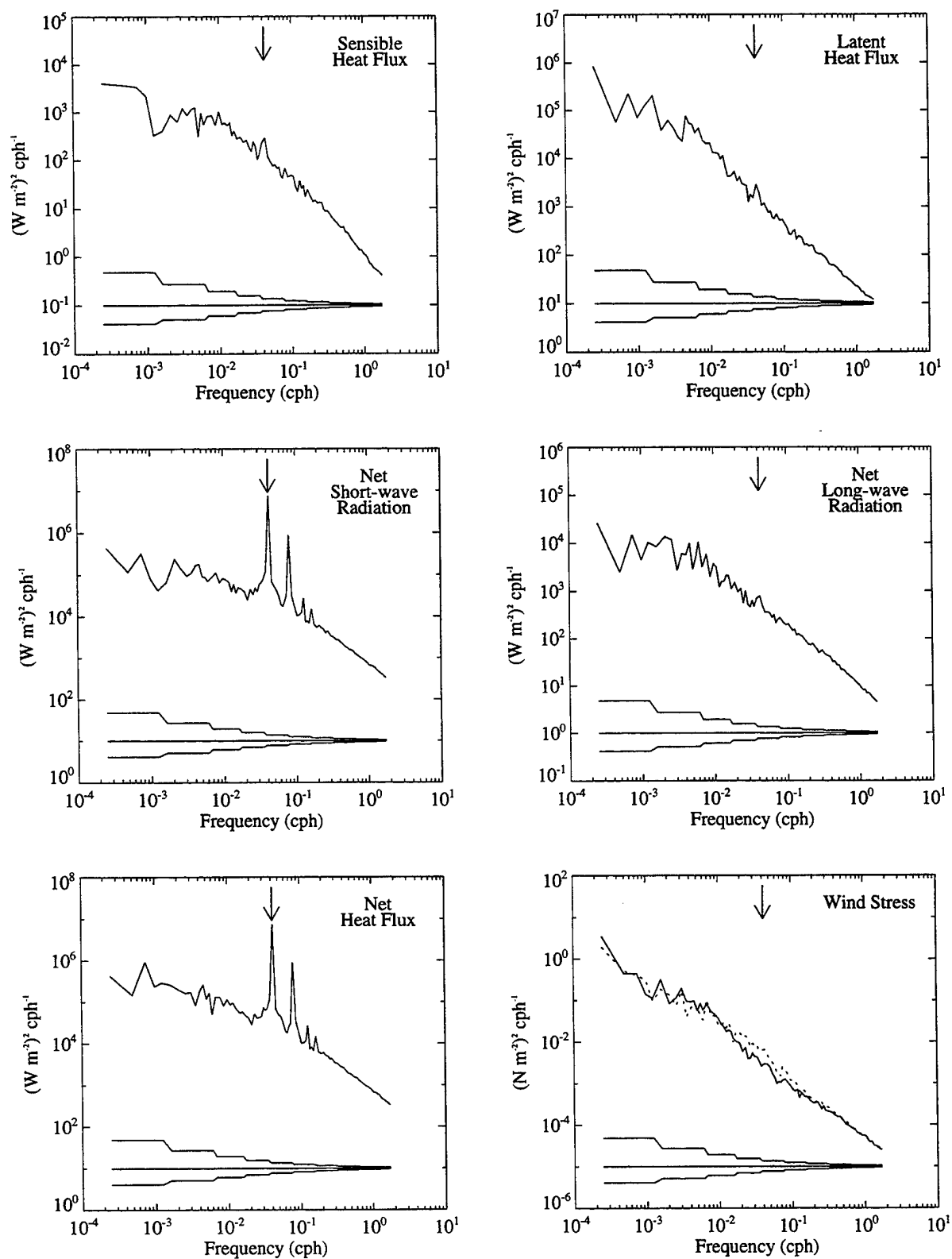
Figure 4-34. Autospectra of heat fluxes. Rotary autospectra of the wind stress provides both clockwise (solid) and counter-clockwise (dotted) spectras. The arrow indicates the diurnal frequency ( 24^{-1} cph).
