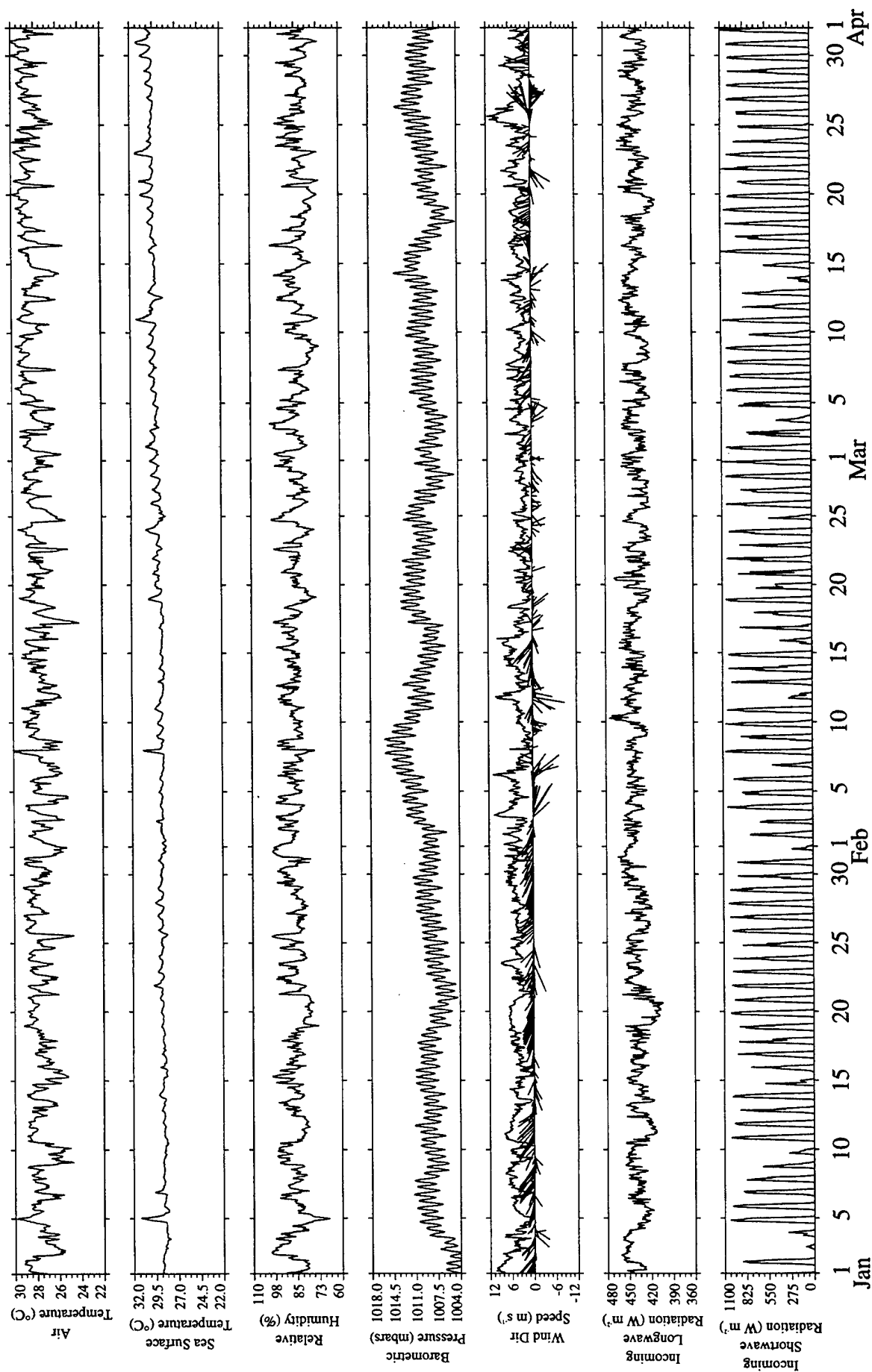
Figure 5-5. Hourly time series of meteorological observations for January through March 1998. (PACS South)
