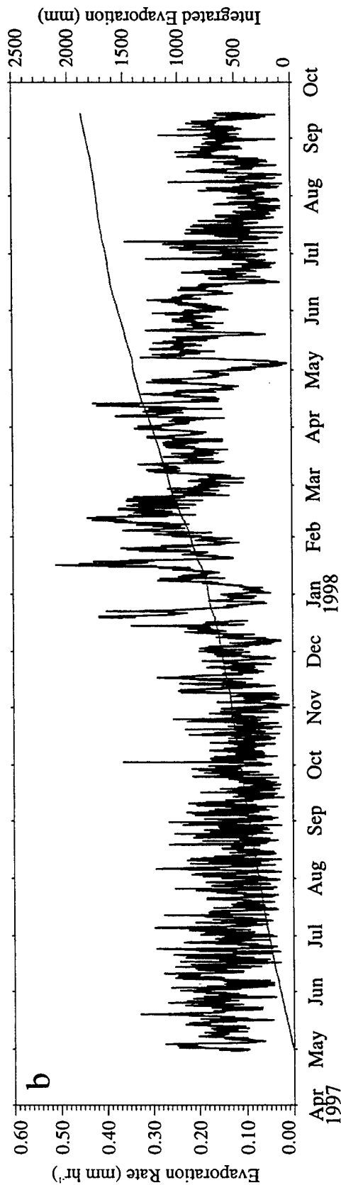
Figure 4-8. (a) Hourly averaged precipitation rate (black) and accumulated precipitation (gray) from IMET self-siphoning rain gauge. (b) Hourly averaged evaporation rate (black) and integrated evaporation (gray) from bulk formulae. (PACS North)
