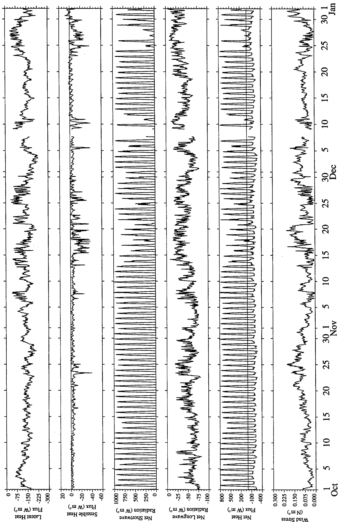
Figure 5-12. Hourly time series of estimated heat and momentum fluxes for October through December 1997. (PACS South)
