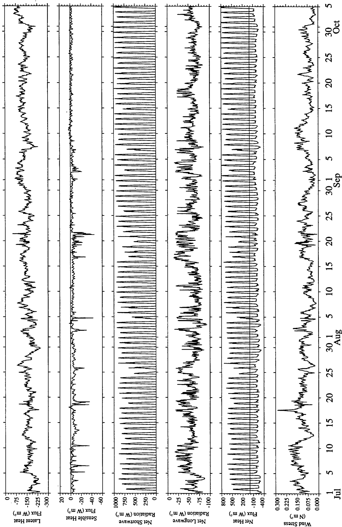
Figure 5-11. Hourly time series of estimated heat and momentum fluxes for July through September 1997. (PACS South)
