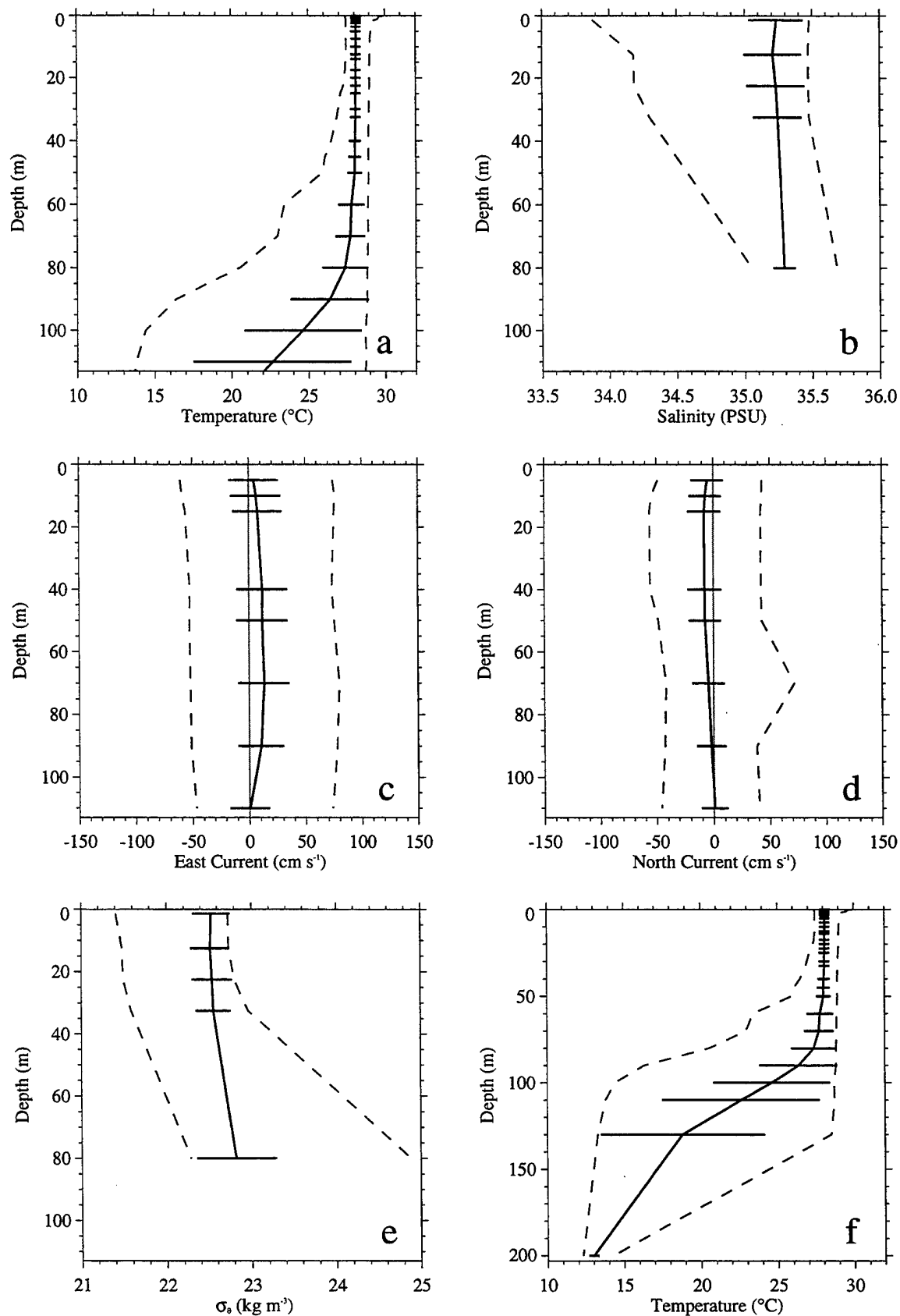
Figure 5-37. Mean profiles of April 1997 to December 1997 (horizontal bar indicates \pm standard deviation, dash line indicates maximum and minimum range). (PACS South)
