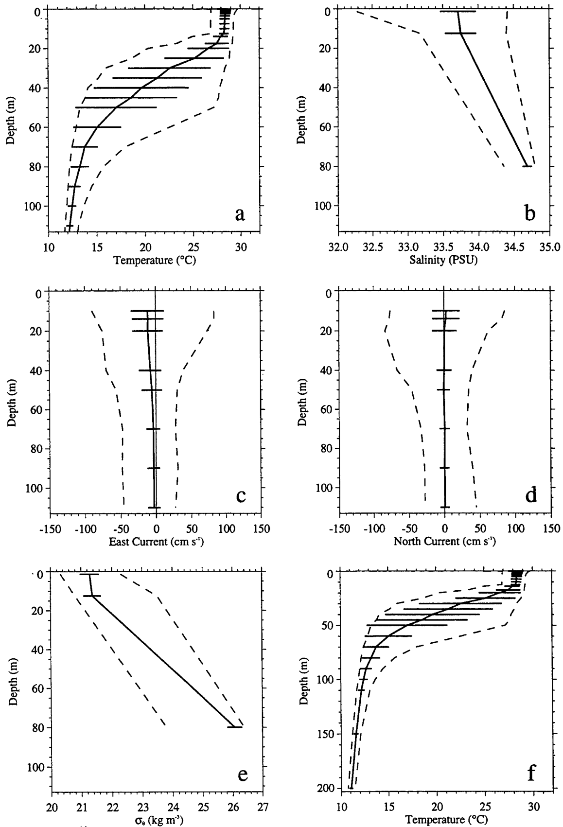
Figure 4-37. Mean profiles of April 1997 to December 1997 (horizontal bar indicates \pm standard deviation, dash line indicates maximum and minimum range). (PACS North)
