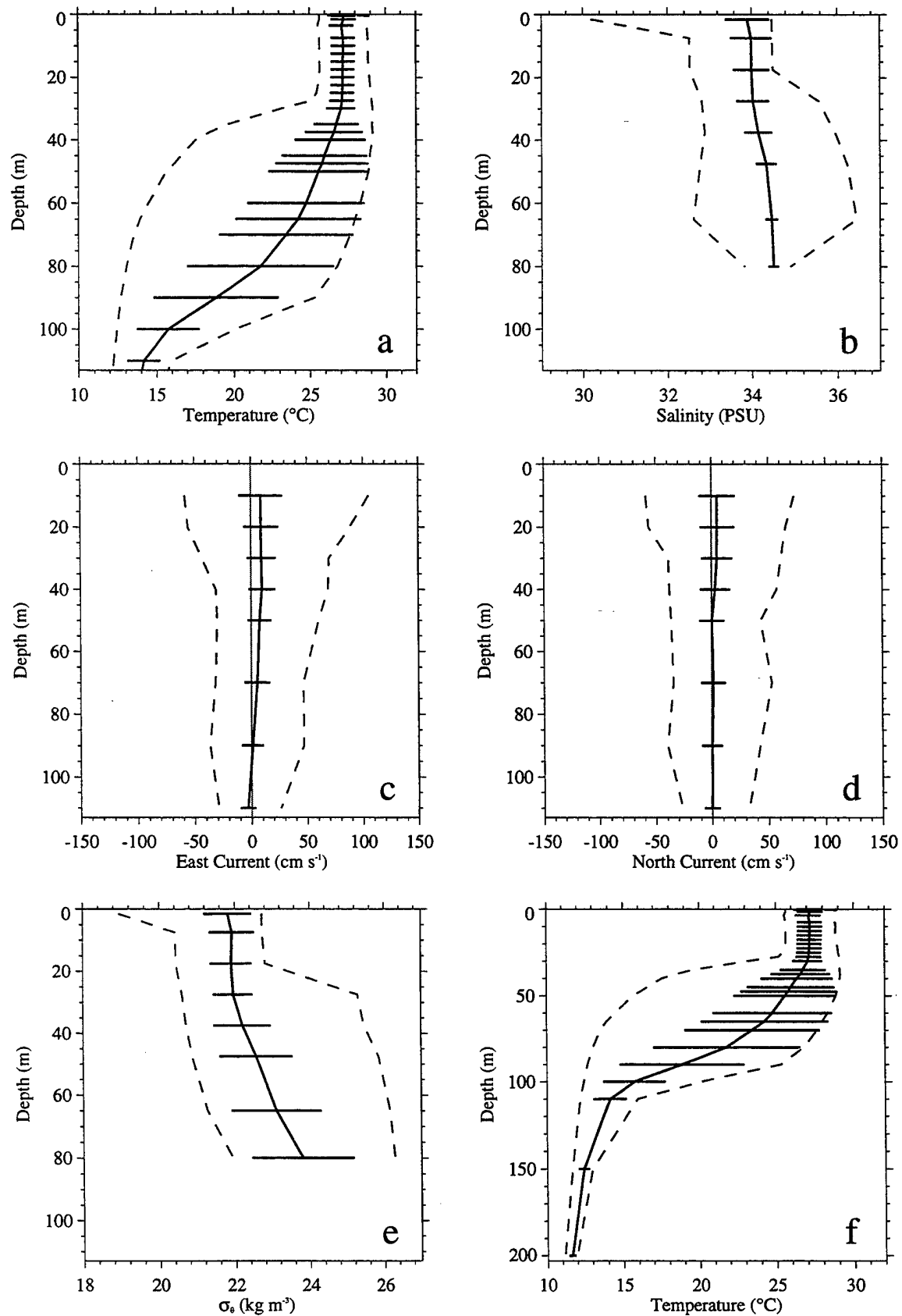
Figure 4-38. Mean profiles of December 1997 to September 1998 (horizontal bar indicates \pm standard deviation, dash line indicates maximum and minimum range). (PACS North)
