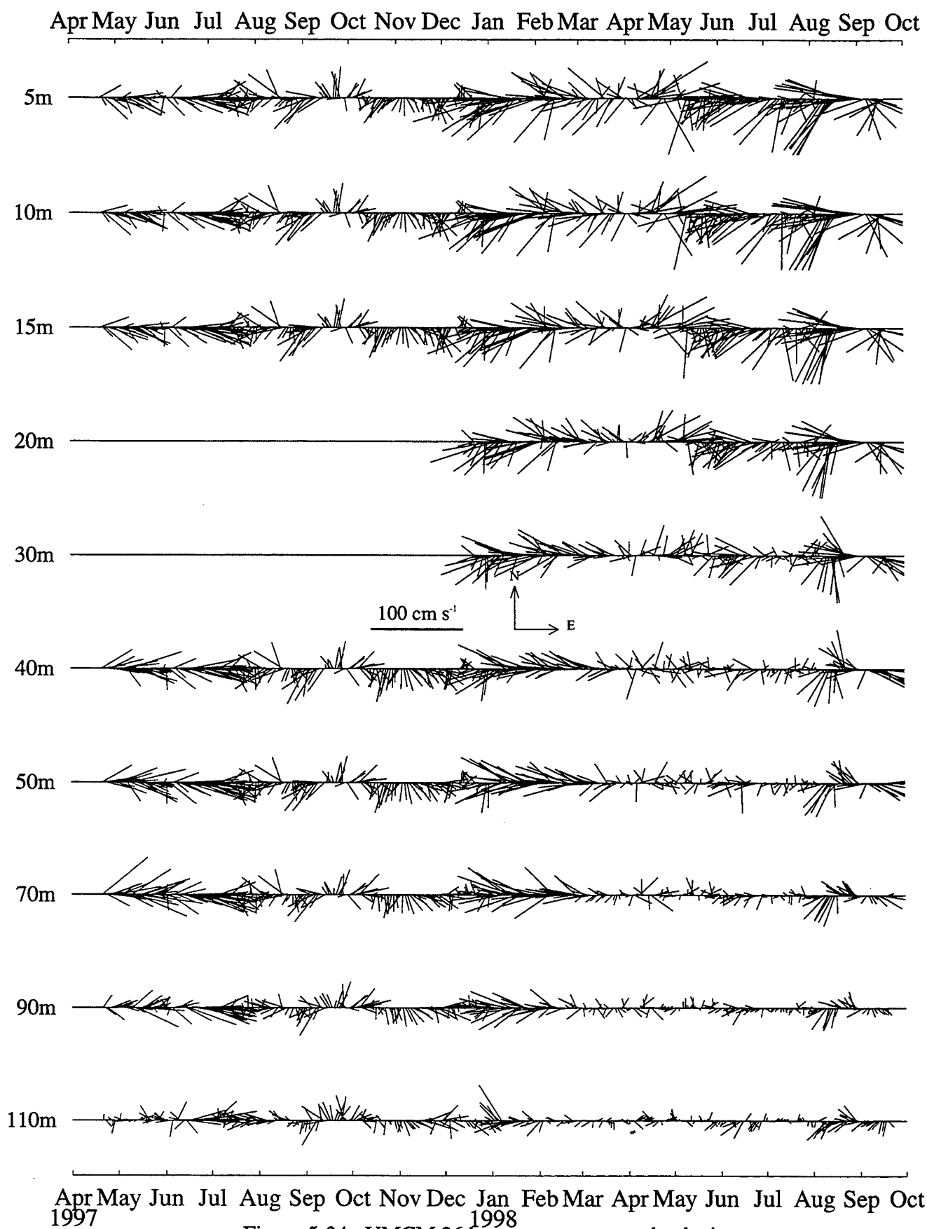
Figure 5-24. VMCM 36 hour vector averaged velocity. (PACS South)
