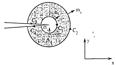
Fig. 1 A simply connected domain A_i enclosed by the contour C ( C = C_1 + C_2 + C_3 + C_4 ) near crack tip. The domain is where the domain integral is evaluated.
