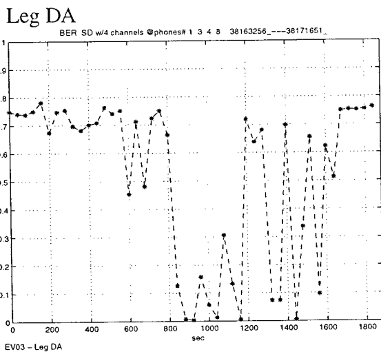
Figure 20: The BER of the equalized received signals (using spatial diversity) on channels 1, 3, 4, and 8 during event 03 and event 04.
