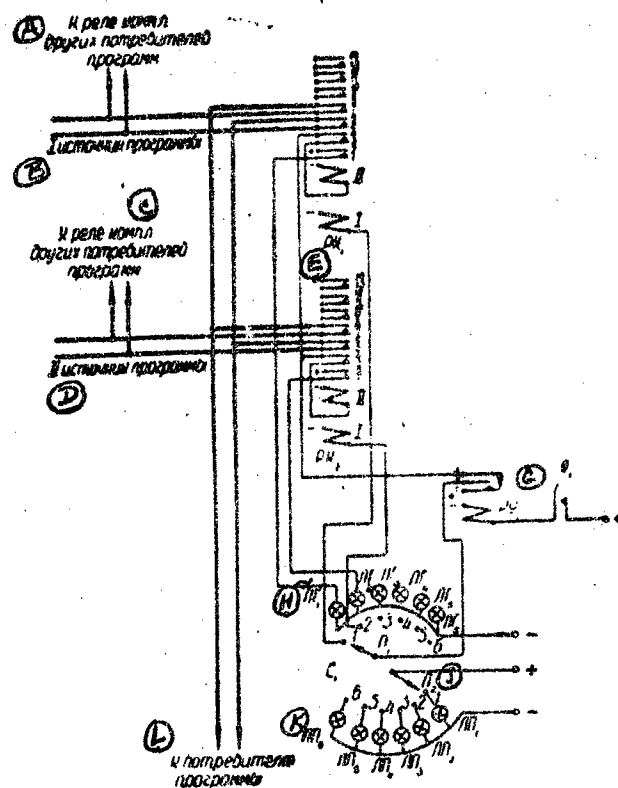
Figure. A) To relay units of other program-transmission facilities; B) program source I; C) to relay units of other program-transmission facilities; D) program source II; E) RK_1 ; F) PK_2 ; G) RU_1 ; H) LG ; I) P_1 ; J) P_2 ; K) LP ; L) to program-transmission facility,
