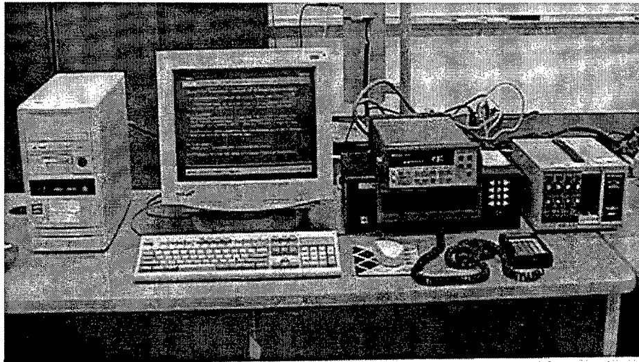
Figure 8. Experimental set-up, Computer, 855C Programmable Controller, Multimeter, Amplifier.
