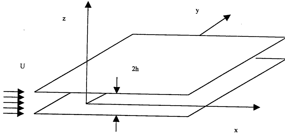
Figure 2. Hele-Shaw Cell.
