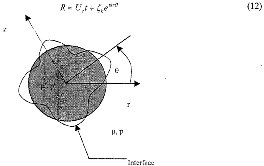
Figure 4. Plan View of Radial Hele-Shaw Cell.
