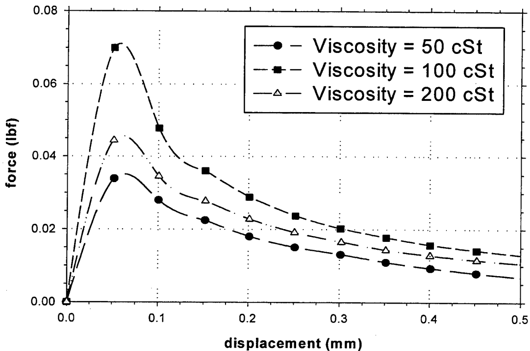
Figure 14. Force-Displacement plot that shows the effect of medium viscosity fluids on F_{\max} and d_{\max} . The Initial Liquid Layer Thickness ( l_0 ) is 50\mu\text{m} , and Separation Velocity ( V ) is 24\mu\text{m/s} .
