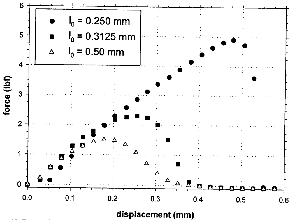
Figure 19. Force-Displacement plot that shows the effect of Initial Liquid Layer Thickness on F_{\max} and d_{\max} . Separation Velocity ( V ) is 4.5\mu\text{m/s} and Viscosity ( \nu ) is 100,000 cSt.
