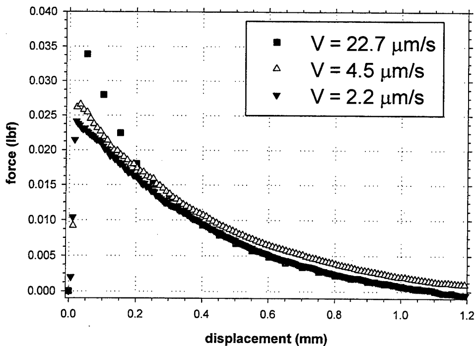
Figure 16. Force-Displacement plot that shows the effect of Separation Velocity on F_{\max} and d_{\max} . The Initial Liquid Layer Thickness ( l_0 ) is 50 \mu\text{m} and Viscosity ( \nu ) is 50 cSt.
