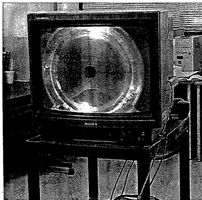
Figure 9. Experimental set-up showing monitor for bottom view.
