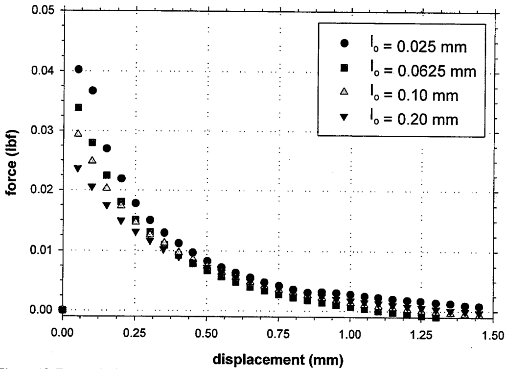
Figure 18. Force-Displacement plot that shows the effect of Initial Liquid Layer Thickness on F_{max} and d_{max} . Separation Velocity ( V ) is 24\mu\text{m/s} and Viscosity ( \nu ) is 50 cSt.
