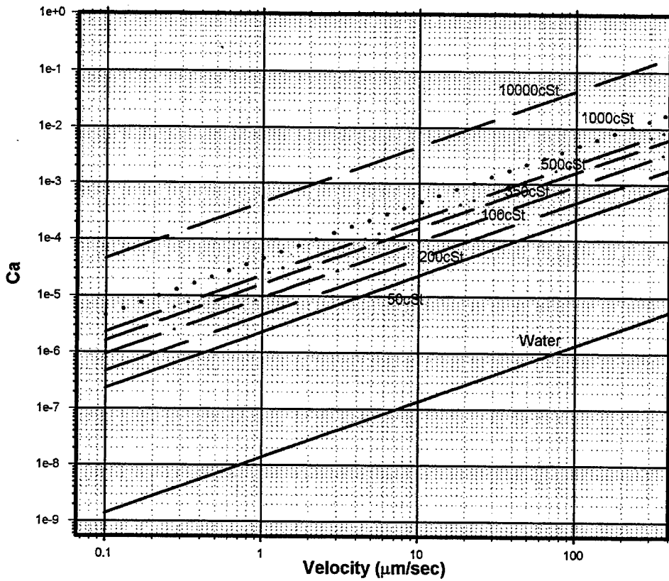
Figure 12. Capillary number vs. Velocity plot.
