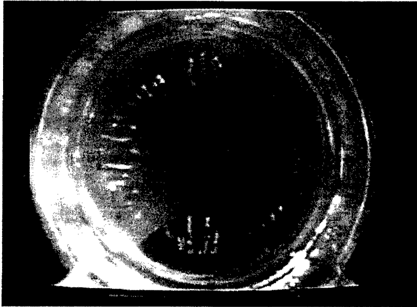
Figure 22. 10,000 cSt Silicone Oil, Initial Liquid Layer Thickness of 312.5\mu\text{m} and Separation Velocity of 12\mu\text{m/s} (Scale of 1div=1mm), N\approx 47 .
