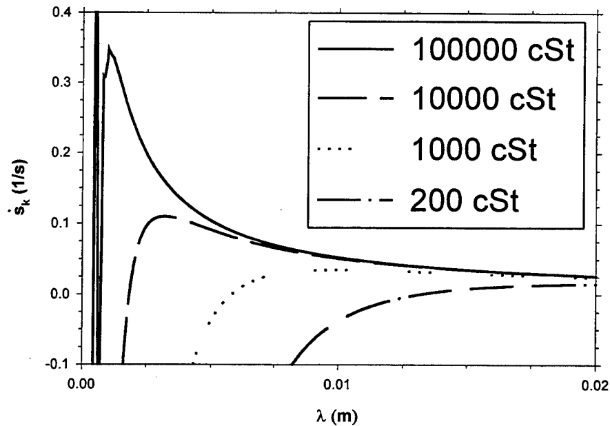
Figure 5. Growth Rate vs Wavelength (Radial velocity and Displacement Constant).
