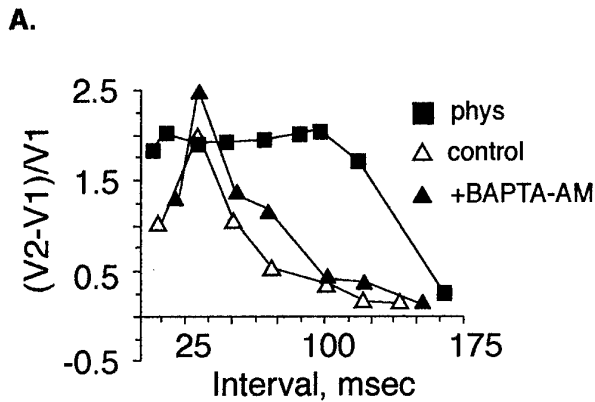
Fig. 4-3. Physiological and transcriptional responses both depend on intracellular Ca^{++} accumulation and Na^+ influx.
