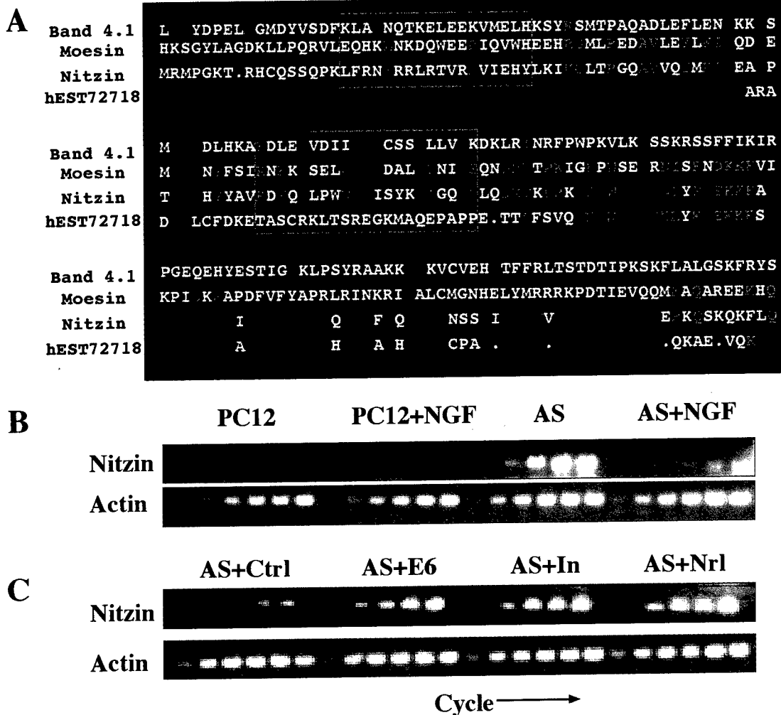
FIG. 4. Expression of nitzin, a band 4.1 protein family member, is associated with AS-ACHE neuritogenesis. (A) Sequence alignment. Partial amino acid sequences from mouse band 4.1, human moesin, rat nitzin, and the corresponding human expressed sequence tag homolog to nitzin. Band 4.1 family consensus sequences are marked in red, ERM consensus sequences in blue, and nitzin/expressed sequence tag homologous residues in green. Band 4.1 signature no. 2 in sequence blocks 3 and 4 are marked by red brackets, and ERM family motifs IV and V are enclosed in blue boxes. (B) Transcriptional modulations. Nitzin mRNA levels were evaluated by RT-PCR in naive and NGF-differentiated PC12 and AS-ACHE cells, and in AS-ACHE cells transfected with a control plasmid (AS + ctrl), or plasmids encoding AChE-E6 (AS + E6), catalytically inactivated AChE (AS + In) or neuroigin-1 (AS + Nrl) as in Fig. 3. Samples were removed as described in the Fig. 3 legend. Note the pronounced expression of nitzin in AS-ACHE but not PC12 cells, its suppression under NGF, and the neuritogenic-associated increases in rescued AS-ACHE cells, under conditions in which actin mRNA levels remained unchanged.
