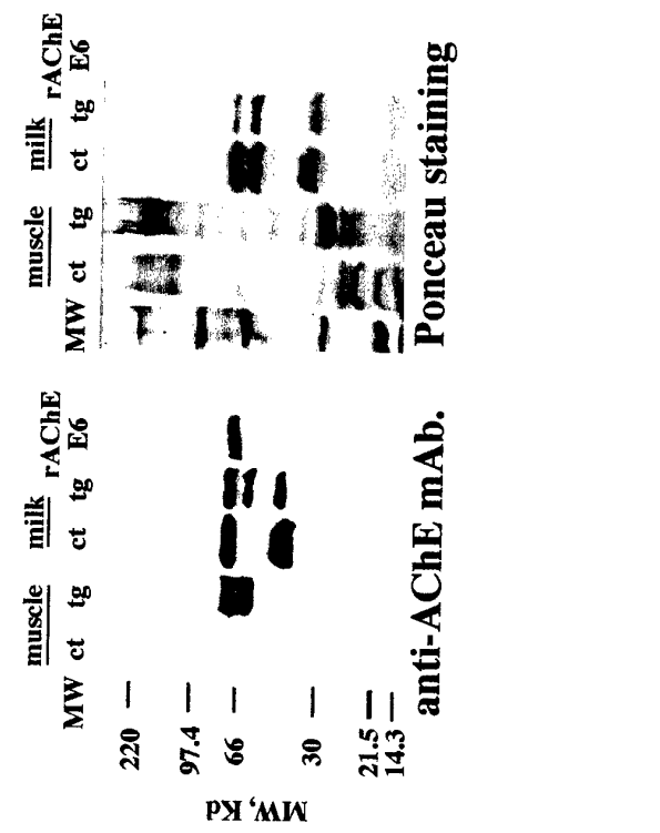
Fig. 7-4. Immunodetection of recombinant human AChE in milk and muscle of transgenic mice
