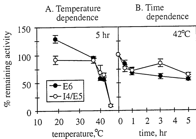
Fig. 6-3. Heat stability of the recombinant AChE variants
