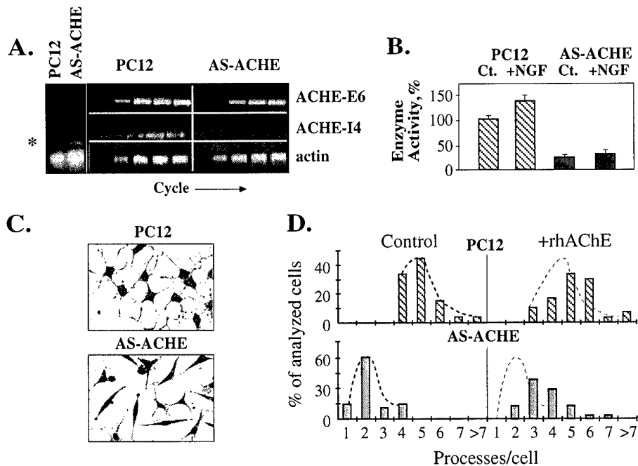
Fig. 3-1. AChE suppression is associated with a partially rescuable neurotogenic deficiency.
