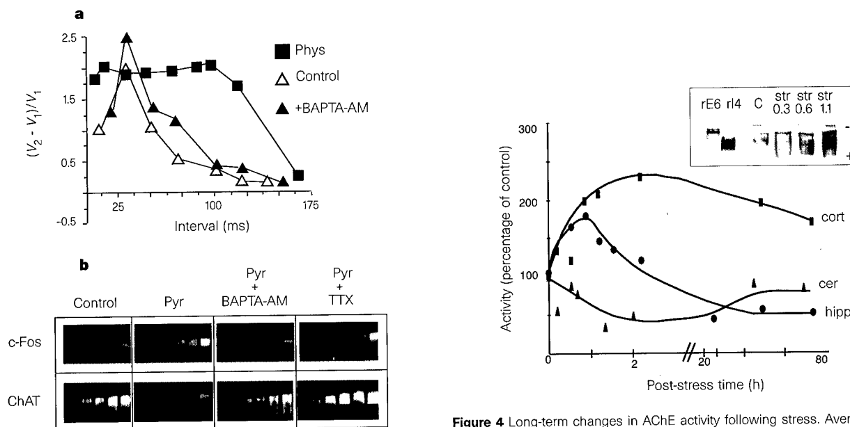
Figure 4 Long-term changes in AChE activity following stress. Average AChE activities (per cent of control) are shown in extracts of cortex (cort), cerebellum (cer), or hippocampus (hipp) from a total of 26 animals killed at the noted times after forced swimming. Specific activity (100%) in untreated controls was 3.98 \pm 1.20 , 1.95 \pm 1.34 , and 2.51 \pm 0.39 \text{ nmol substrate hydrolysed per min per mg tissue} for cortex, hippocampus and cerebellum, respectively. Inset shows that stress intensifies cortical AChE activity and diversifies its electrophoretic heterogeneity. Total proteins extracted from cortex of mice killed at the noted post-stress (str) times were electrophoresed ( 20 \mu\text{l} per lane, 1:10 \text{ wt/vol} ) in 7% non-denaturing polyacrylamide gels; catalytically active AChE was stained histochemically 14 . Recombinant human exon 6/AChE (rE6) and read-through AChE (read-through intron 4, rI4) produced in Xenopus oocytes ( 1/5 oocytes per lane) served as known correlates. C, control.
