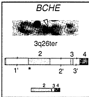
Fig. 12. BCHE , the butyrylcholinesterase gene, has been localized to 3q26ter by in situ hybridization (Gnatt et al. , 1990), and has a gene structure very similar to the homologous ACHE (Fig. 1). Although, unlike ACHE , it has a single transcript, there is considerable variation in its biological appearance due to a high frequency of mutations, some of which have no enzymatic activity, but more commonly have lower affinity for substrates and inhibitors (Whittaker, 1986; Soreq and Zakut, 1993).
