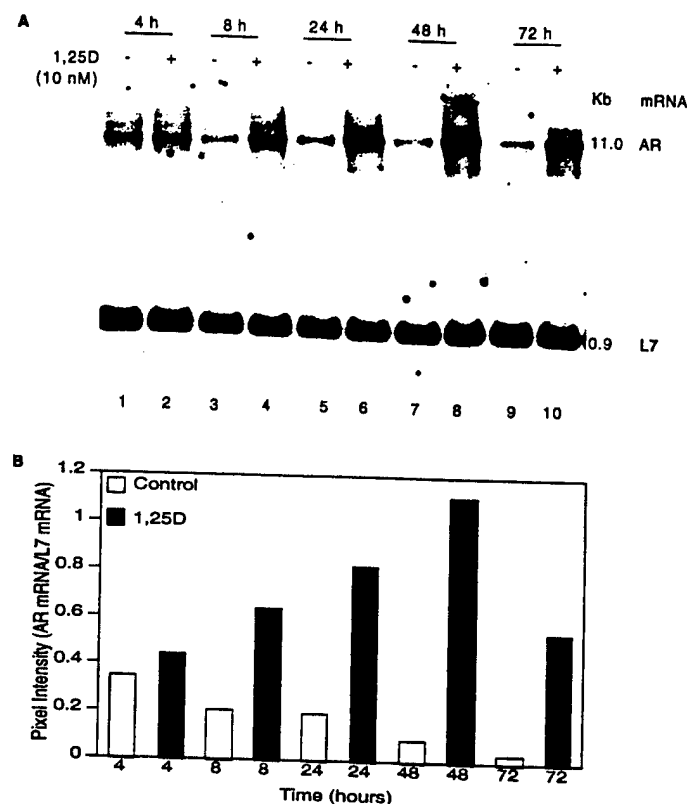
FIG. 2. Time-course of AR mRNA expression in LNCaP cells, in response to 1,25-(\text{OH})_2\text{D}_3 . A, Northern blot analysis. LNCaP cells were treated with 1,25-(\text{OH})_2\text{D}_3 , at 10 nM, for the indicated time period. Total RNA was isolated and analyzed by Northern blot using the human AR cDNA and L7 cDNA as probes. B, The pixel intensity of each AR band in panel A was scanned by computing densitometer, and the data were integrated by scanner software and indexed to the corresponding levels of L7 mRNA.
