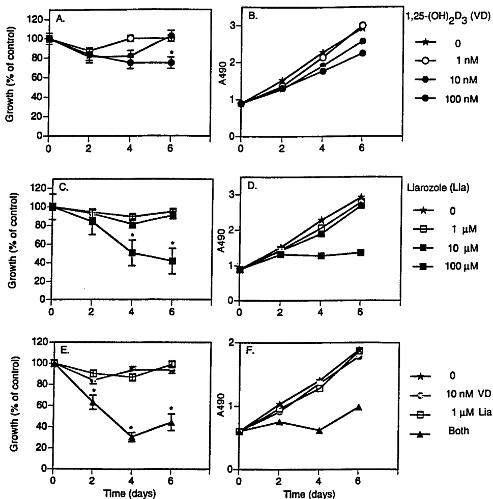
FIG. 1. Dose-response effect of 1,25-(OH) 2 D 3 , liarzozole, and the combination on DU 145 cell growth over a time course of 6 days. Cells were plated at approximately 2000 cells/well in 96-well tissue culture plates in 200 \mu l medium with the indicated concentrations of hormone. Media were changed every 2 days. Cell proliferation was estimated using the MTS assay. Data are expressed as the mean \pm SD ( n = 3 ) in the left panels. The right panels show a single representative experiment comparing treatment to vehicle and expressed in absorbance units. *, Significant changes ( P < 0.05 ) compared with the ethanol control. A and B, Treatment with 1,25-(OH) 2 D 3 . C and D, Treatment with liarzozole. E and F, Treatment with a combination of 1,25-(OH) 2 D 3 (10 nM) and liarzozole (1 \mu M).
