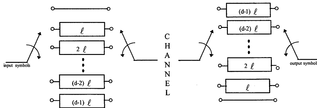
Figure 5.4 Convolutional Interleaver
