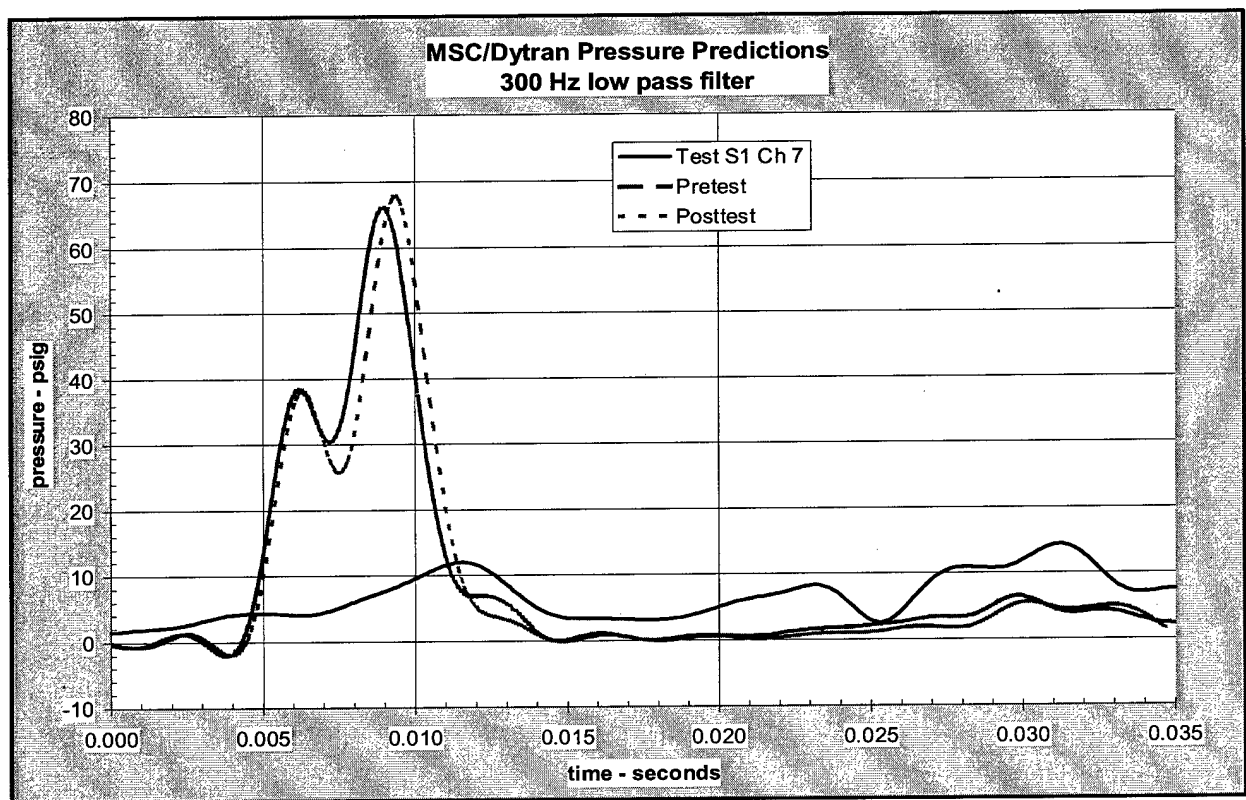
Figure 14. S1 pre & posttest pressures – FS 103-119 BL 0 – DRI/KRASH vs test
