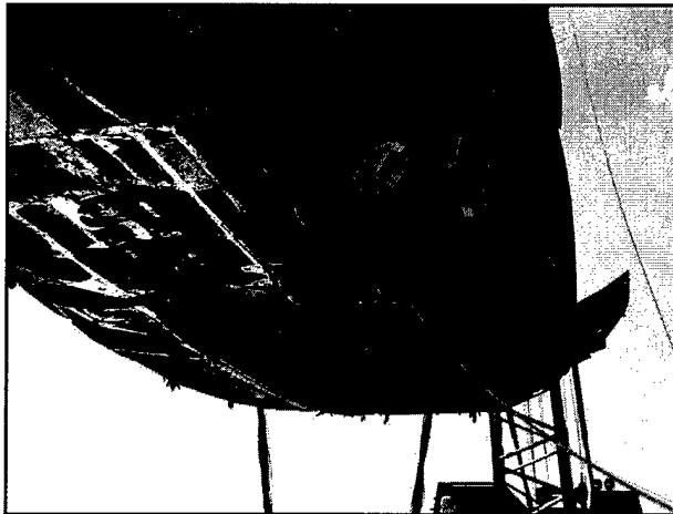
Figure 7. S1 test underside damage
