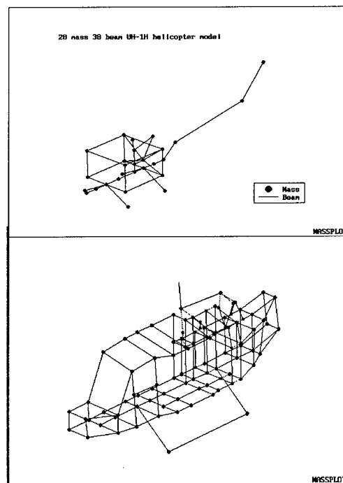
Figure 3. Original and final DRI/KRASH Models
