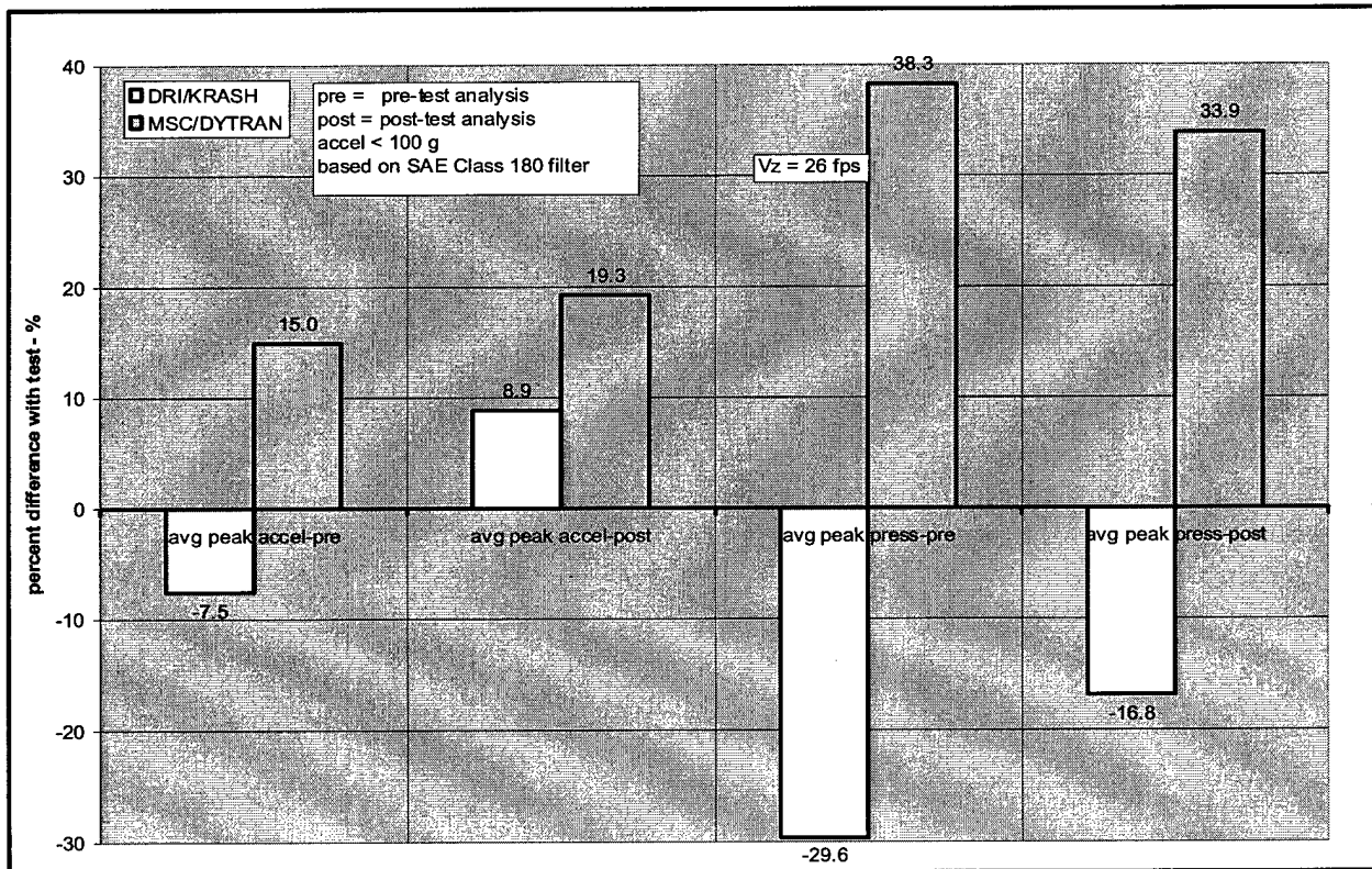
Figure 17. Analysis vs test data - overall
