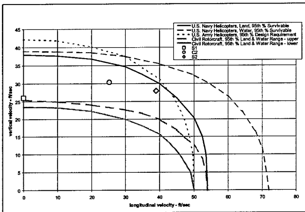
Figure 4. Impact envelope and test conditions
