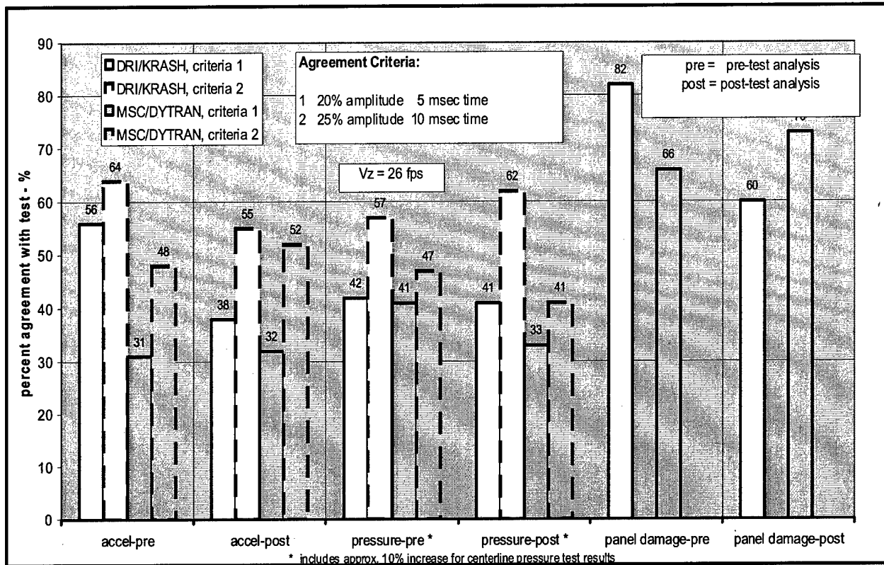
Figure 16. Analysis vs test data - discrete
