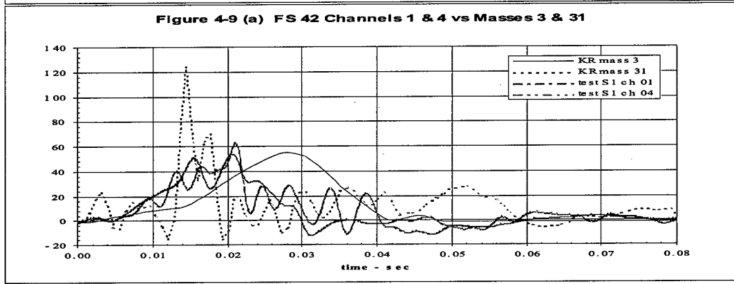
Figure 8. S1 pre & posttest accelerations - FS 42 BL 14 - DRU/KRASH vs test
