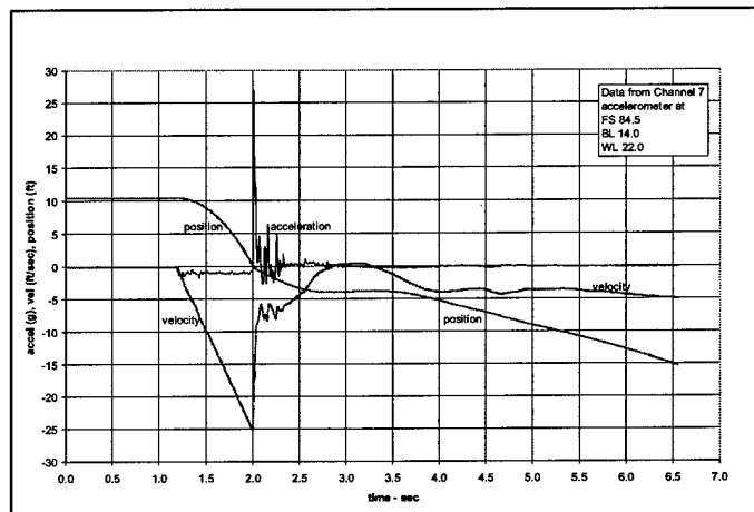
Figure 6. S1 test vertical acceleration, integrated velocity and position
