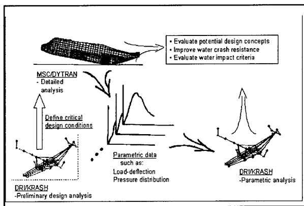
Figure 1. Combined FEM/hybrid approach.
