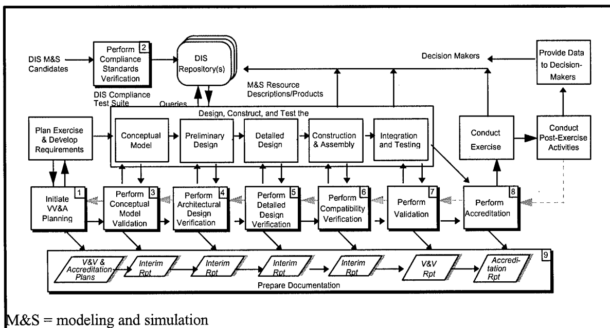
Figure 7. DIS Nine-Step VV&A Process Model
