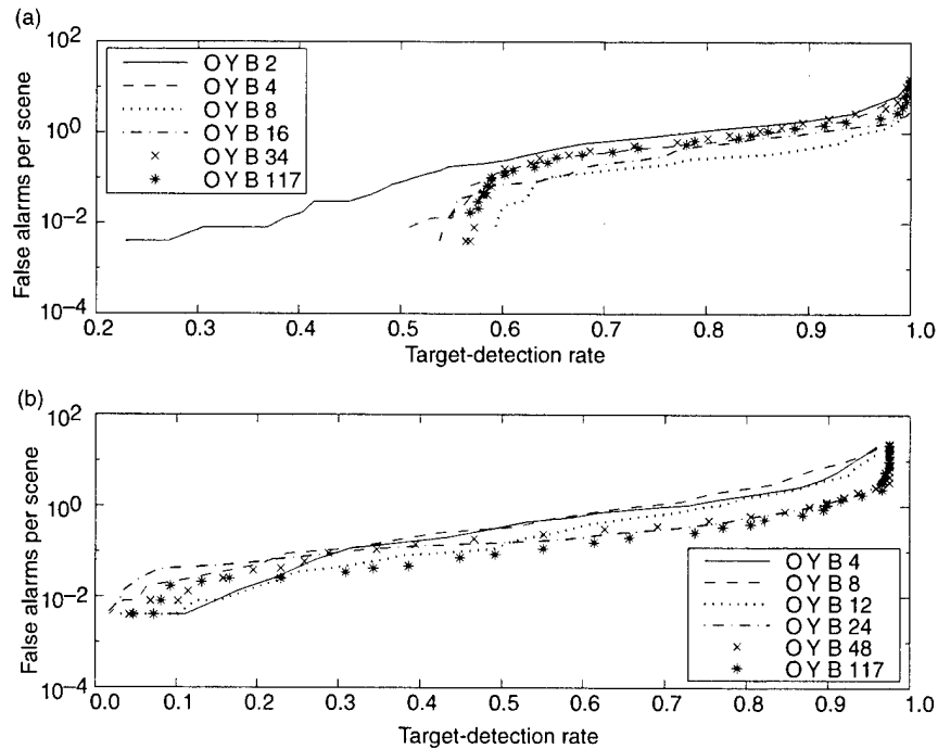
Figure 2. (a) M60 and (b) tnk baseline (B) performance.
