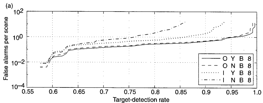
Figure 3. Additional (a) M60 and (b) tnk baseline (B) performance curves.
