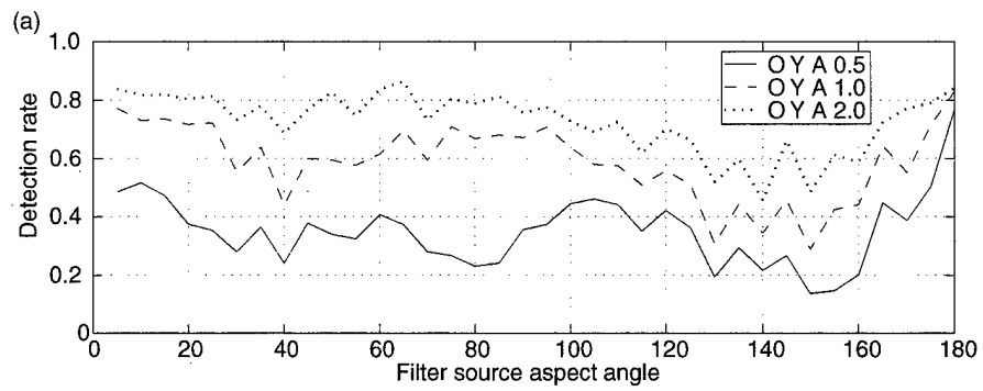
Figure 8. (a) M60 and (b) tnk filter performance as function of filter source aspect angle (A).
