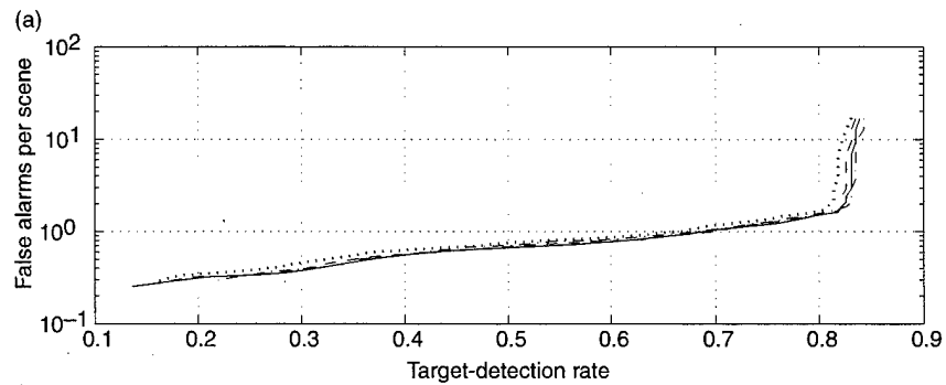
Figure 9. (a) M60 and (b) tnk filter performance for all scales and all aspect angle.
