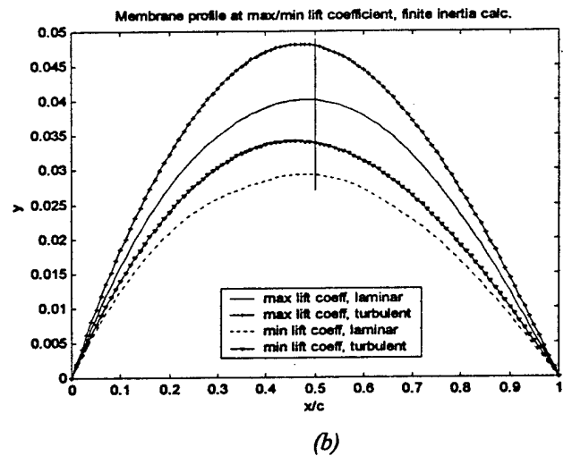
Figure 10: The membrane profiles at maximum and minimum values of C_L for laminar and turbulent flows, \alpha = 4^\circ , Re = 10^6 , \Pi_1 = 7.9 , \tilde{\Pi}_1 = 0.99 , (a) Massless computation, (b) Finite inertia computation, \tilde{\rho}_m = 500 .
