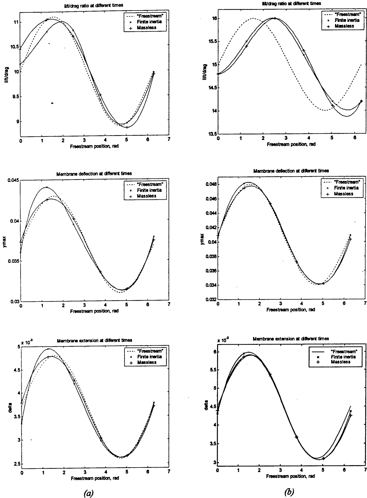
Figure 6: Lift/Drag ratio, membrane maximum deflection and extension during one freestream oscillation, \Pi_1=7.9 , \tilde{\Pi}_1=0.99 , \alpha=4^\circ (a) Laminar case, Re=4000 (b) Turbulent case, Re=10^6 .
