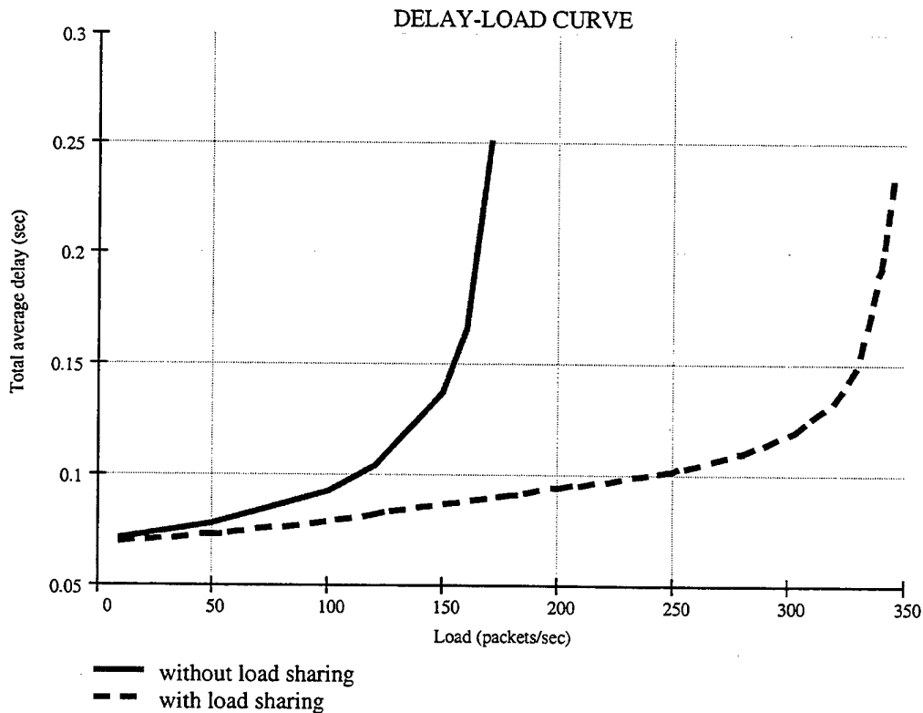
Figure 35. Delay-load curve
